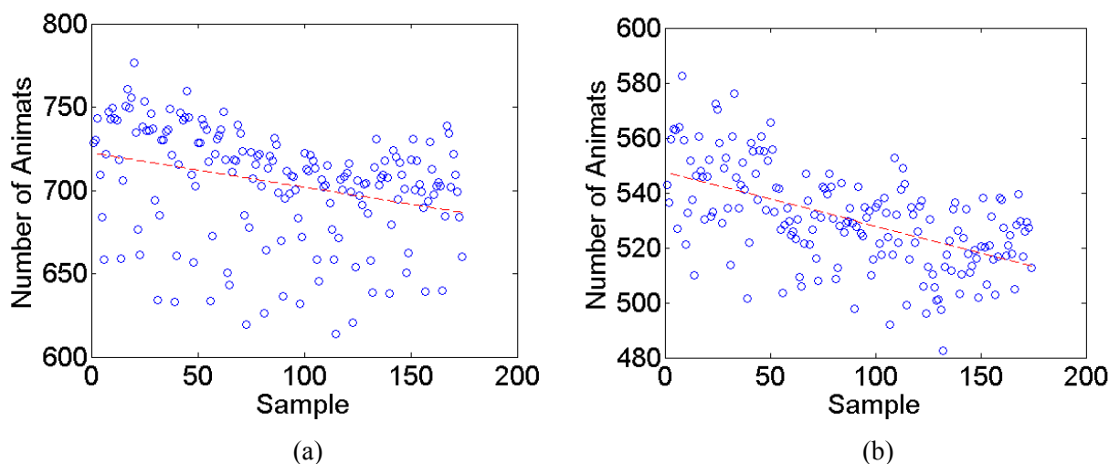
Figure 23. Cuvier's beaked whales: Behavioral exposure estimates for (a) Survey sites A and (b) B. Exposure estimates are for 24 h sliding windows (samples), which advance in 4 h increments during 30 day simulations. Circle markers indicate exposure estimates during each 24 h sample period, dashed red line is a least-squares fit.
