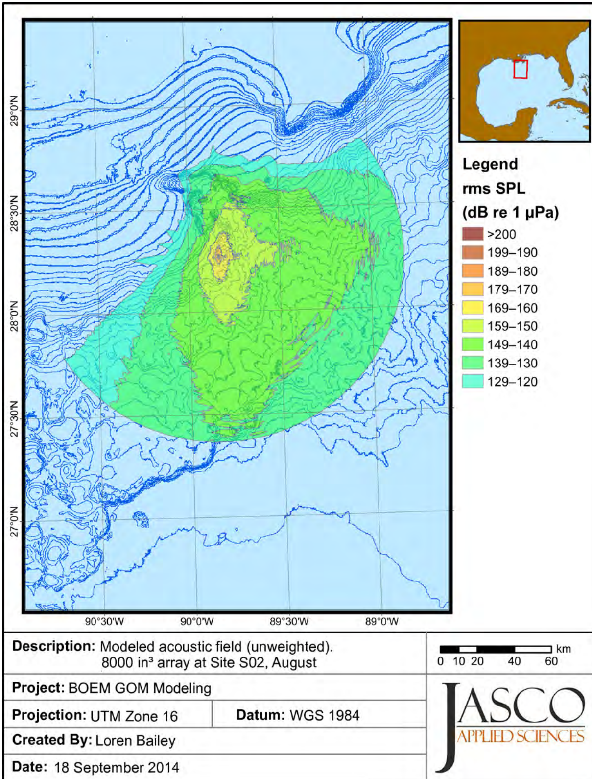
Figure 127. Broadband (10–5000 Hz) maximum-over-depth sound pressure levels for 8000 in 3 airgun array, in August at the Survey site A, S02 modeling province. Blue contours indicate water depth in meters.
