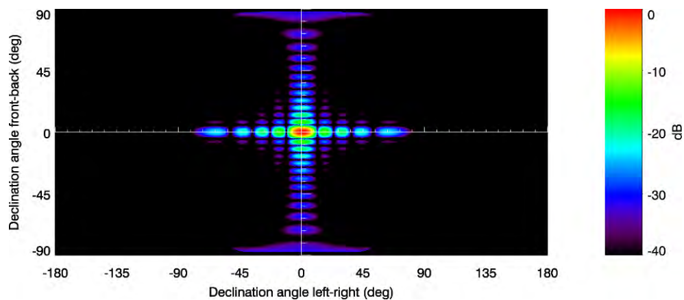
Figure 4. Calculated beam pattern for a rectangular transducer with a 4^\circ \times 10^\circ beamwidth. The beam power function is shown relative to the on-axis level using the Robinson projection.
