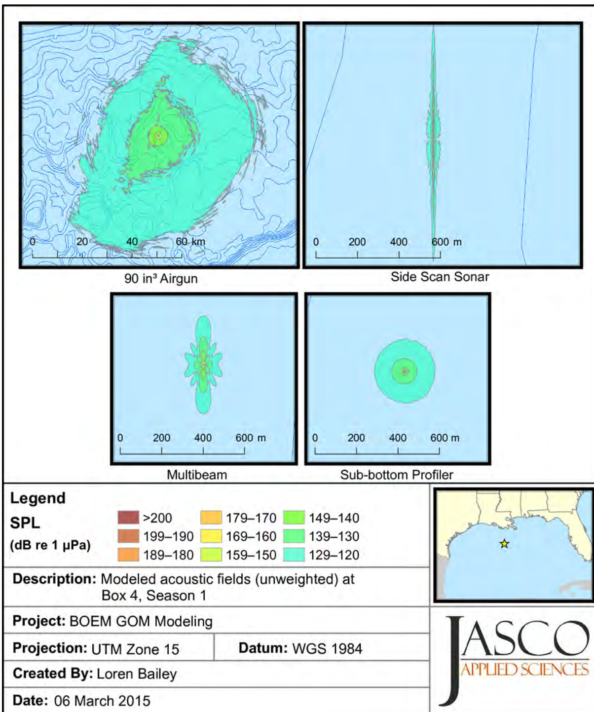
Figure E-5. Box 4 geotechnical sources: Maximum-over-depth sound pressure levels during Season 1 (February).
