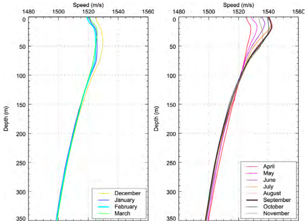
Figure 29. The Shelf zone ( 28.5^{\circ} N, 90^{\circ} W): Mean monthly sound speed profiles, separated into Seasons 1 (left) and 2 (right). Bolded profiles indicate average sound speed profile used for the season. Derived from data obtained from GDEM V 3.0 (Teague et al. 1990, Carnes 2009).
