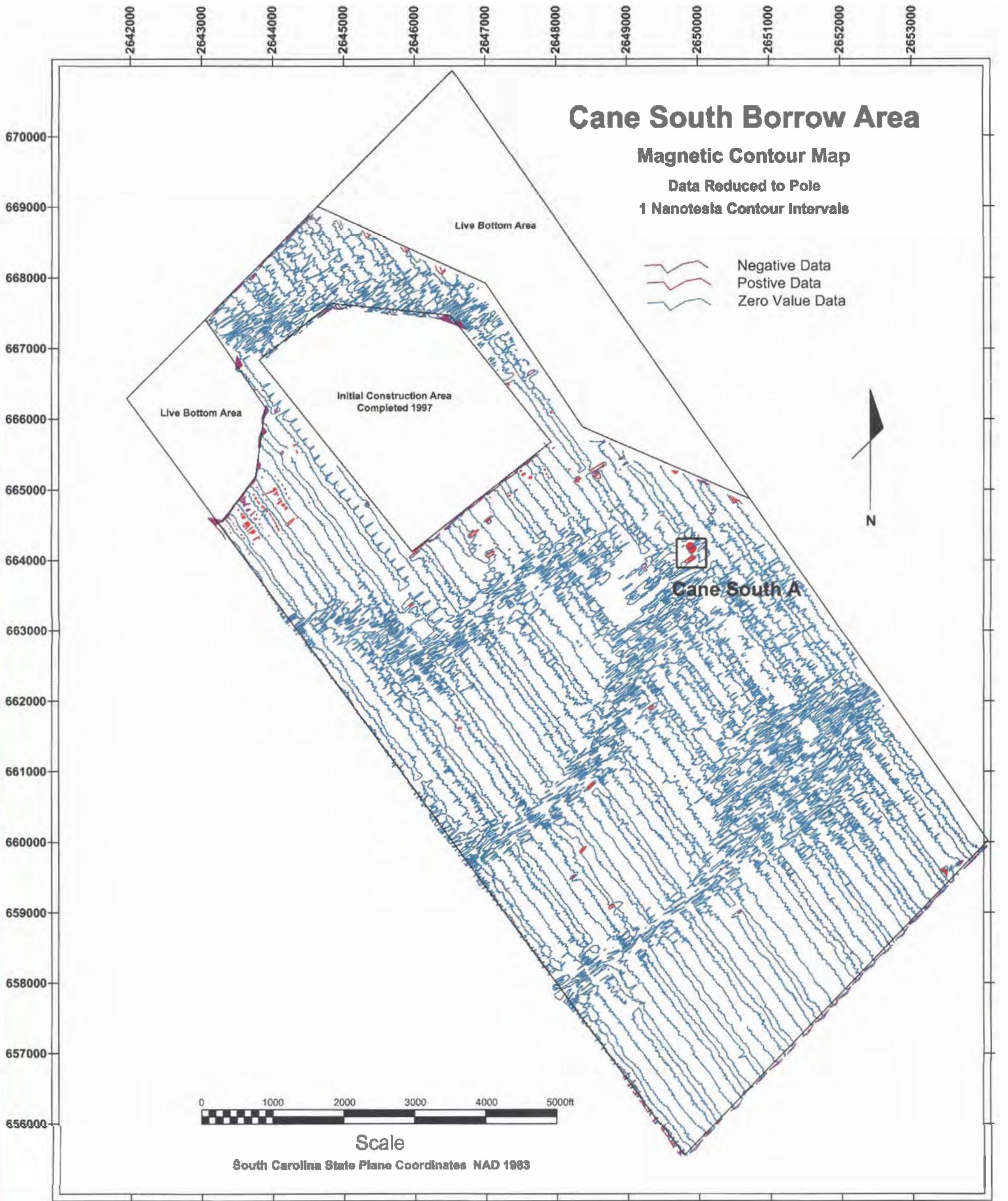
Figure 8. Cane South Borrow Area Magnetic Contour and Target Location Map.
