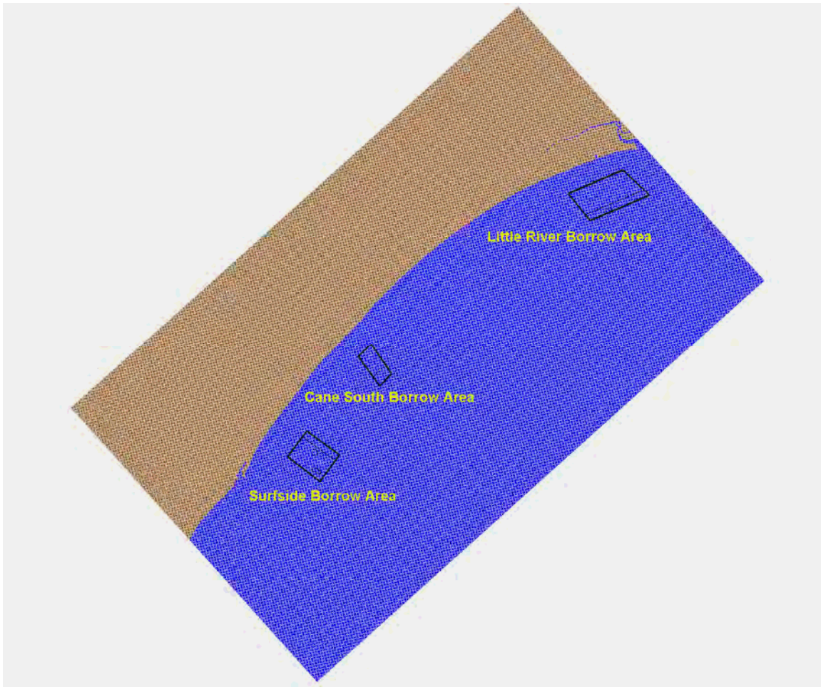
Figure 3: STWAVE Model grid overlaid with Myrtle Beach borrow areas.
