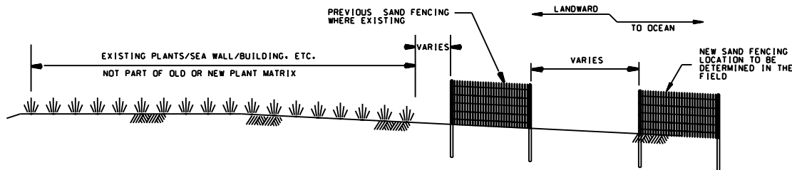
FENCING AND BEACH GRASS NO SCALE
