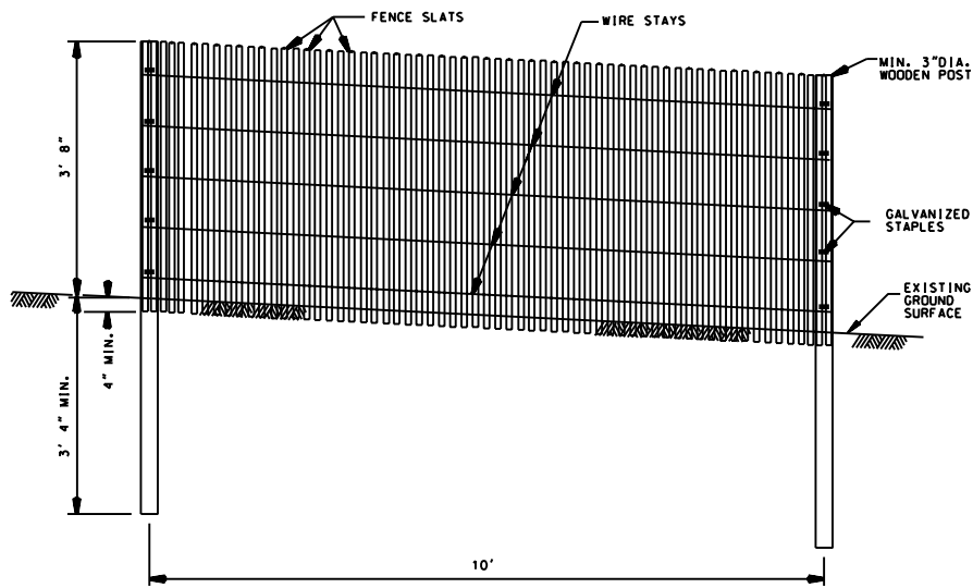
ELEVATION -- FENCE PANEL NO SCALE
