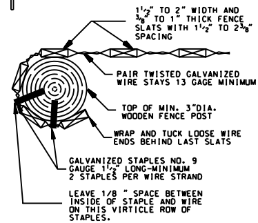
DETAIL A FENCE POST (TYP.) NO SCALE
