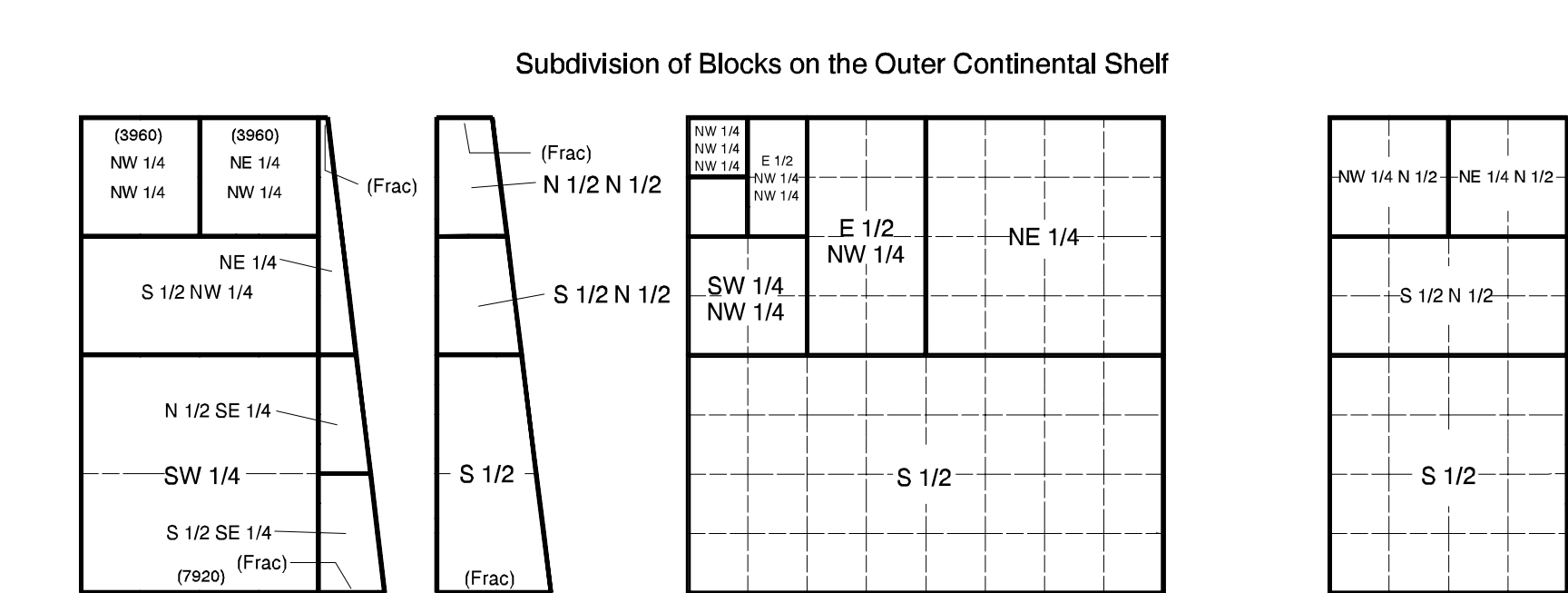
Typical method of subdivision of the regular blocks and irregular blocks, each subdivision being an aliquot part of the total, based on midpoint subdivision throughout, with fractional areas and measurements along the east boundary.
