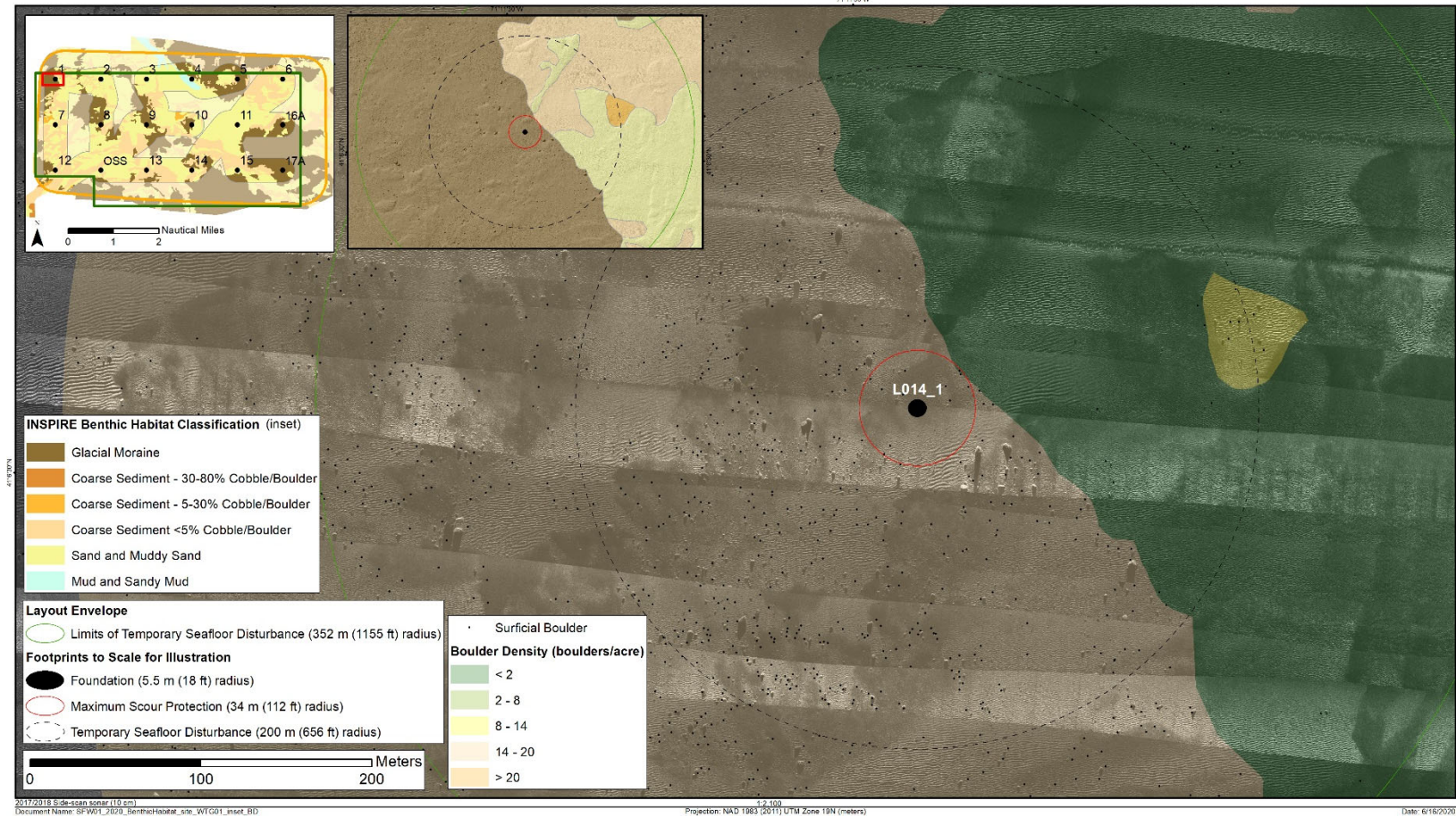
Figure 4-4. WTG-1 footprint with habitat classification, boulder density, and high-resolution side-scan sonar
