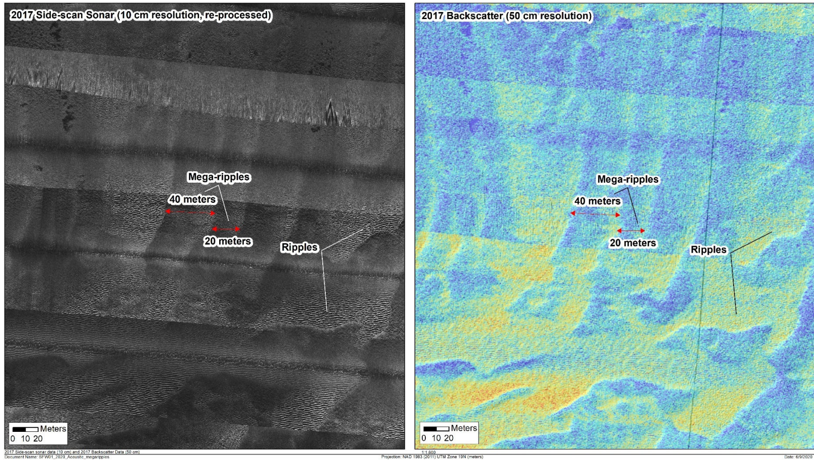
Figure 2-11. Mega-ripples visible in SSS (left) and backscatter data (right)
