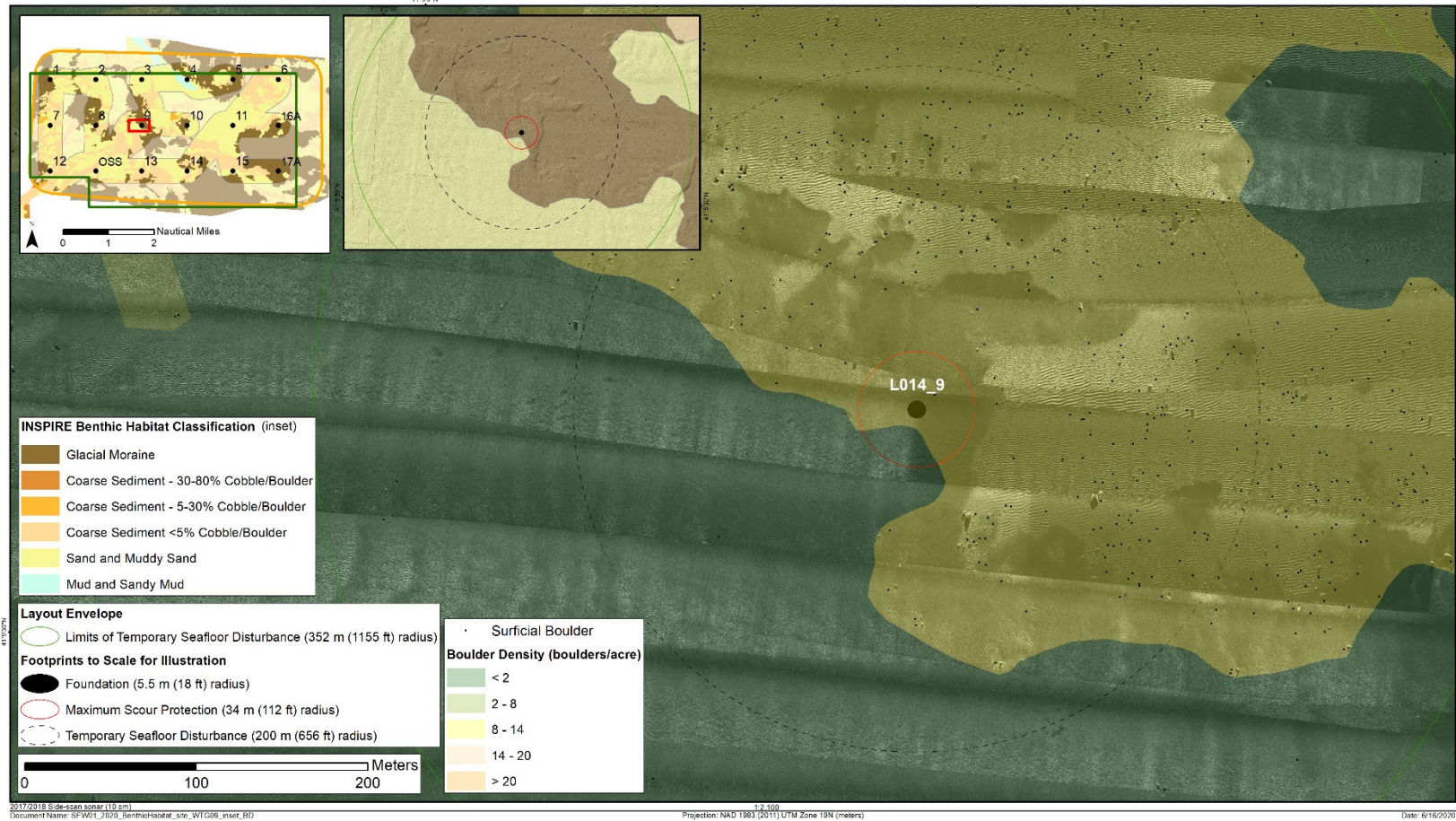
Figure 4-5. WTG-9 footprint with habitat classification, boulder density, and high-resolution side-scan sonar
