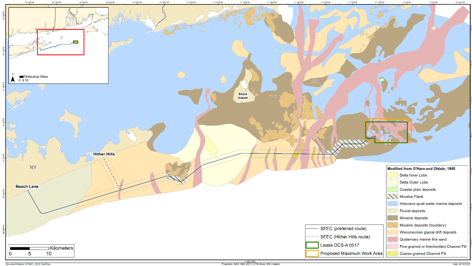
Figure 3-8. Distribution of surficial geological deposits (after Fugro 2019 modification to O'Hara and Oldale 1980) in Rhode Island Sound
