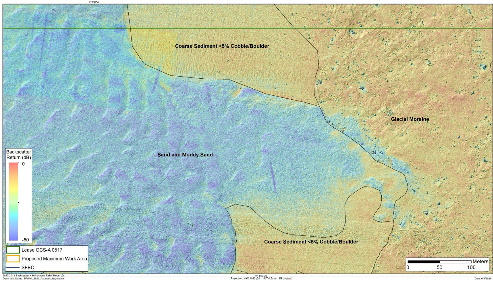
Figure 2-15. Example of using backscatter data to delineate large scale facies
