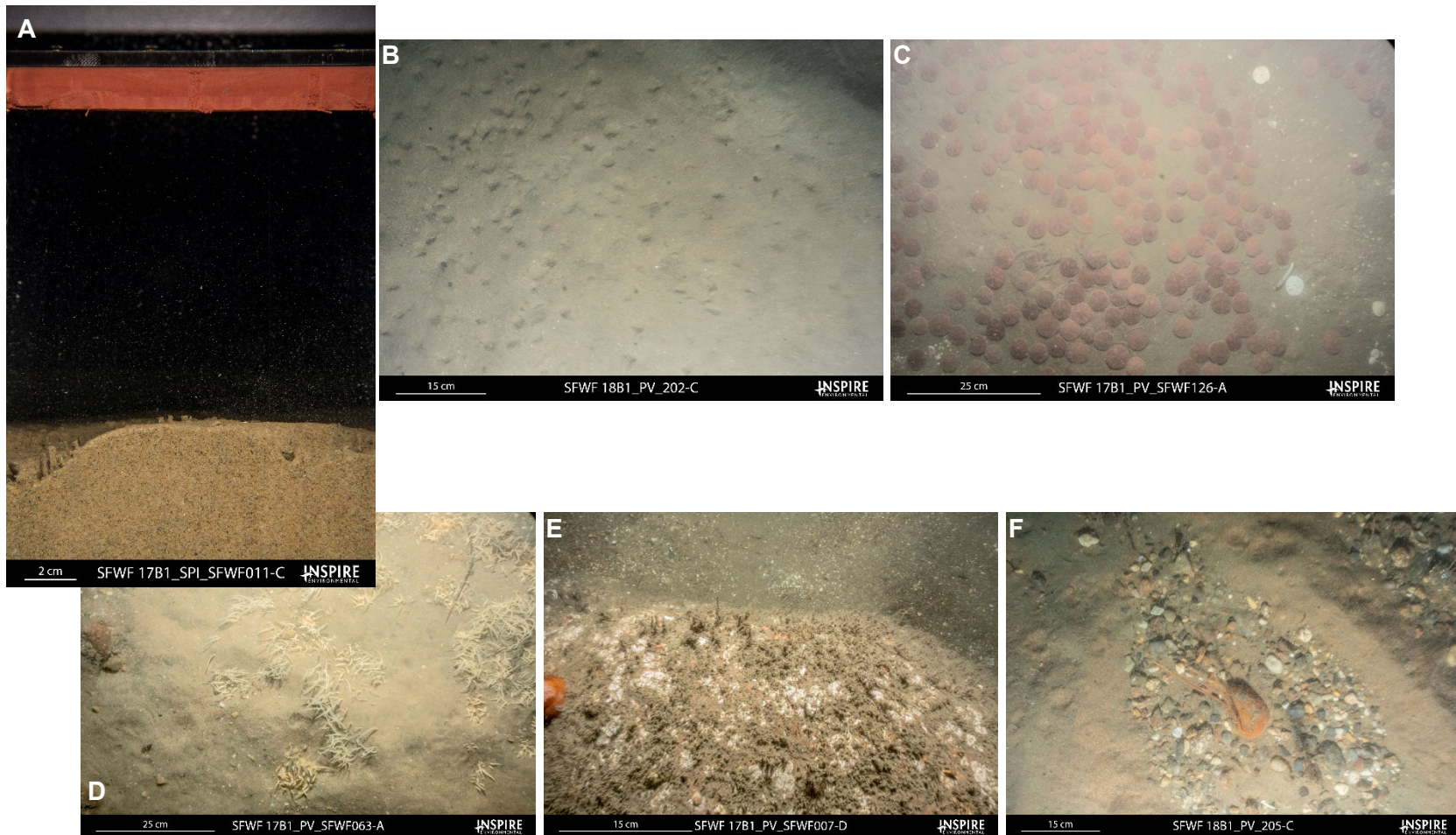
Figure 2-14. Representative SPI and PV images depicting soft sediment infaunal communities: (A) infaunal tubes, (B) extensive burrowing activity, and (C) sand dollars; and attached epifaunal communities: (D) Polymastia sp. sponge, (E) anemones, grazed barnacles, and (F) attached hydroids
