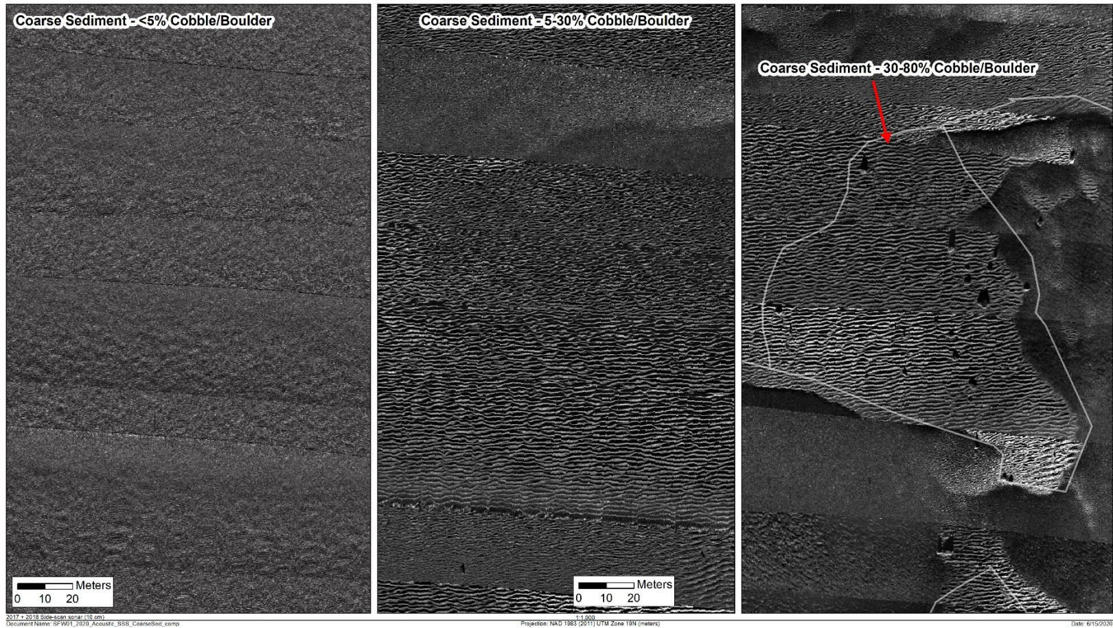
Figure 3-4. Example SSS data depicting Coarse Sediment habitats with <5%, 5-30%, and 30-80% cover of cobbles and boulders
