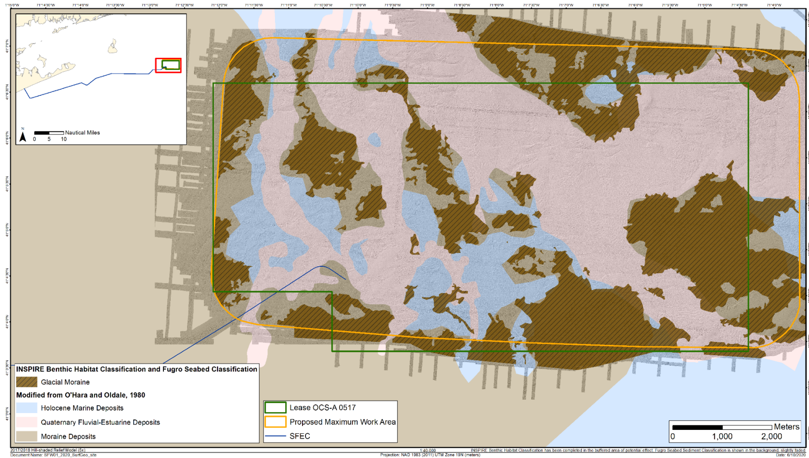
Figure 3-7. Distribution of surficial geological deposits (Fugro 2019 modification to O’Hara and Oldale 1980) and benthic habitat types within the SFWF
