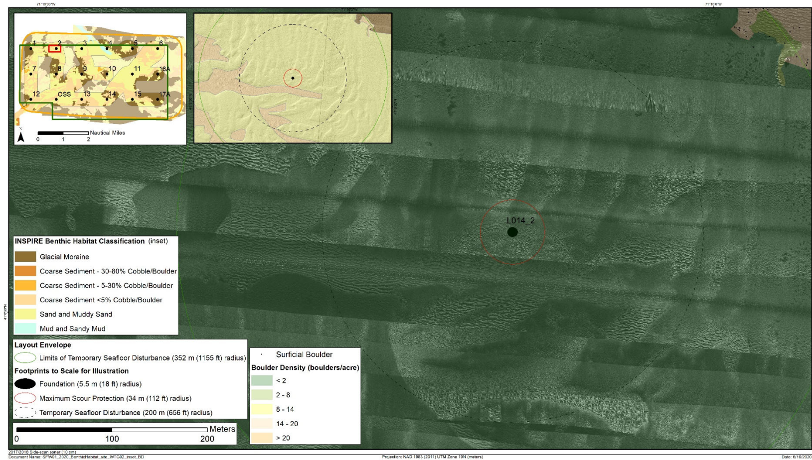
Figure 4-3. WTG-2 footprint with habitat classification, boulder density, and high-resolution side-scan sonar
