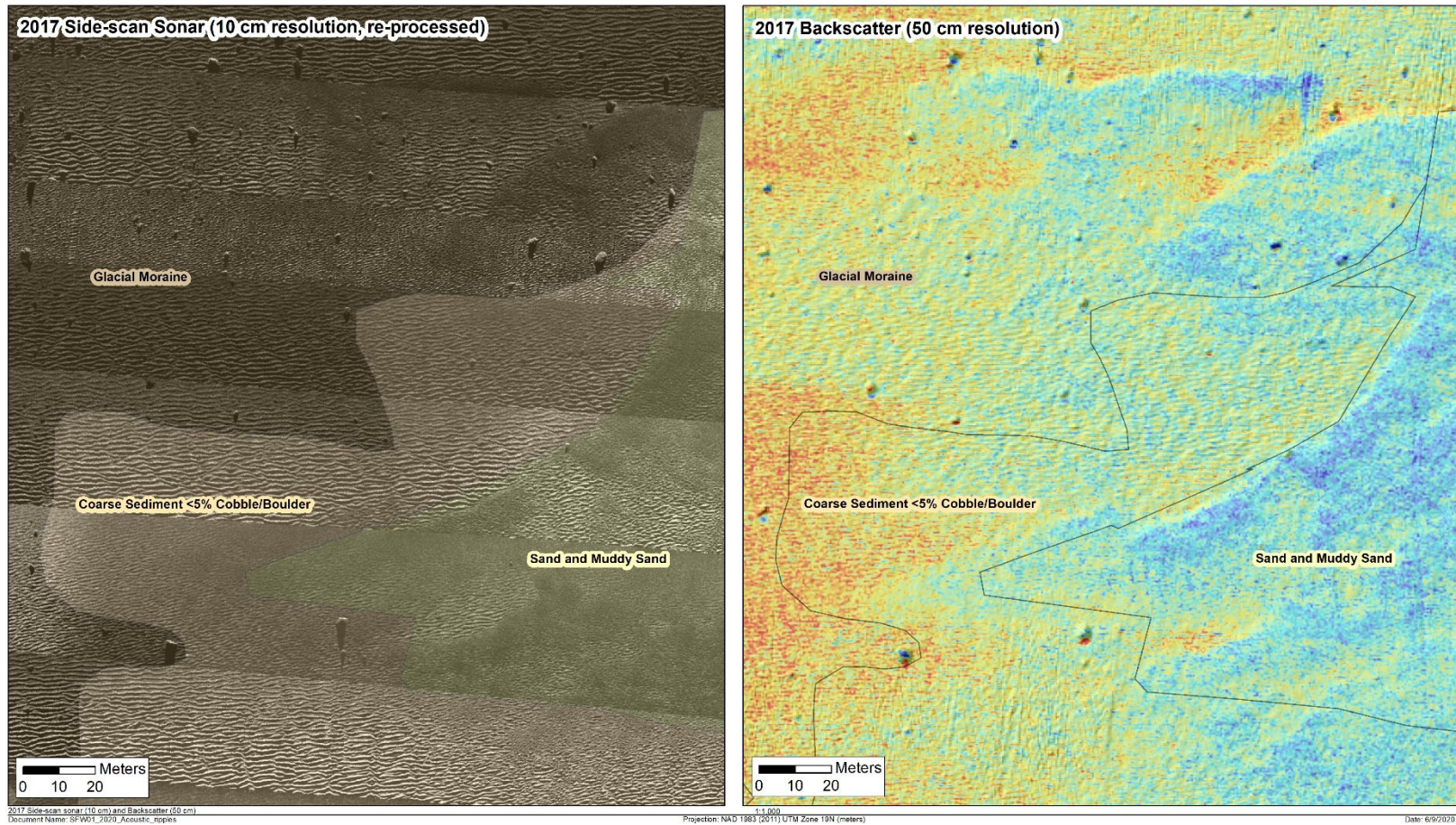
Figure 2-12. Ripples visible in SSS (left) and backscatter data (right)
