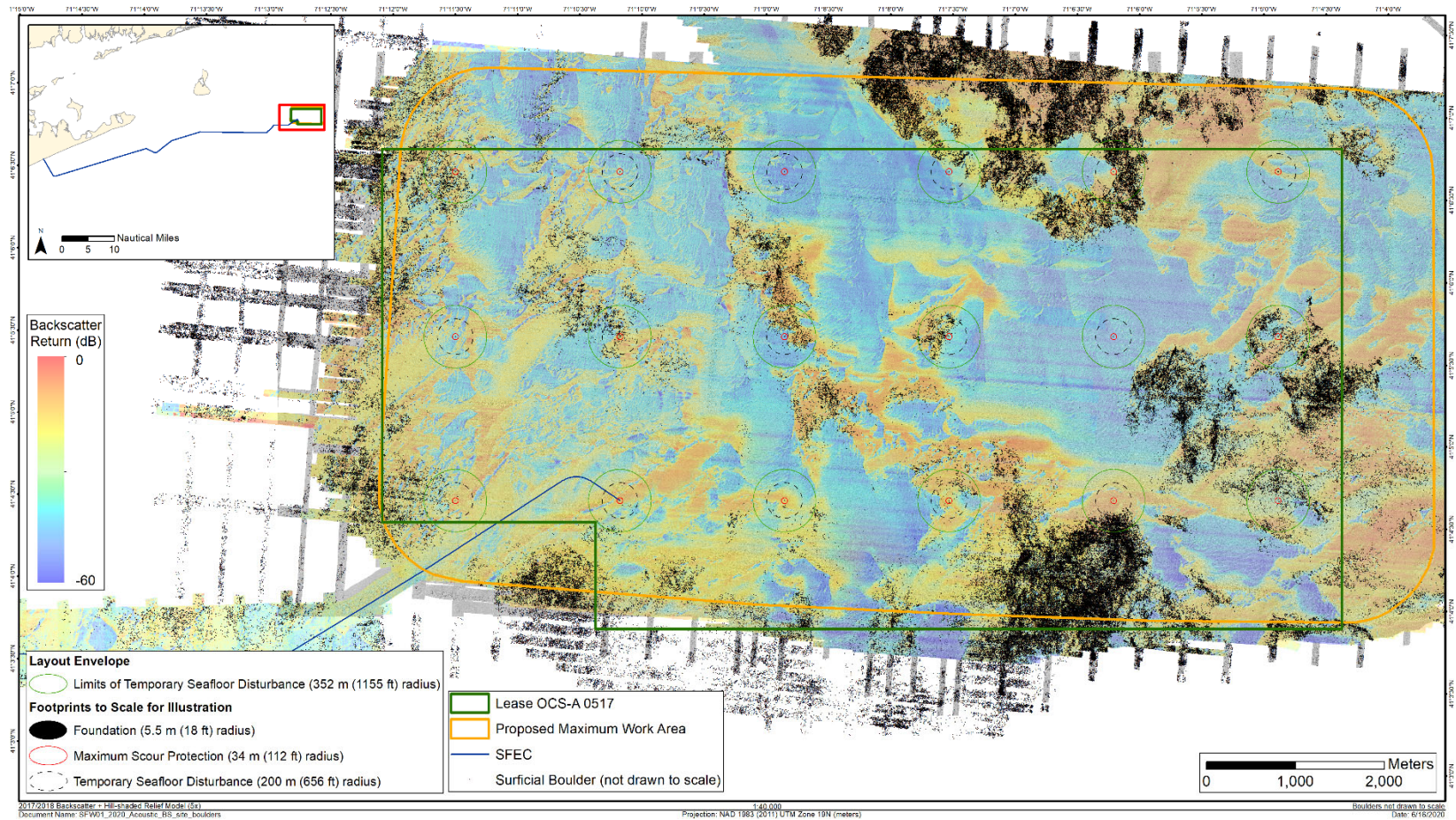
Figure 2-9. Boulder picks on backscatter data at the SFW Lease Area
