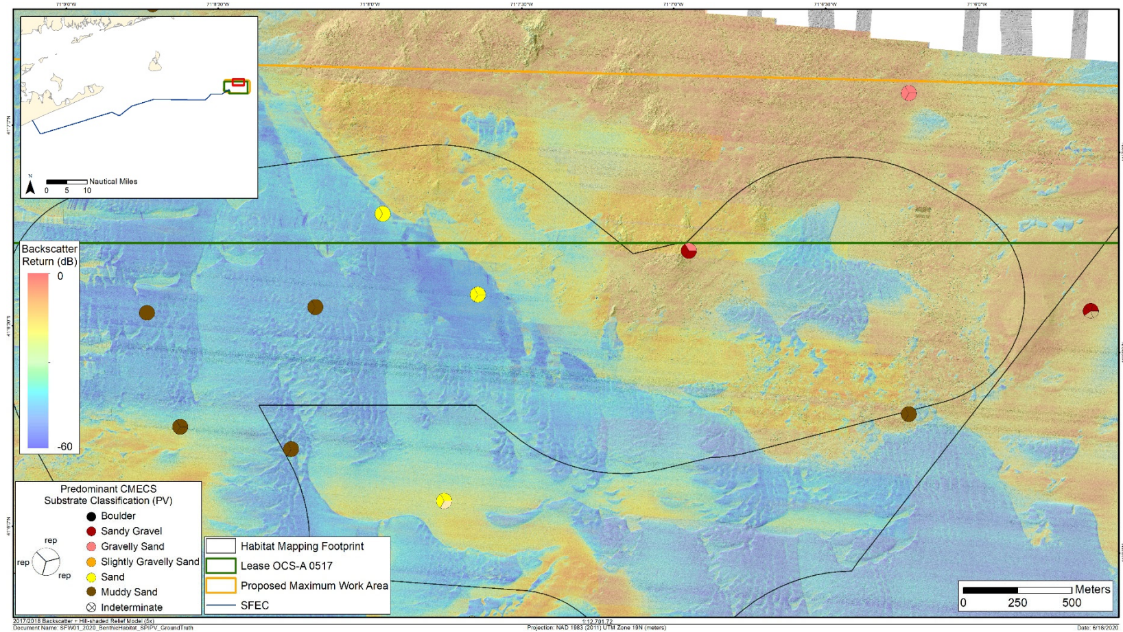
Figure 2-19. Ground-truth PV data for CMECS Substrate Group/Subgroup overlaid on MBES backscatter data
