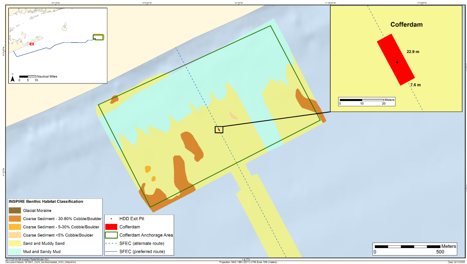
Figure 3-26. Benthic habitats mapped at the Hither Hills sea-to-shore transition and the cofferdam footprints for which maximum areas of potential impact were calculated
