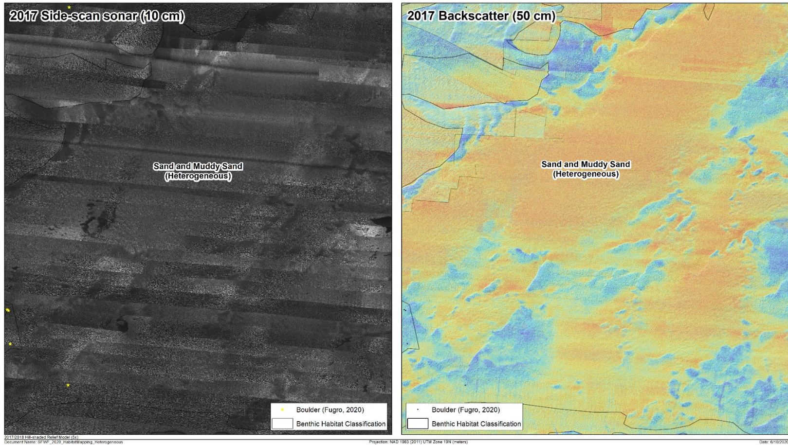
Figure 2-21. Examples of heterogeneity visible in side-scan sonar (left) and backscatter data (right)
