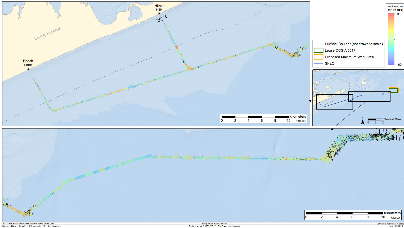
Figure 2-10. Boulder picks on backscatter data along the SFEC
