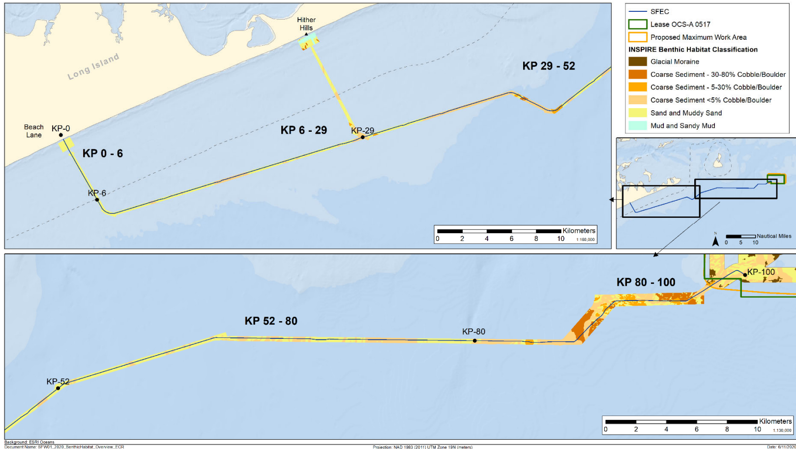
Figure 3-23. Benthic habitats mapped along the SFEC and SFEC segments for which maximum areas of potential impact were calculated; KPs mark kilometers between the landfall and the OSS. Boulder relocation is assumed along the KP29 - KP52 and KP80 - KP100 segments.
