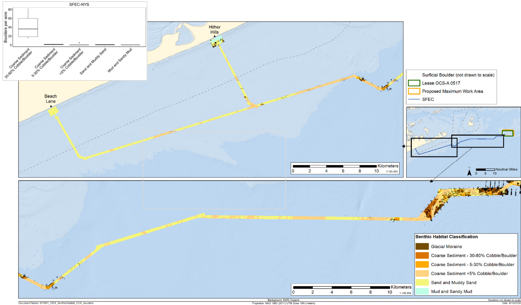
Figure 3-15. Benthic habitat types mapped along the SFEC, boulder picks and box plots of boulder density across habitat types
