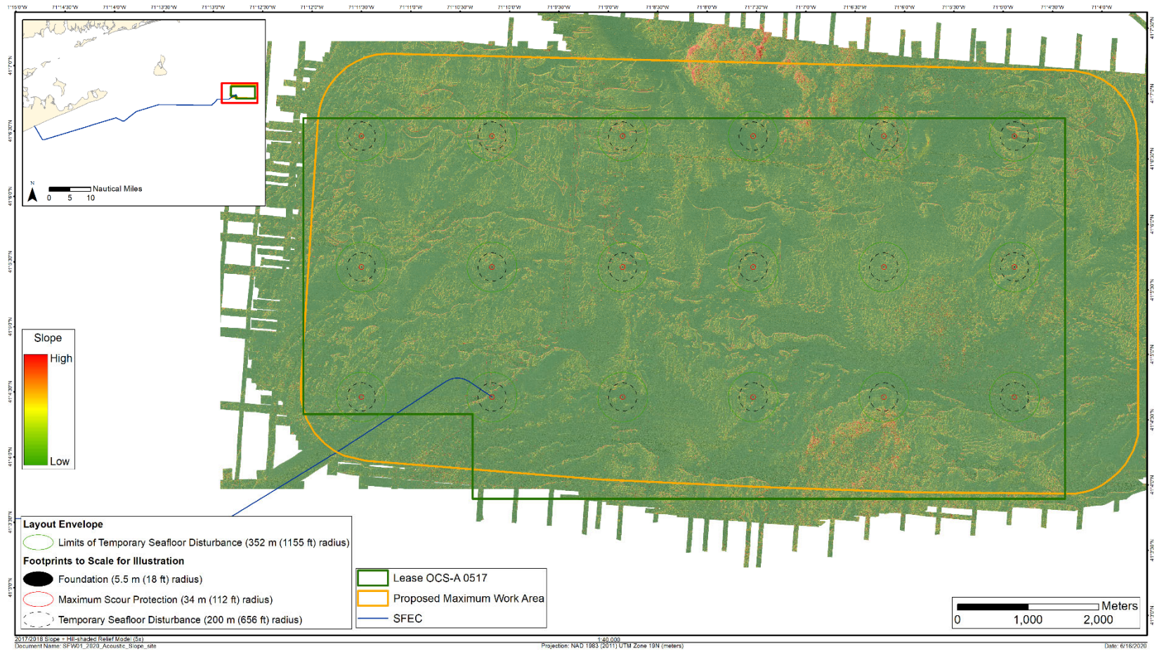
Figure 2-4. Model of seafloor slope at the SFW Lease Area
