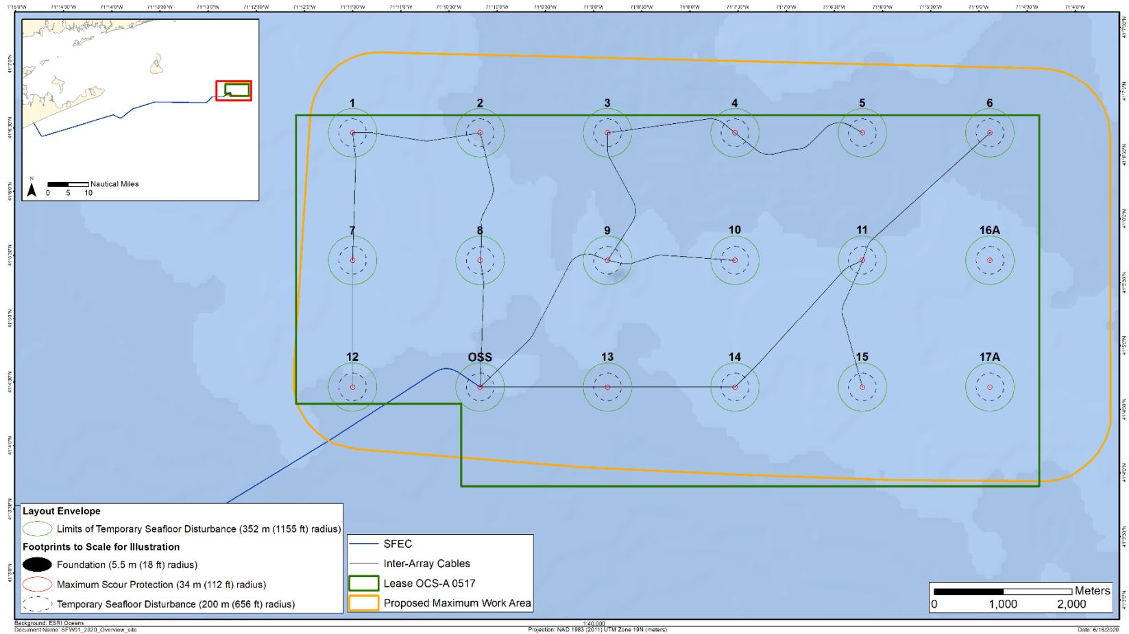
Figure 1-2. South Fork Wind Lease Area proposed project design on 1 x 1 nm grid and planned Inter-array Cables
