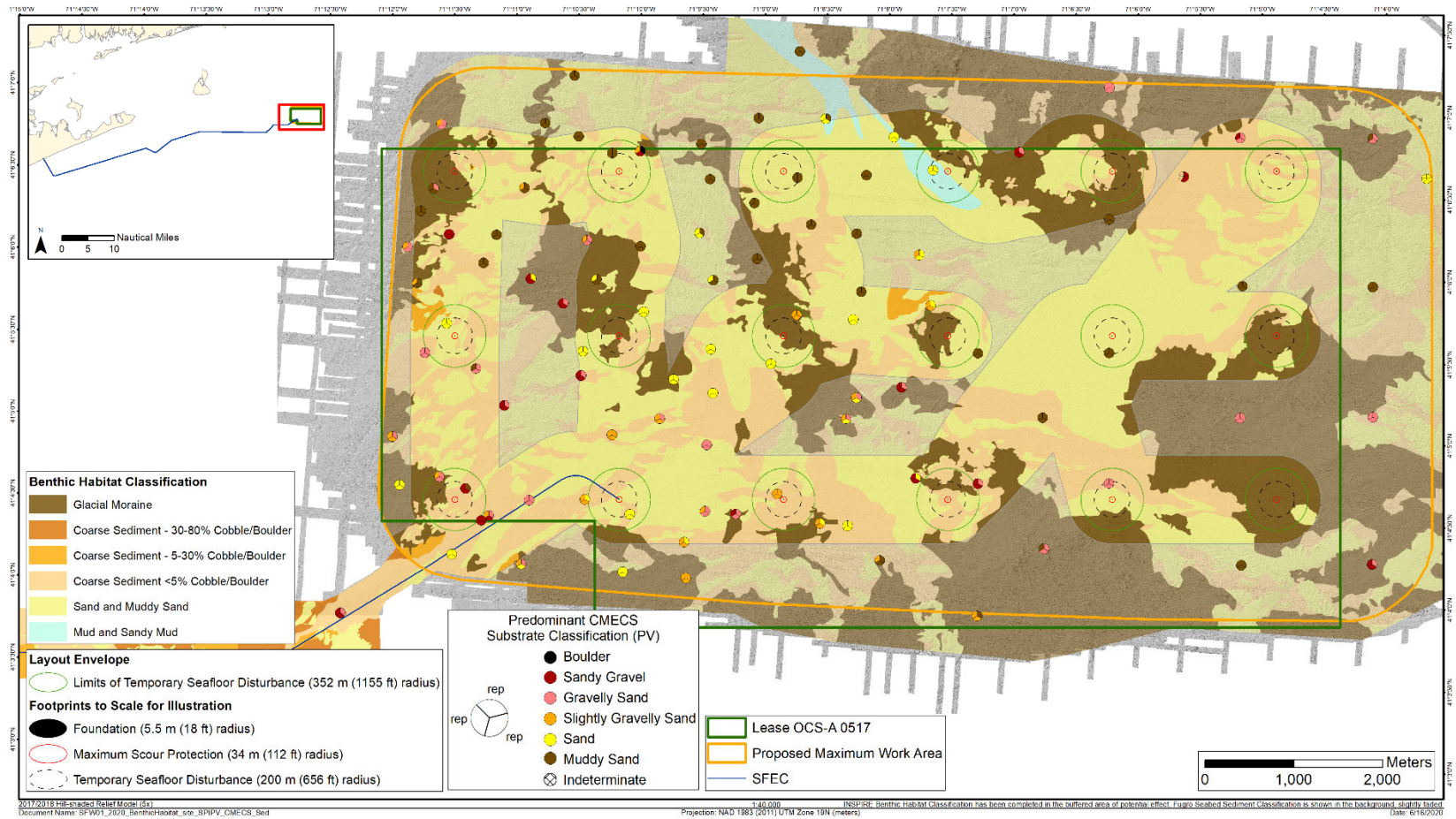
Figure 3-12. Benthic habitat types mapped within the SFWF and ground-truth CMECS Substrate Group/Subgroup
