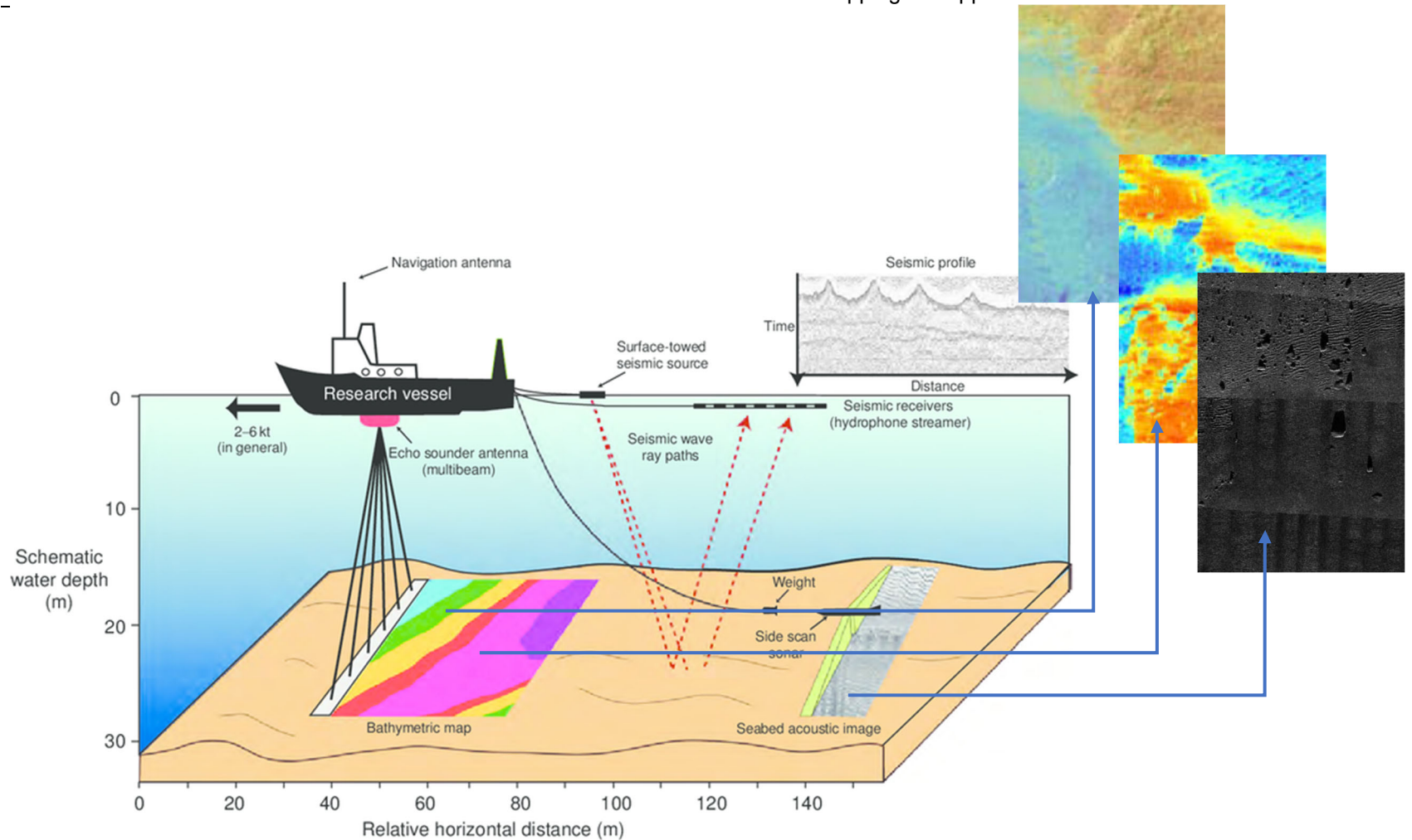
Figure 2-1. Schematic depicting a standard acoustic survey vessel set-up and data collection (after Garel et al. 2009)
