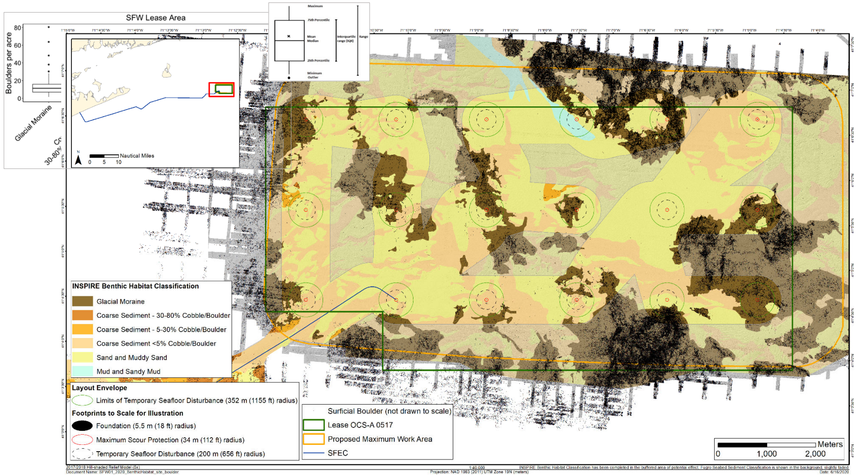
Figure 3-10. Benthic habitat types mapped within the SFWF, boulder picks and a box plot of boulder density across habitat types
