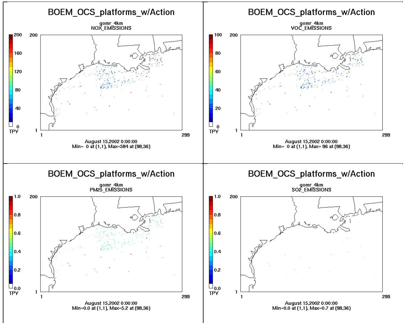
Figure D-14. Spatial Distribution of (clockwise starting from top left) NO x , VOC, SO 2 , and PM 2.5 Emissions (tons per year) from New OCS Oil and Gas Production Platforms under the Proposed Action.
