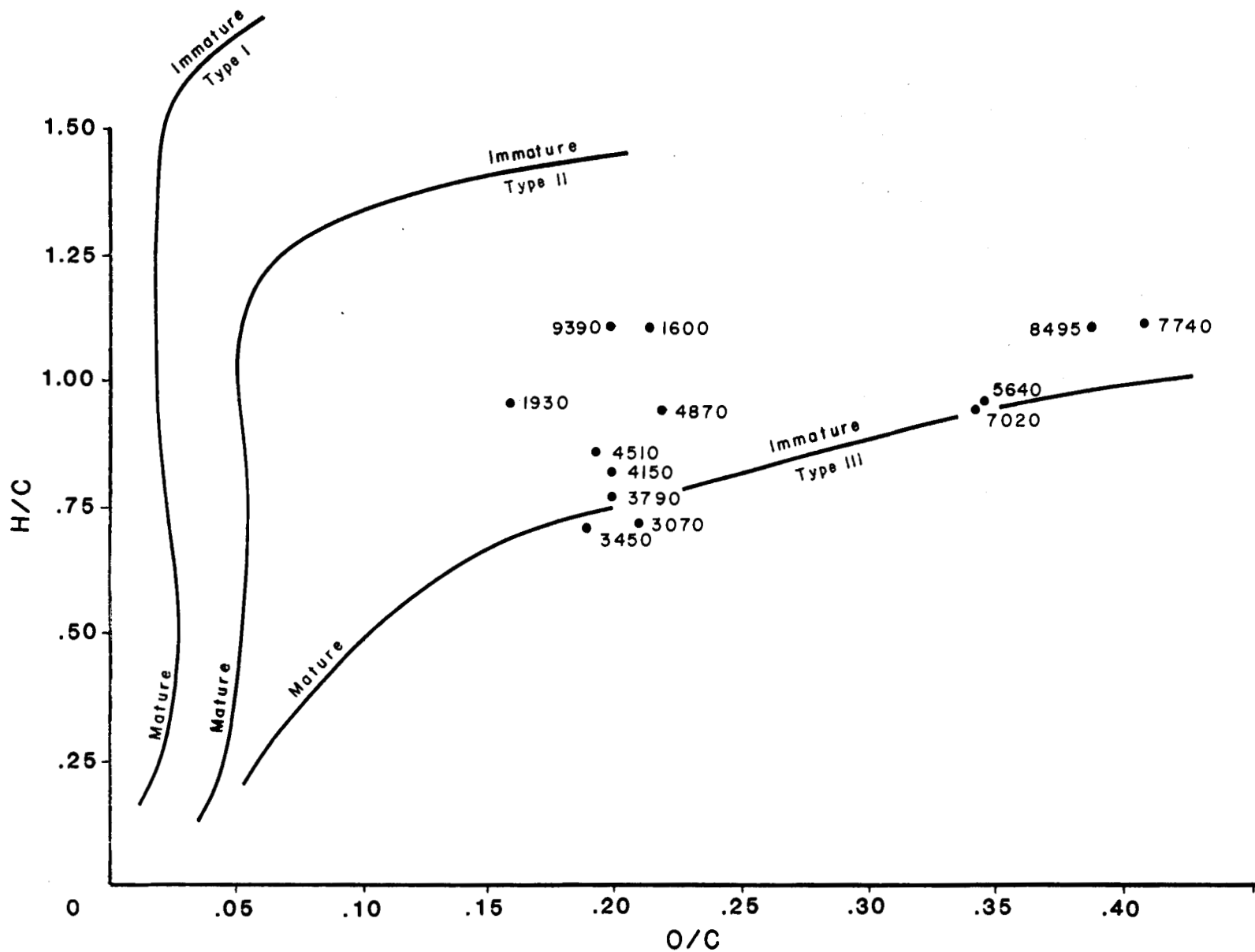
Figure 27. Van Krevelen diagram (atomic ratios) for kerogens. Depths given in feet. (Elemental analyses performed by Amoco Production Co.)
