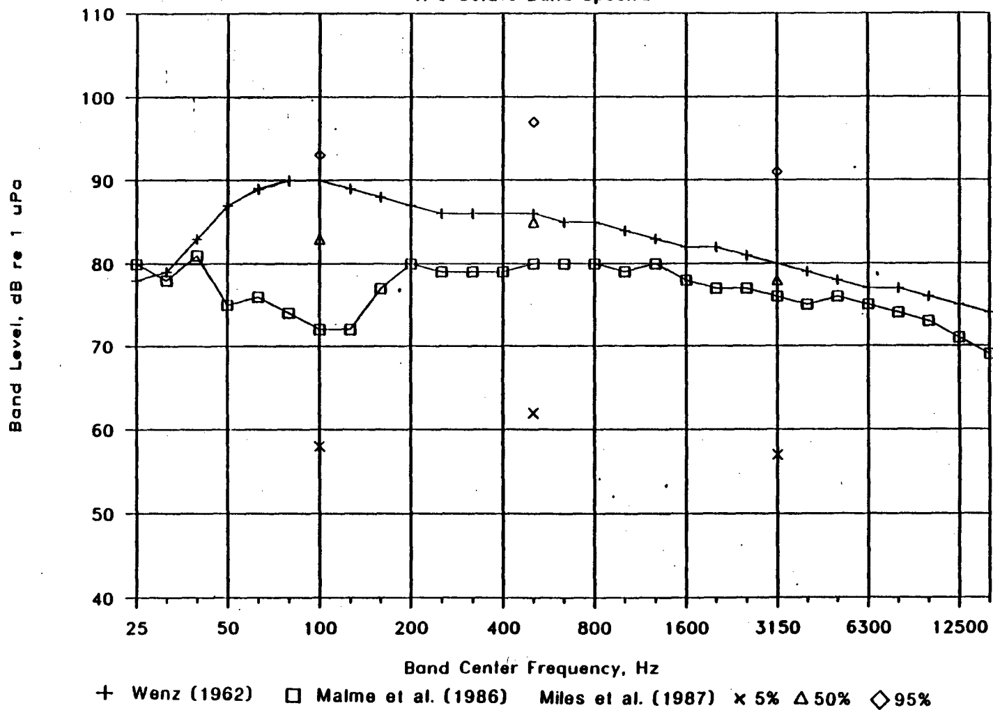
Figure 2. Shallow water ambient noise.
