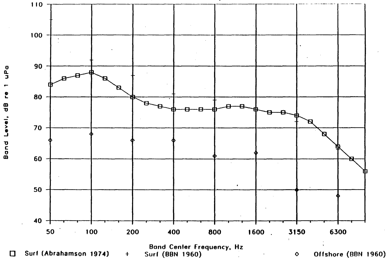
Figure 1. Airborne ambient noise near beach areas.
