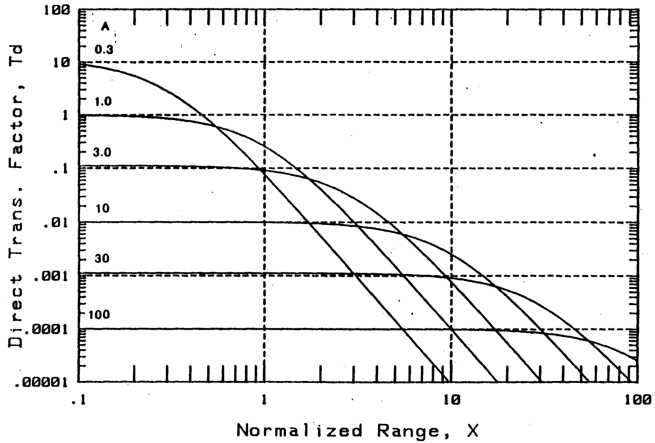
Figure 12. Factors for air - shallow water sound transmission A. Direct path transmission factor B. Depth-averaged path transmission factor.
