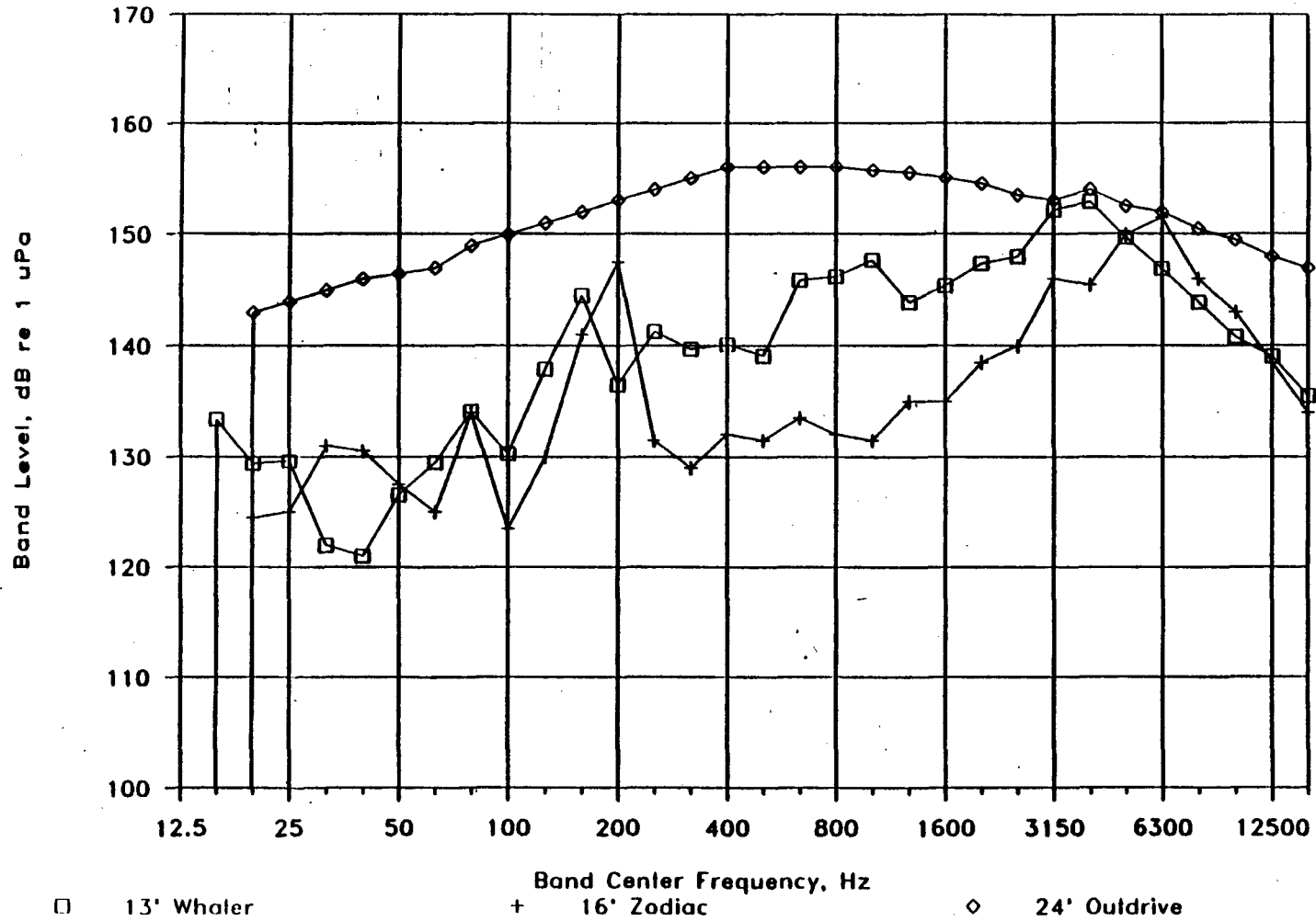
Figure 5. A. Small craft source level spectra B. Medium vessel source level spectra.
