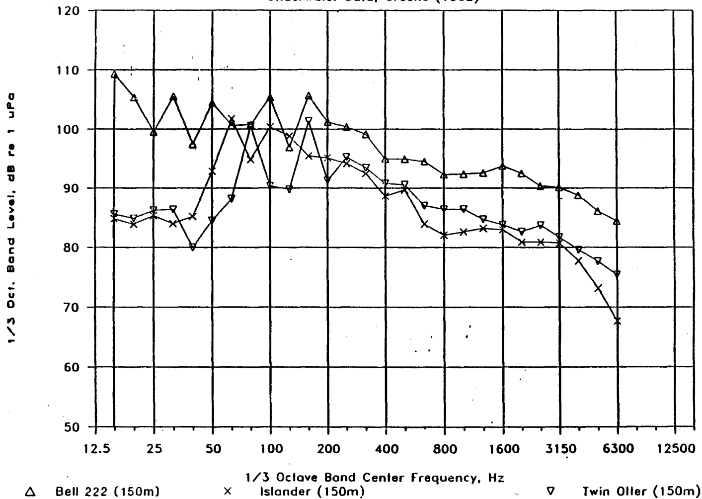
Figure 14. Aircraft noise spectra, underwater data (Greene 1982).
