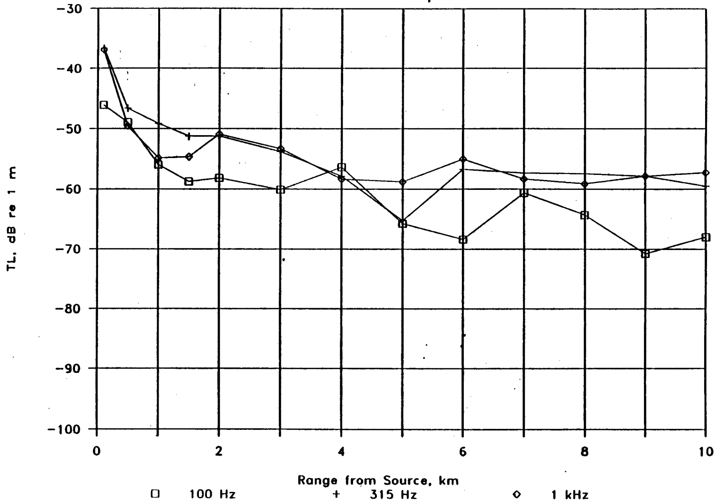
Figure 10. Transmission loss near Unimak Island, depth = 70 m
