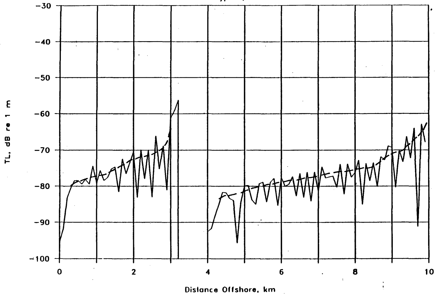
Figure 7. Offshore transmission loss
