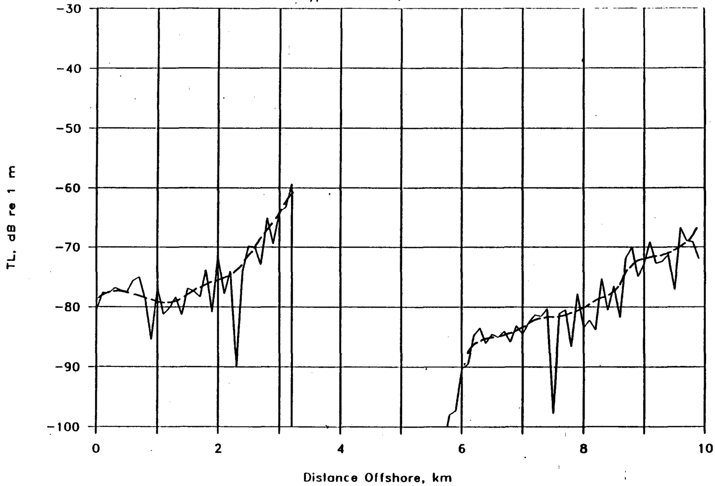
Figure 9. Offshore transmission loss
