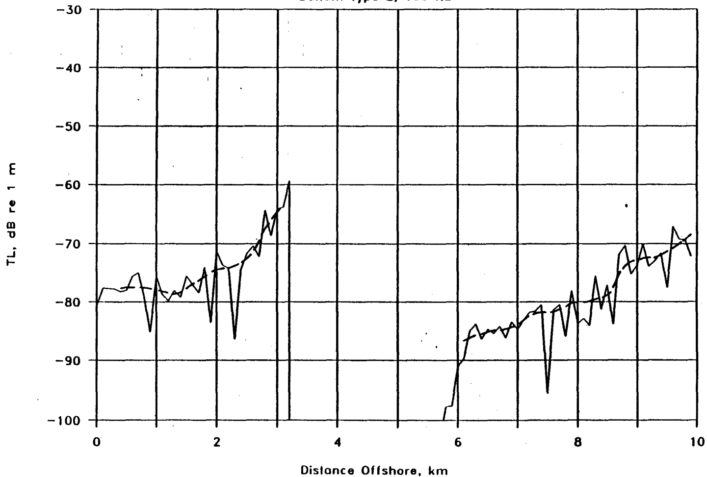
Figure 8. Offshore transmission loss
