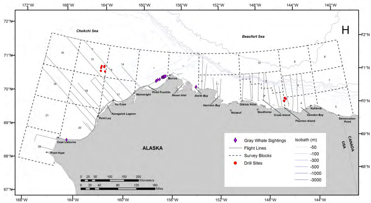
Figure 21 (cont). ASAMM semimonthly gray whale sightings, with transect, search and circling effort, 2012. Deadhead flight tracks are not shown. G: 1-15 October; H: 16-28 October.
