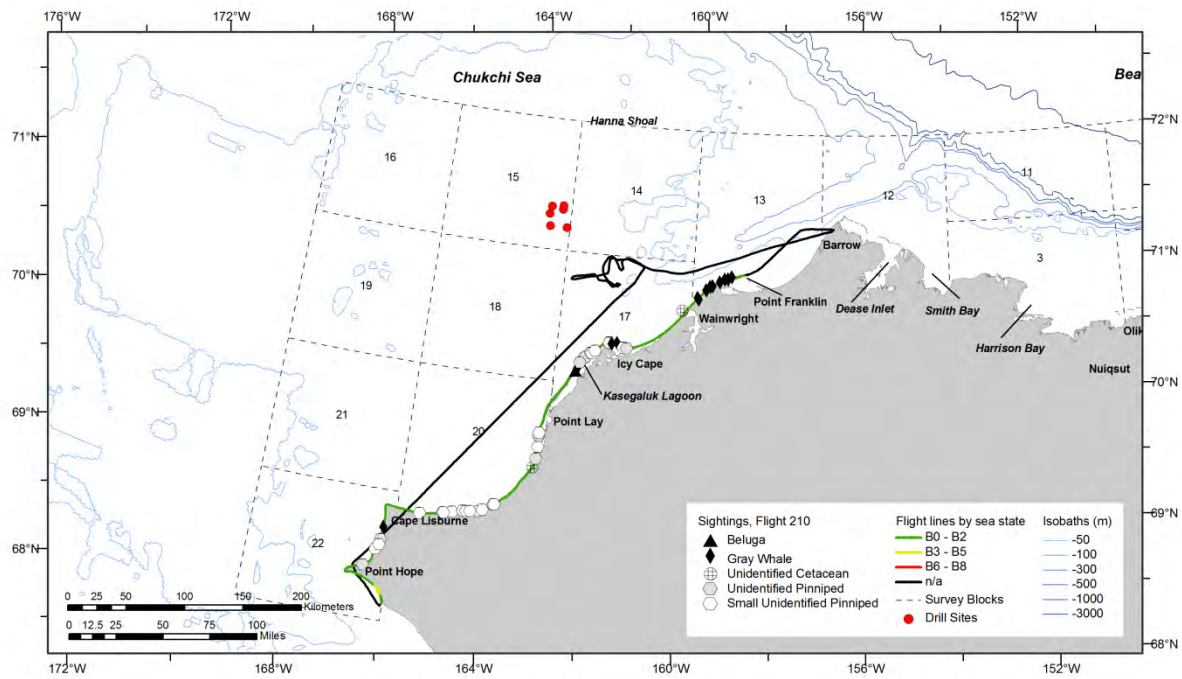
Figure B-19. ASAMM Flight 210 survey track, depicted by sea state, and all sightings.
