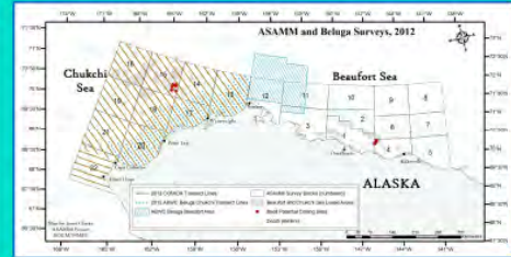
Figure 1. ASAMM and Beluga survey study area, 2012.
