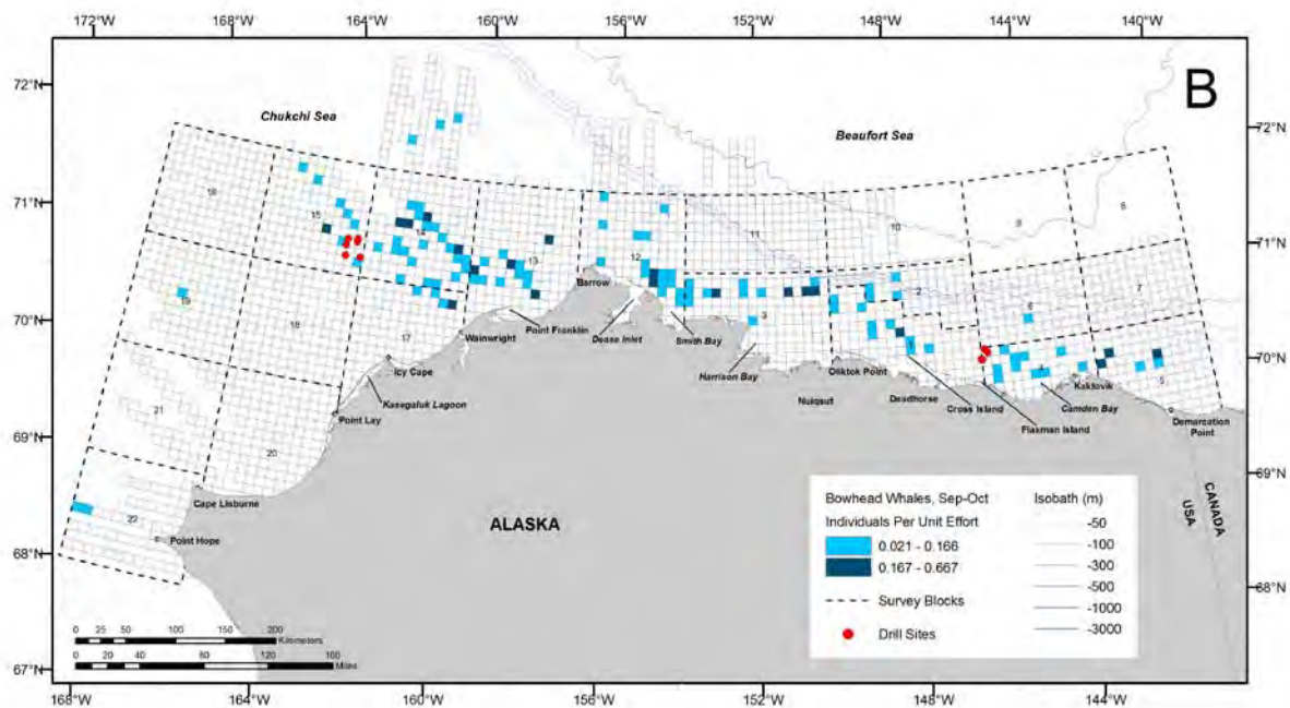
Figure 8. ASAMM bowhead whale sighting rates (whales on transect/km of transect surveyed), (A) summer (June-August); and (B) fall (September-October), 2012. Transect sightings from primary observers only. Empty grid cells have sighting rates of zero; transect survey effort was not conducted in areas without grid cells.
