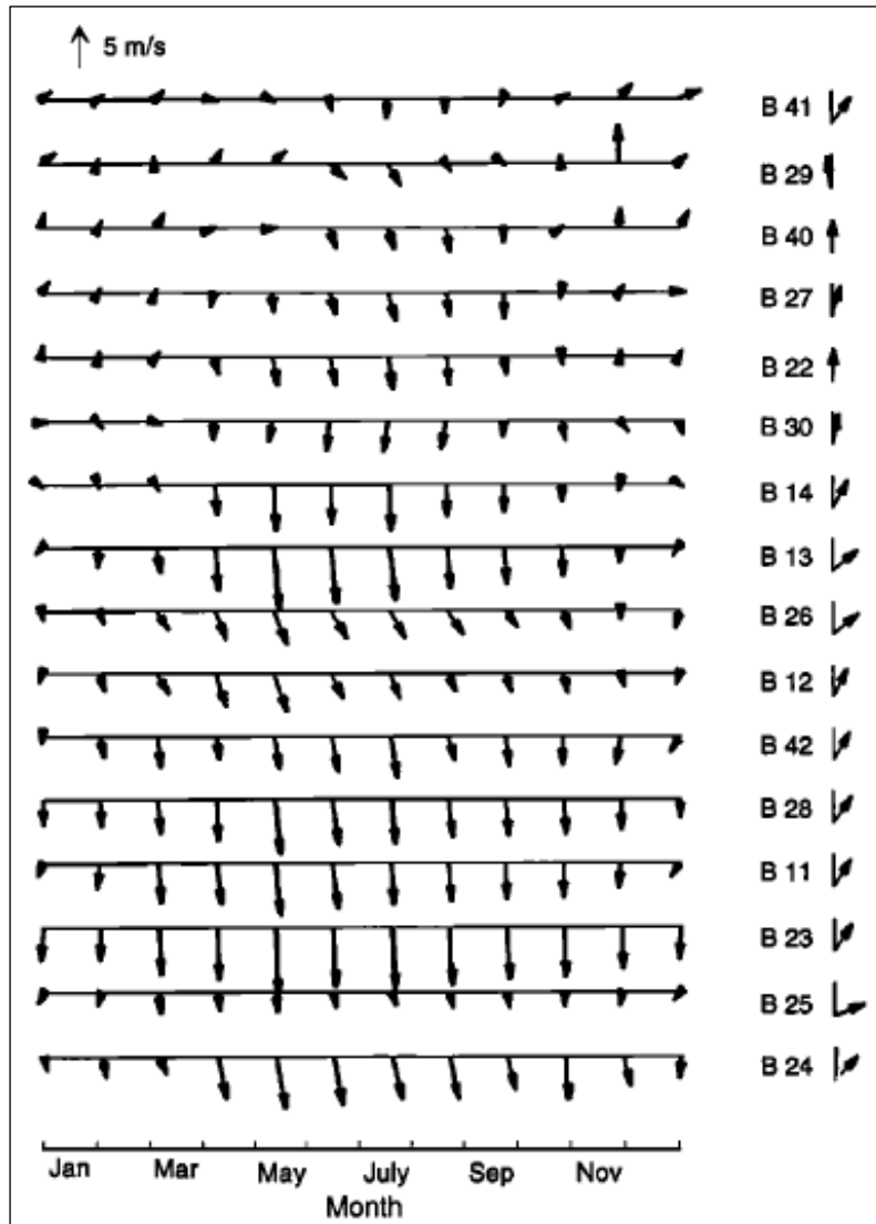
Figure 1.9. Annual cycle of the wind as recorded by NDBC buoys. For each location the vertical direction corresponds to the predominant direction of flow or “principal axes.” The relative orientation of that direction from north is shown at the right with the vectors pointing due north. The last two digits of each NDBC buoy are shown on the right, so that “B 41” refers to NDBC buoy 46041.
