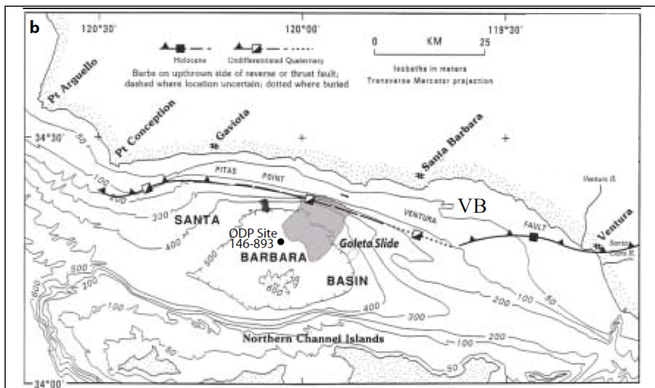
Figure 16.3. Location of major faults that direct fluid to the sea floor, that can rupture during earthquakes. (Greene et al. 2006)
