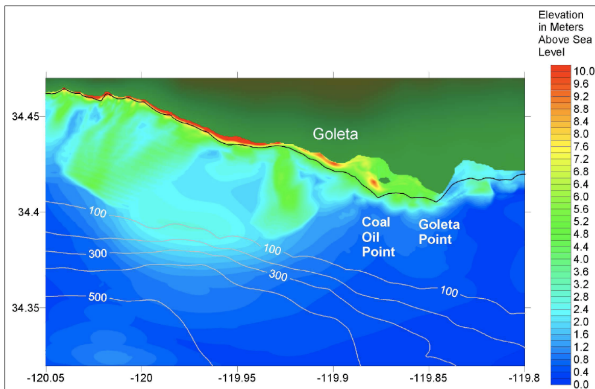
Figure 16.1. Maximum tsunami amplitudes from numerical simulation of the tsunami generated by the Western segment of the Goleta slide.
