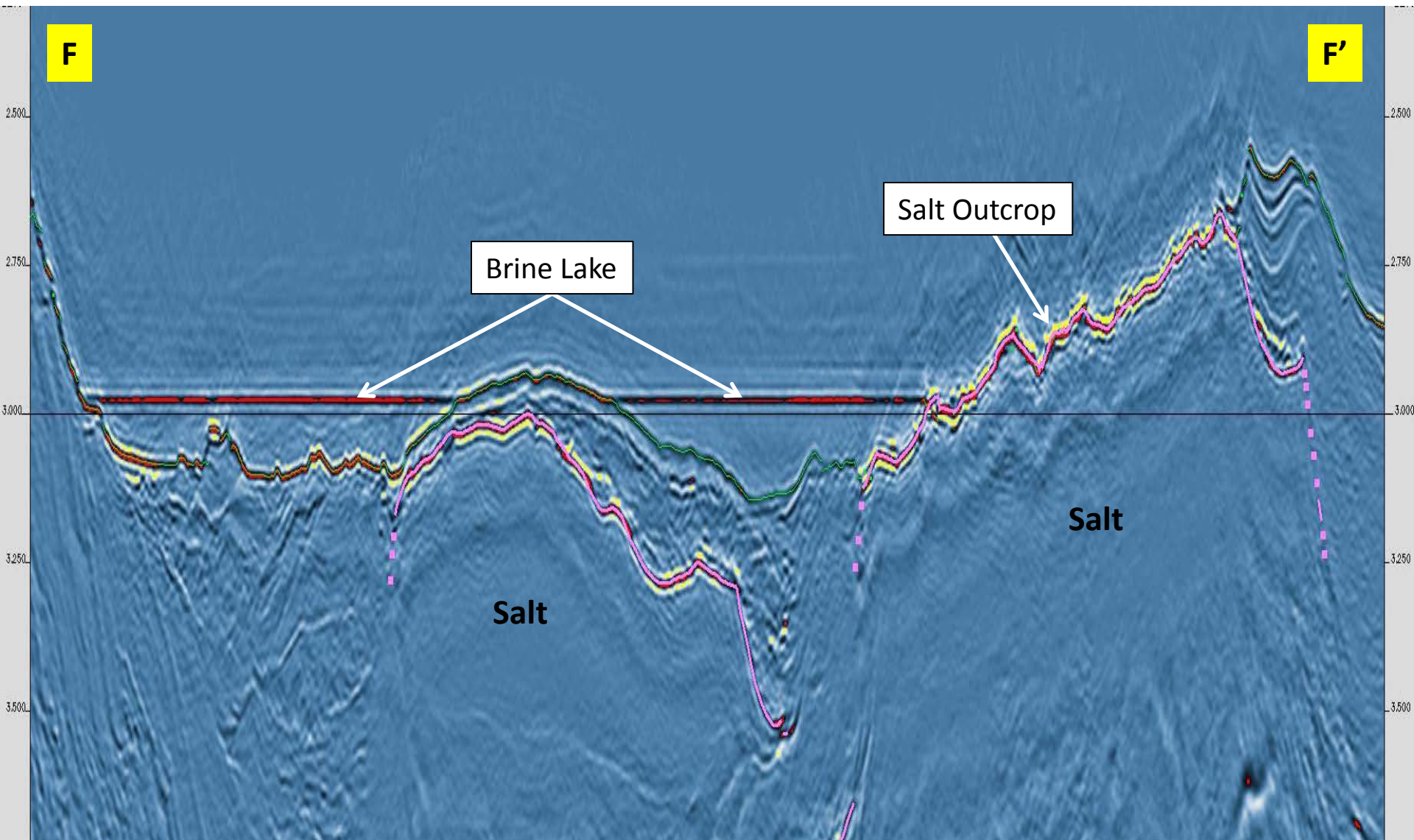
Figure 13 – E-W Seismic Line F-F' Showing Salt Outcropping at the Seafloor and Associated Brine Lake
