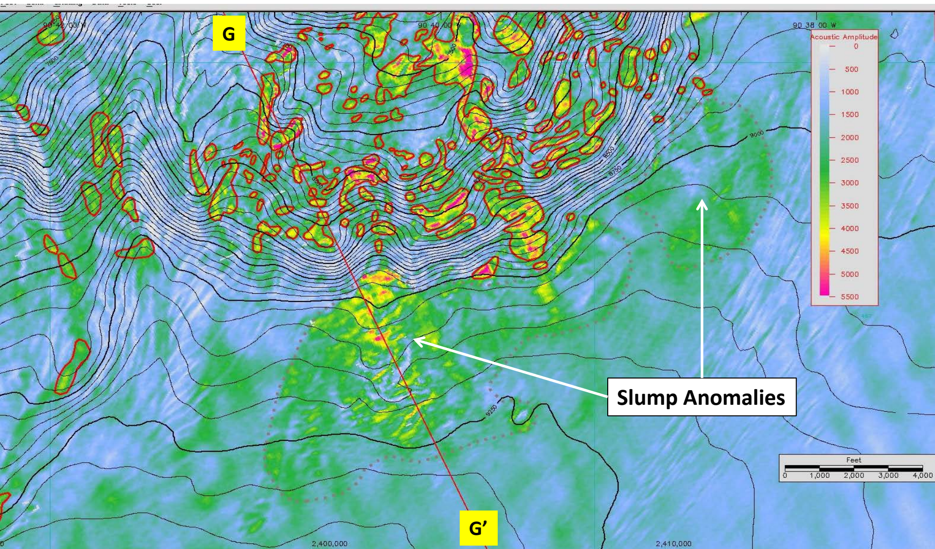
Figure 14 – Bathymetry/Amplitude Map Showing Slump Anomalies
