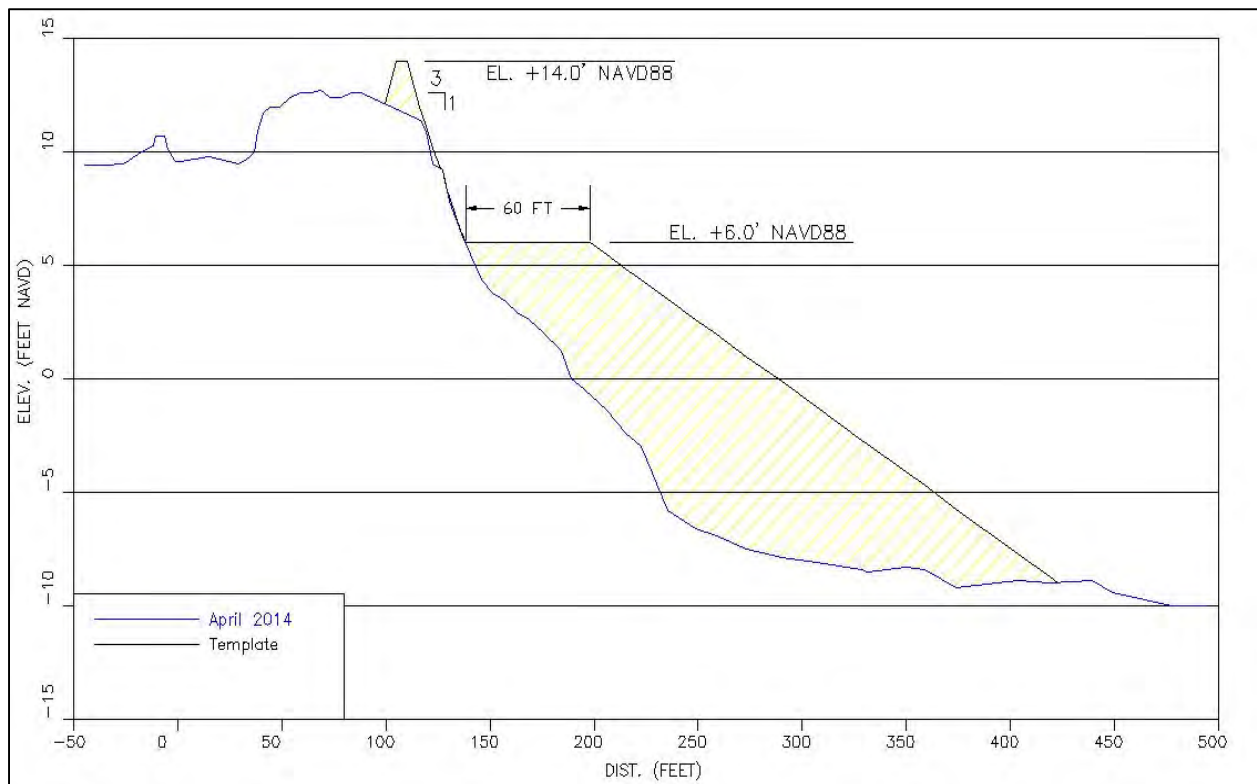
Figure 5. Typical design template for the Town of Kitty Hawk Shoreline Protection Project.
