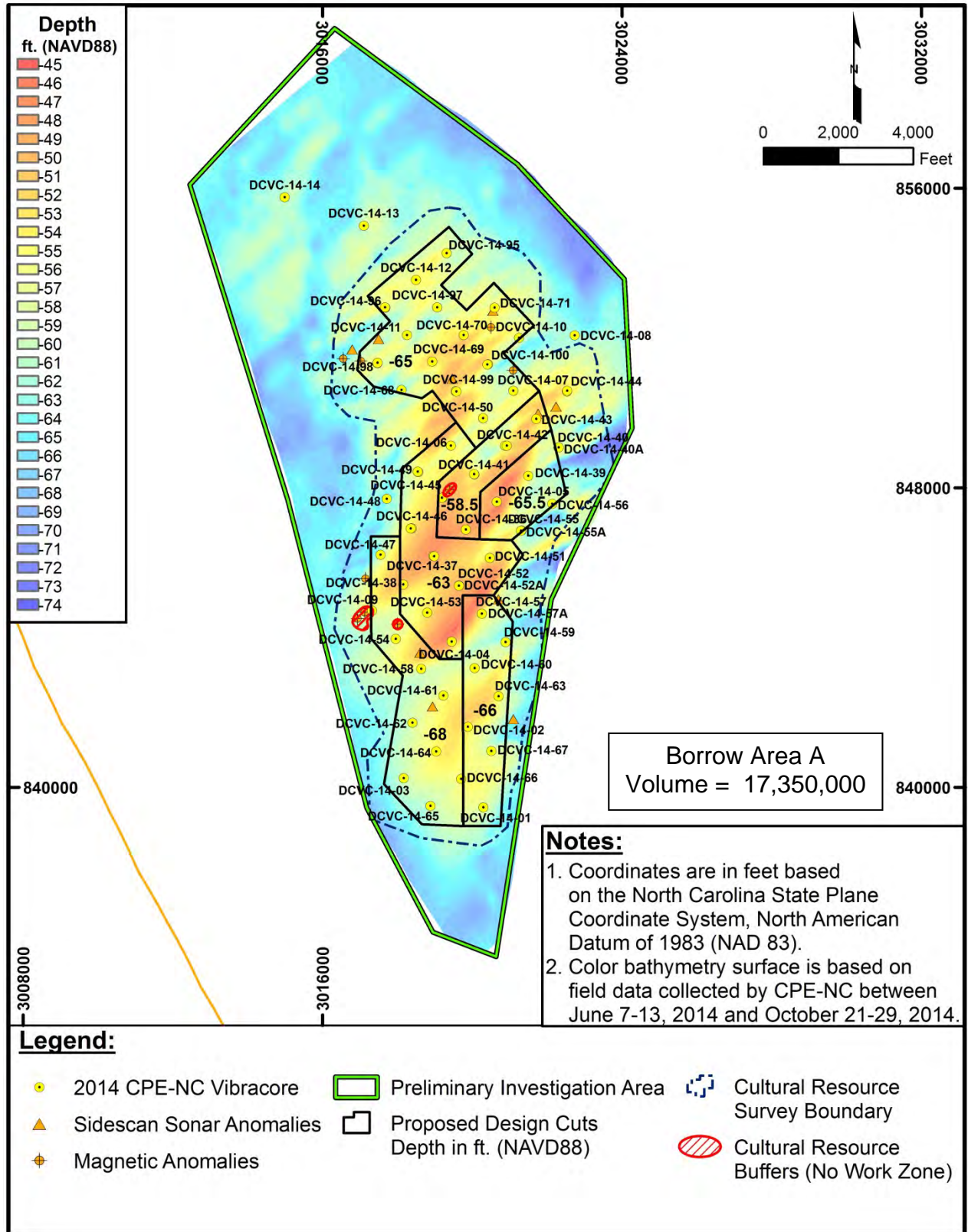
Figure 6. Map of Borrow Area A, showing preliminary design cuts, locations of vibracores, and cultural resource buffers. Locations of other identified magnetic anomalies and side scan sonar anomalies deemed not culturally significant are also shown.
