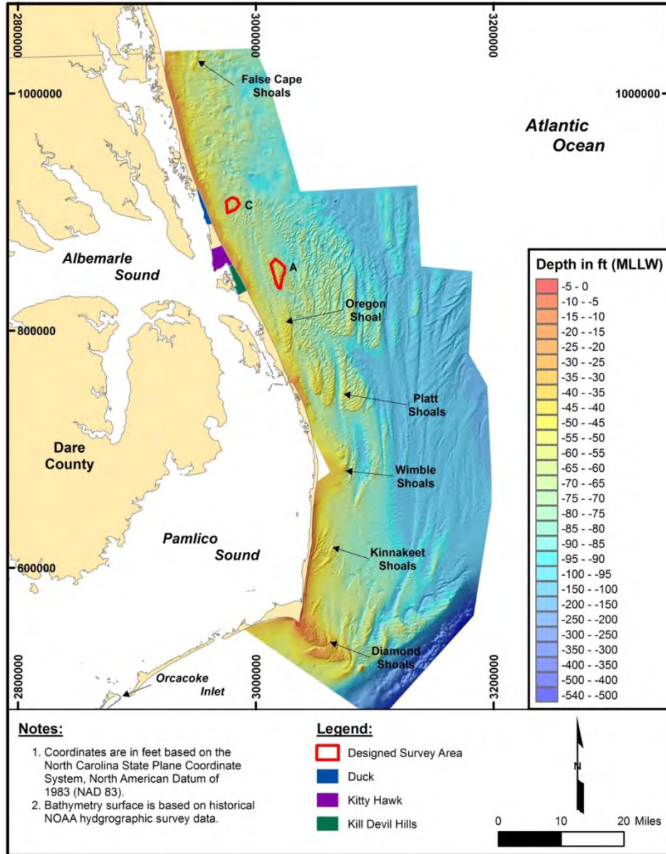
Figure 10. Regional bathymetry with potential borrow areas and major shoal features.
