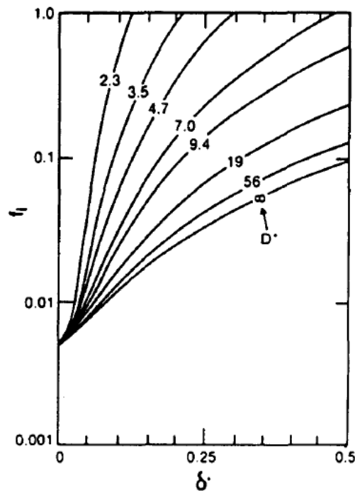
Figure 21: Friction factor as a function of the dimensionless diameter and dimensionless liquid film thickness (Bharathan and Wallis, 1983).
