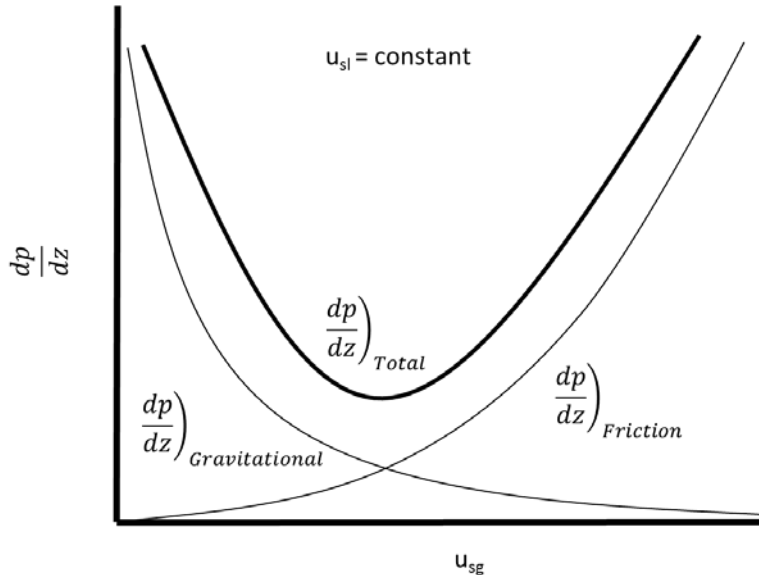
Figure 19: Schematic for pressure gradient behavior in vertical two-phase flow (Shoham, 2005).
