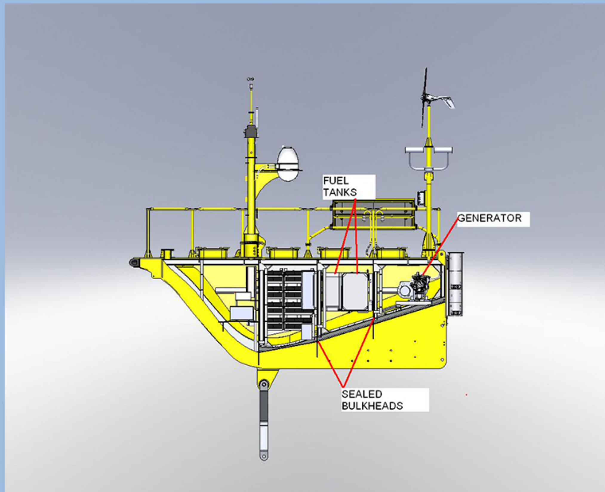
Meteorological Buoy Design
