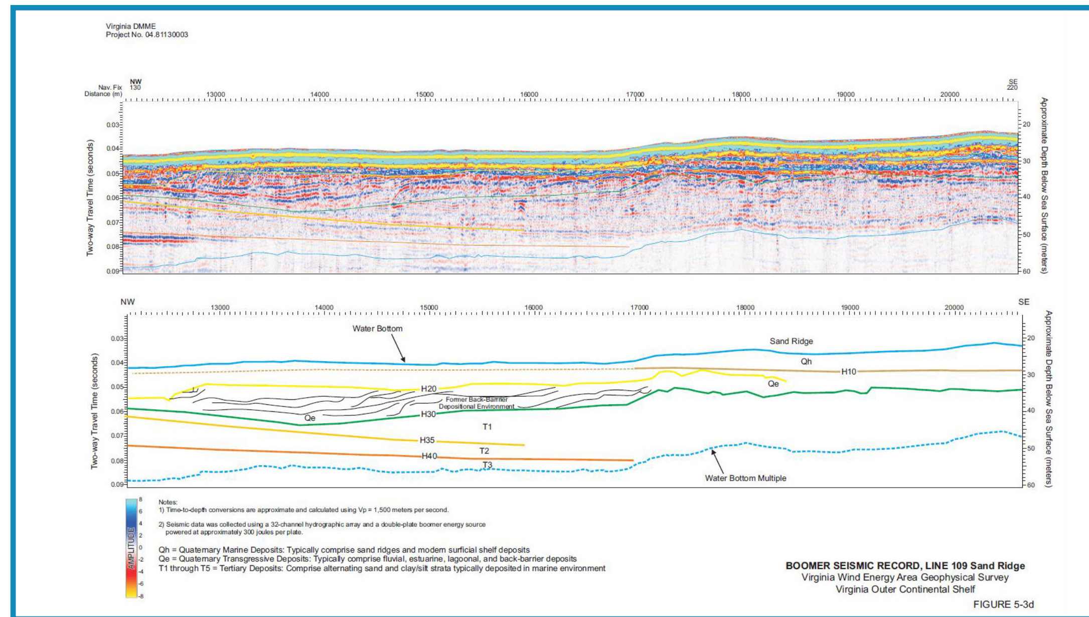
Geology of the Seafloor Using a Sub-bottom Profiler
