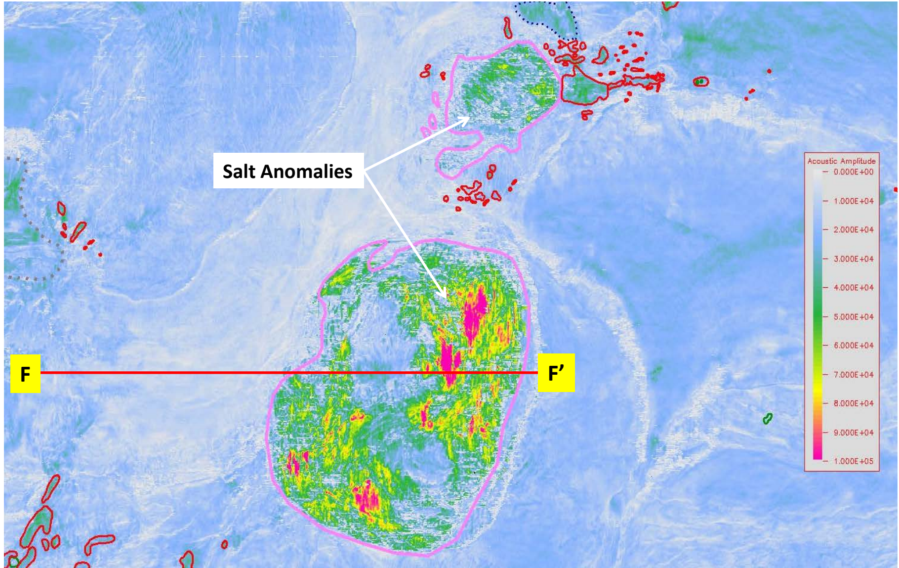
Figure 12 – Amplitude Map Showing Salt Anomalies
