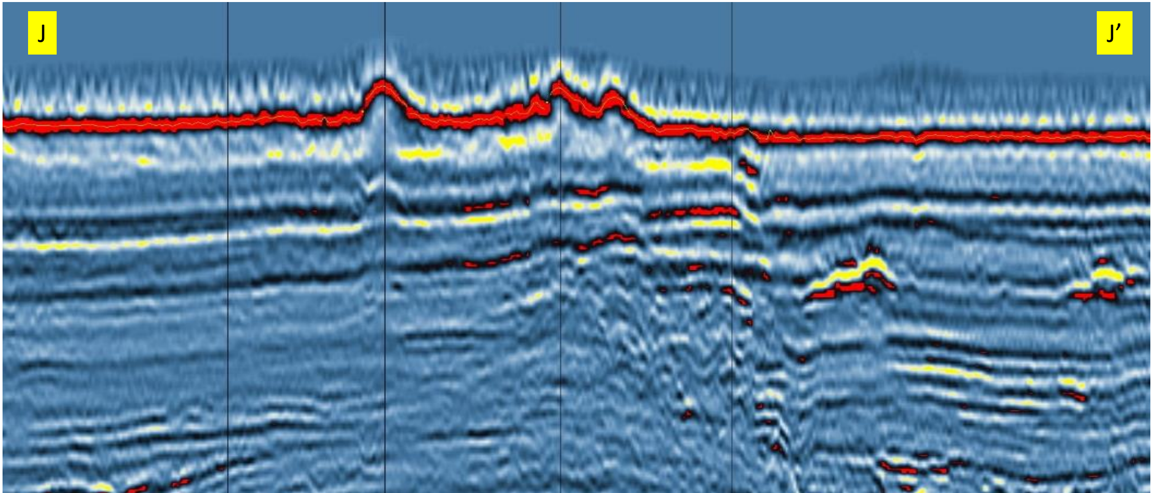
Fig. 20 – Confirmed Relic Patch Reef – E. Flower Gardens Bank NW – SE Seismic 3-D Line J-J'
