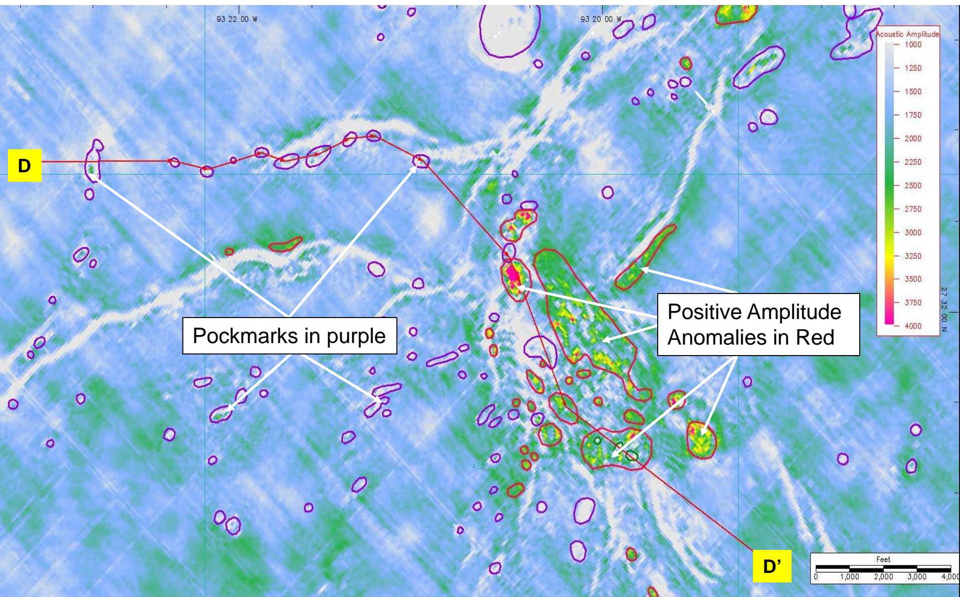
Figure 7 - Seafloor Amplitude Map Showing Pockmarks
