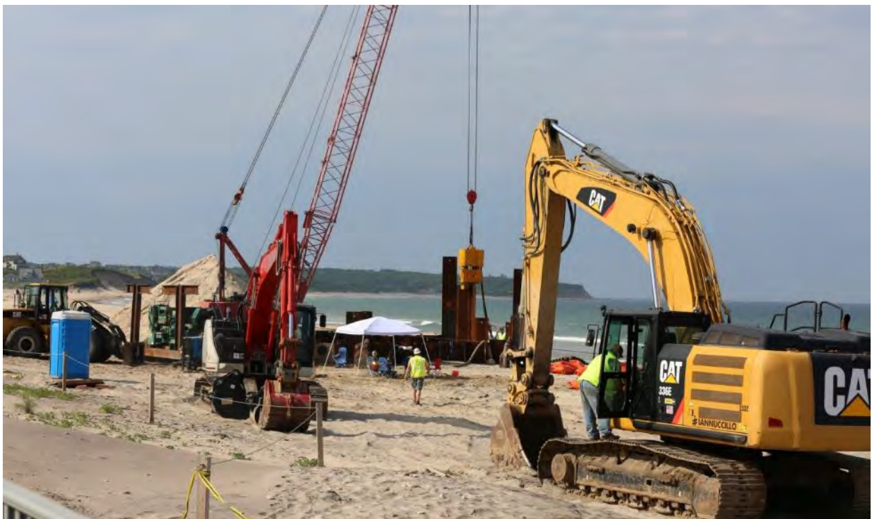
6/23/2016 Block Island Town Beach – Photo 0631: Removal of the cofferdam via vibrator gripper.
