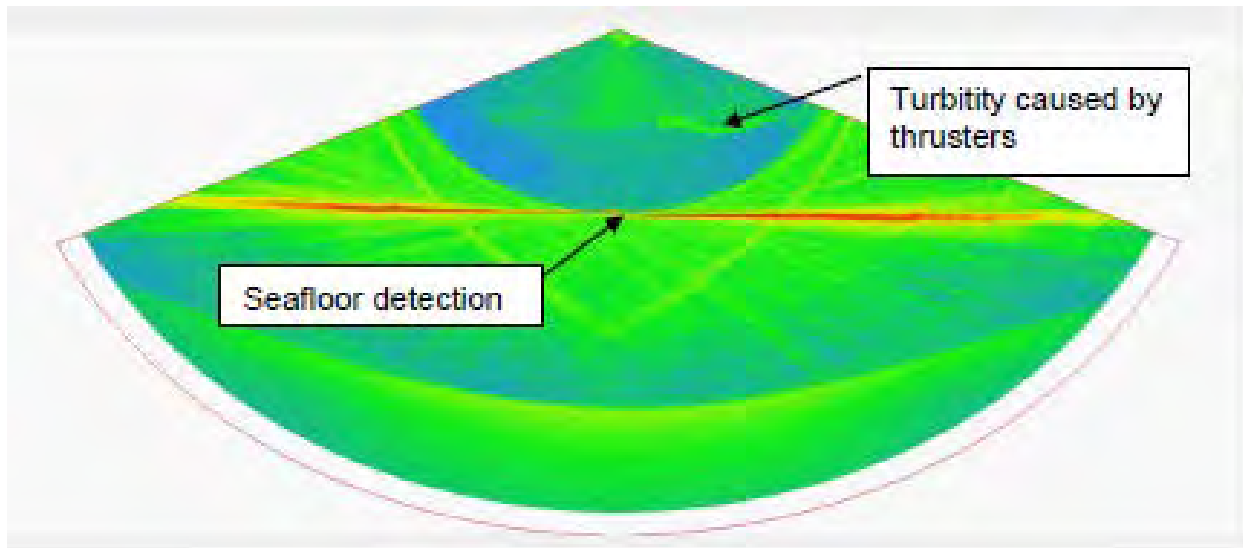
Figure 26. MBES data showing turbidity in the water column from the vessel thrusters. Taken from Bathymetric Survey Plume Monitoring Report (Fugro Pelagos Inc, 2016)
