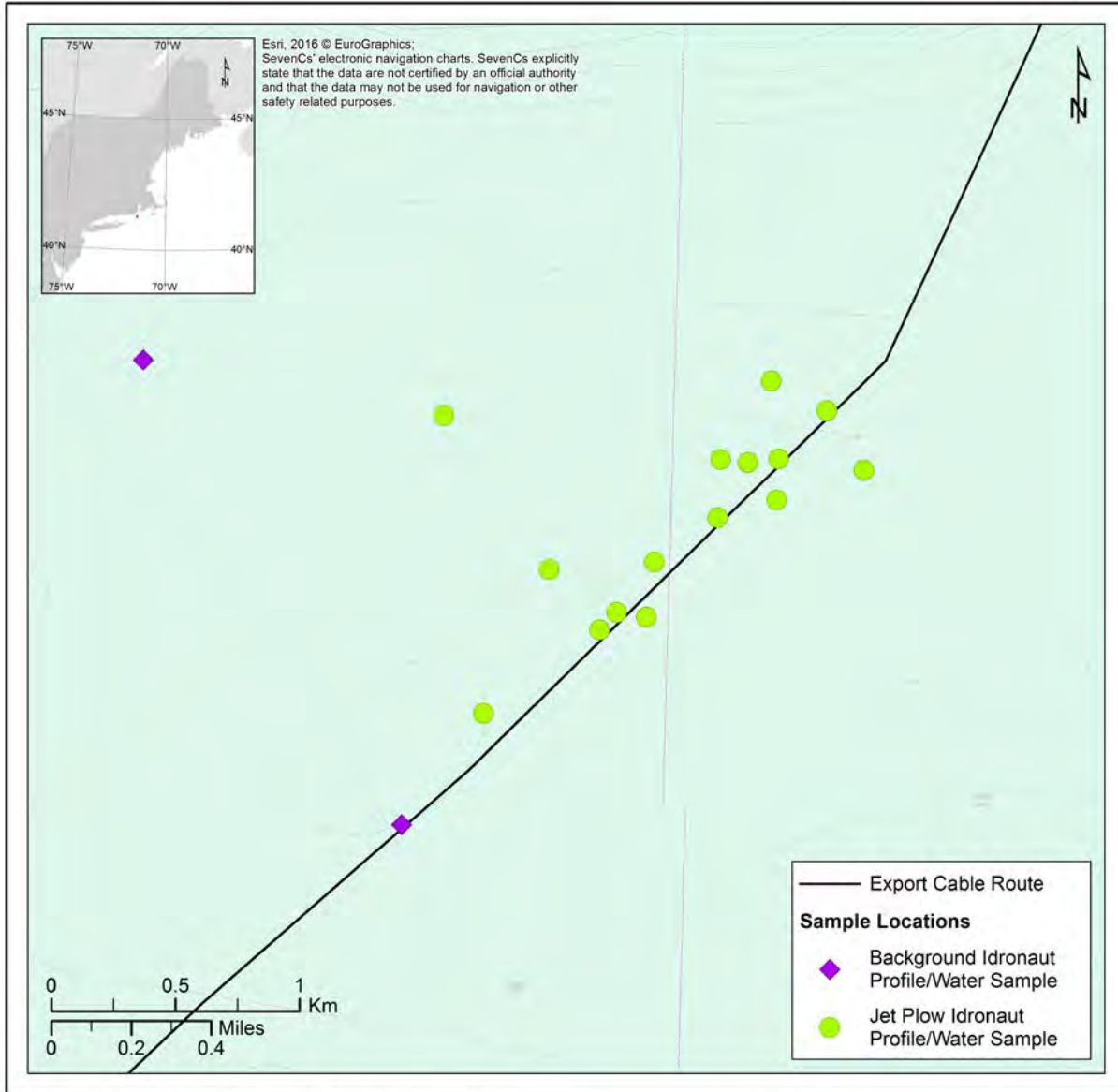
Figure 15. Location of Jet Plow Idronaut turbidity profiles and water samples
