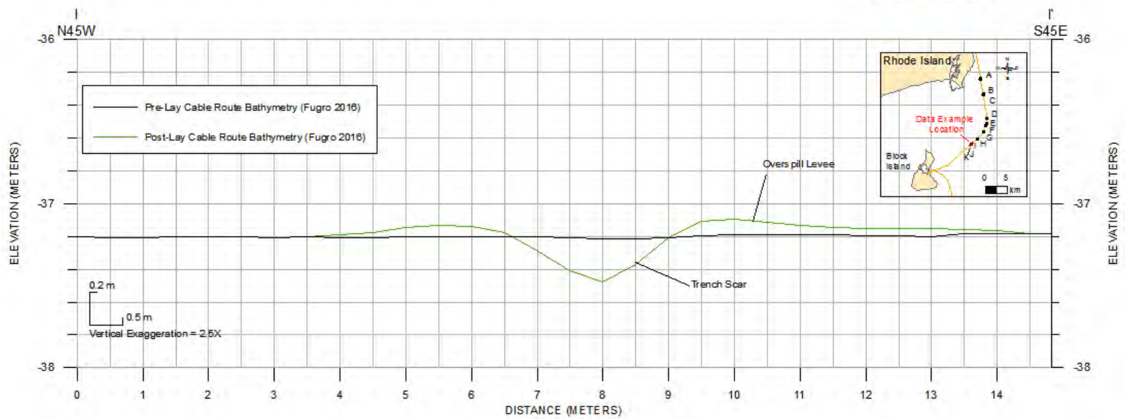
Figure 29. Trench morphology shown in cross section profile
