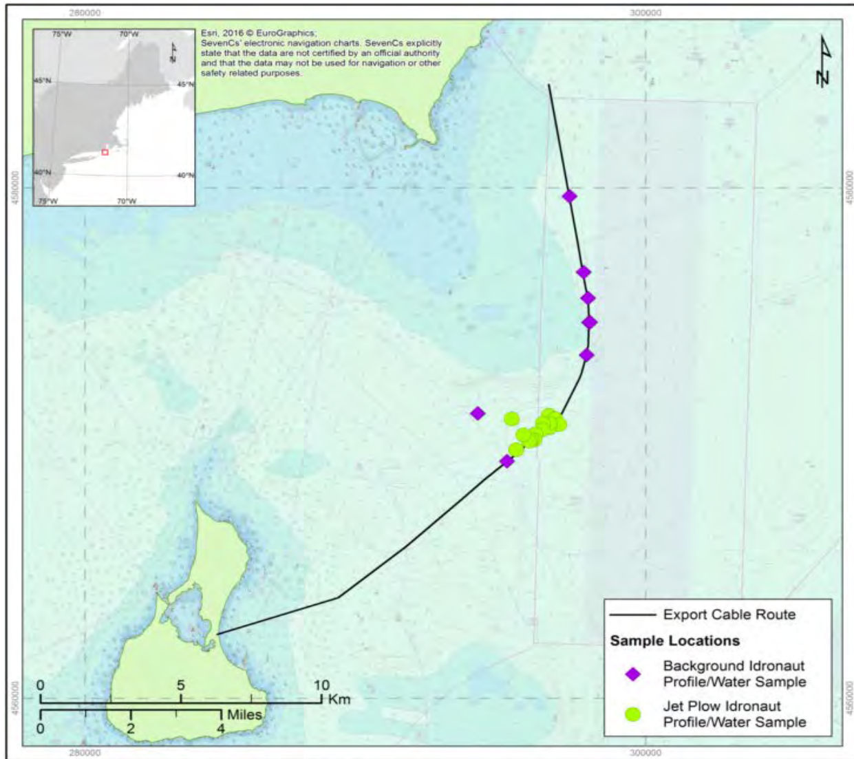
Figure 13. Locations of Idronaut turbidity profiles and water samples along cable route
