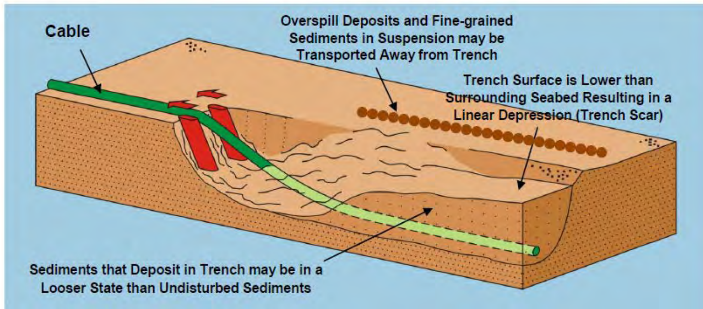
Figure 28. Schematic of jet-trenching process and trench morphology
