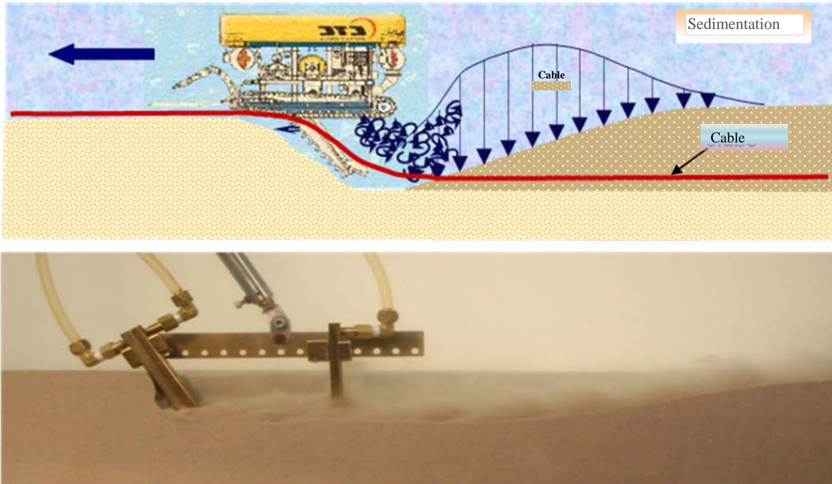
Figure 27. Schematic Illustration of a jet-trencher during operation (Van den Berghe et al., 2008)
