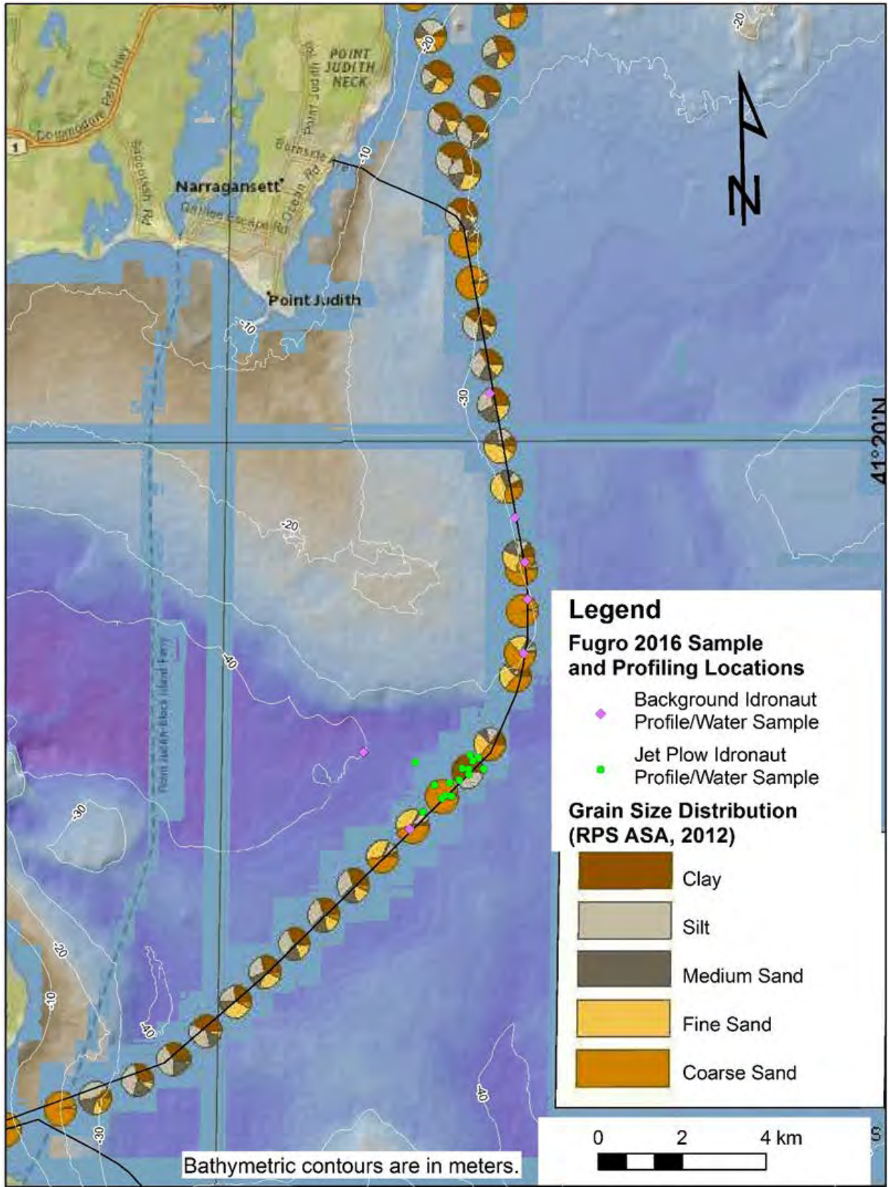
Figure 14. Seafloor sediment characteristics along cable route.
