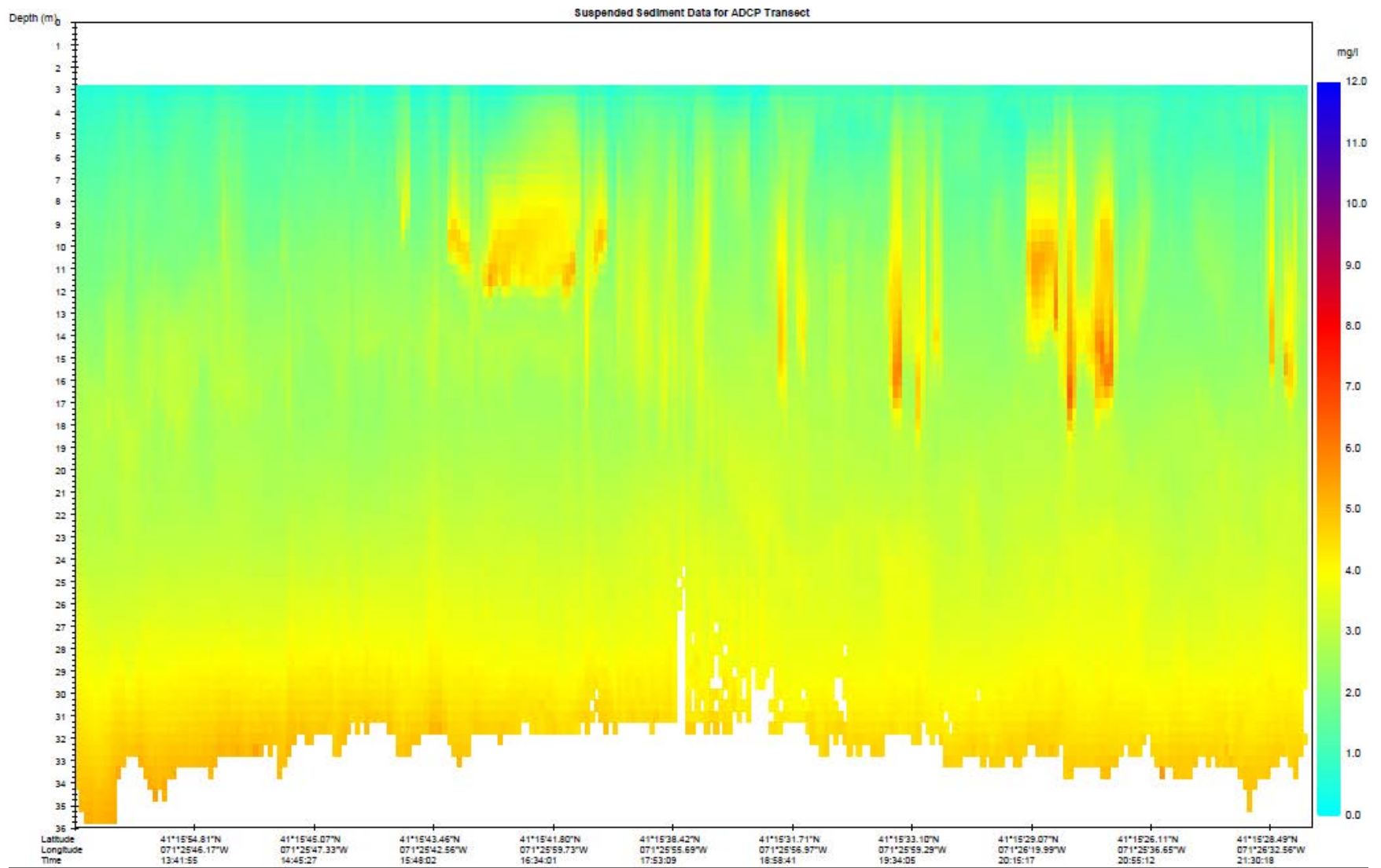
Figure 23. ADCP data showing increased turbidity as a result of instrumentation passing vessel thrusters
