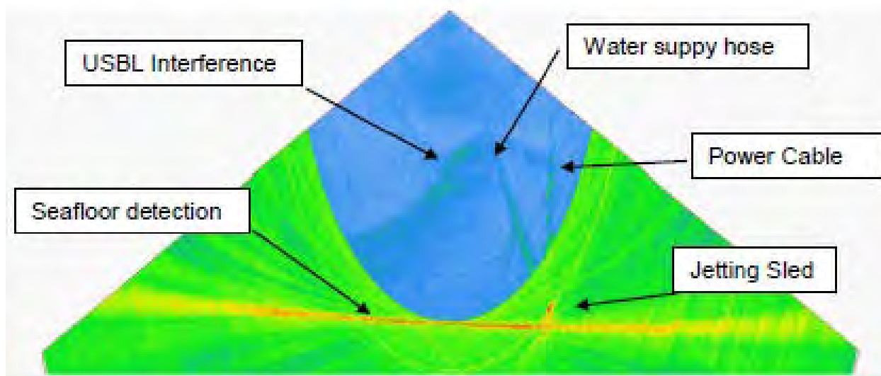
Figure 25. MBES data obtained from next to the jet plow. Image taken from Bathymetric Survey Plume Monitoring Report (Fugro Pelagos Inc., 2016)
