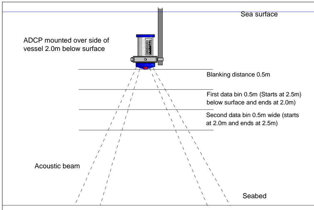
Figure 16. ADCP configuration for vessel-mounted works
