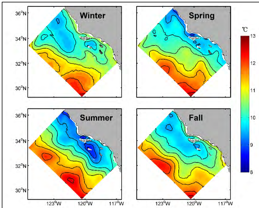
Figure 26. Same as Figure 25, but for 100 m.
