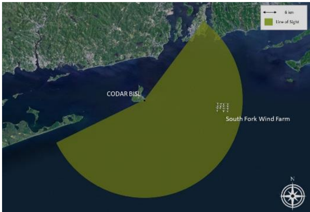
Figure 208 - South Fork, SeaSonde, BISL
