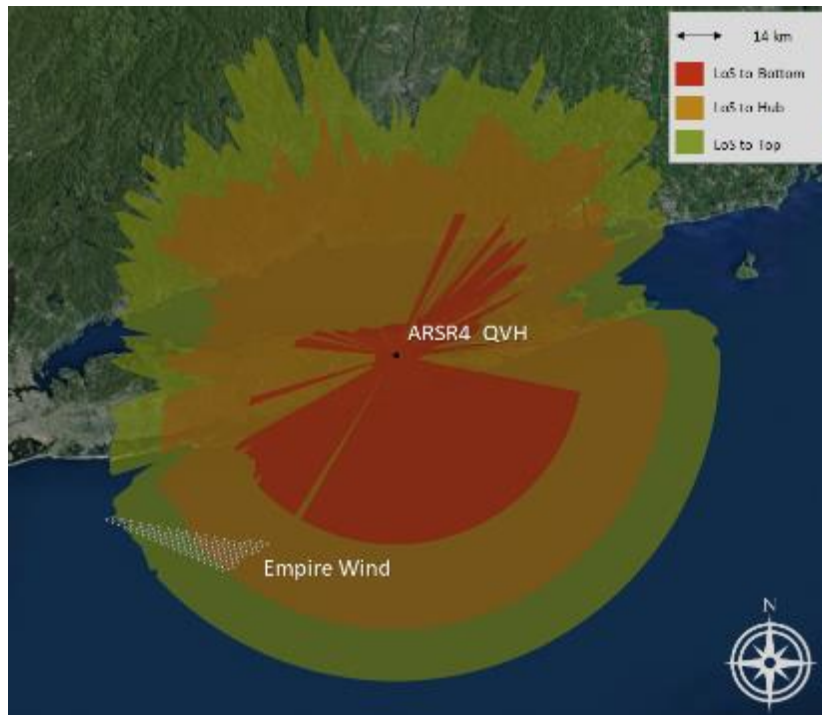
Figure 236 - Empire Wind, ARSR-4, QVH
