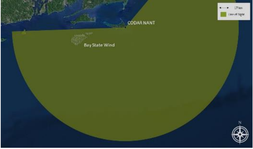
Figure 202 - Bay State, SeaSonde, NANT
