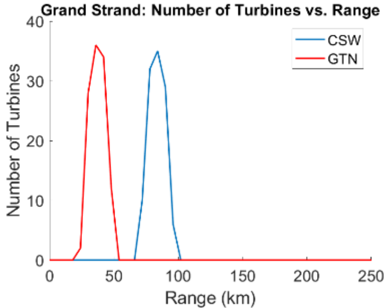
Figure 174 - Number of turbines in each range bin for the long range SeaSondes near the Grand Strand farm.
