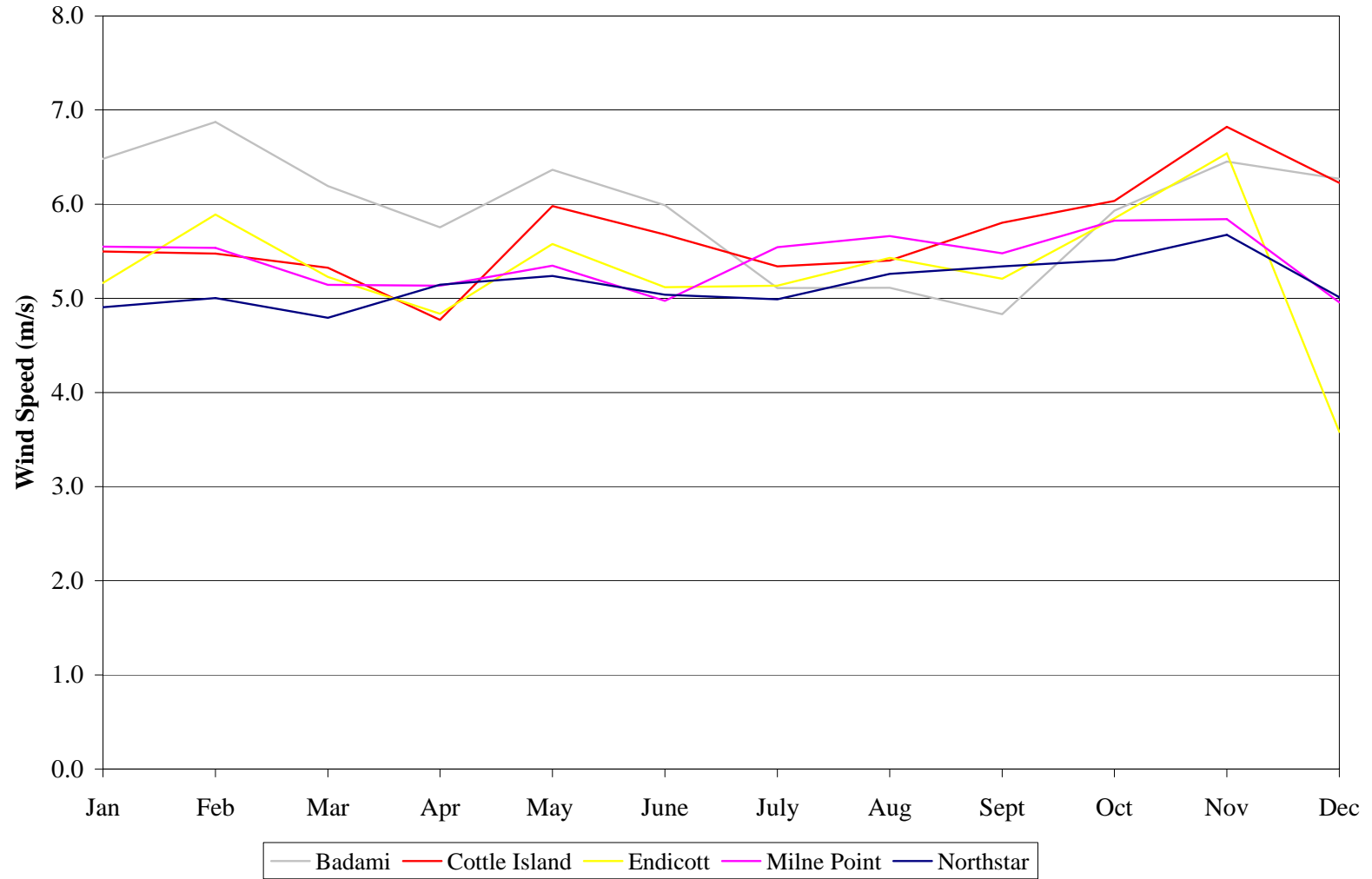
Figure 4-3 Mean Adjusted Monthly Wind Speed
