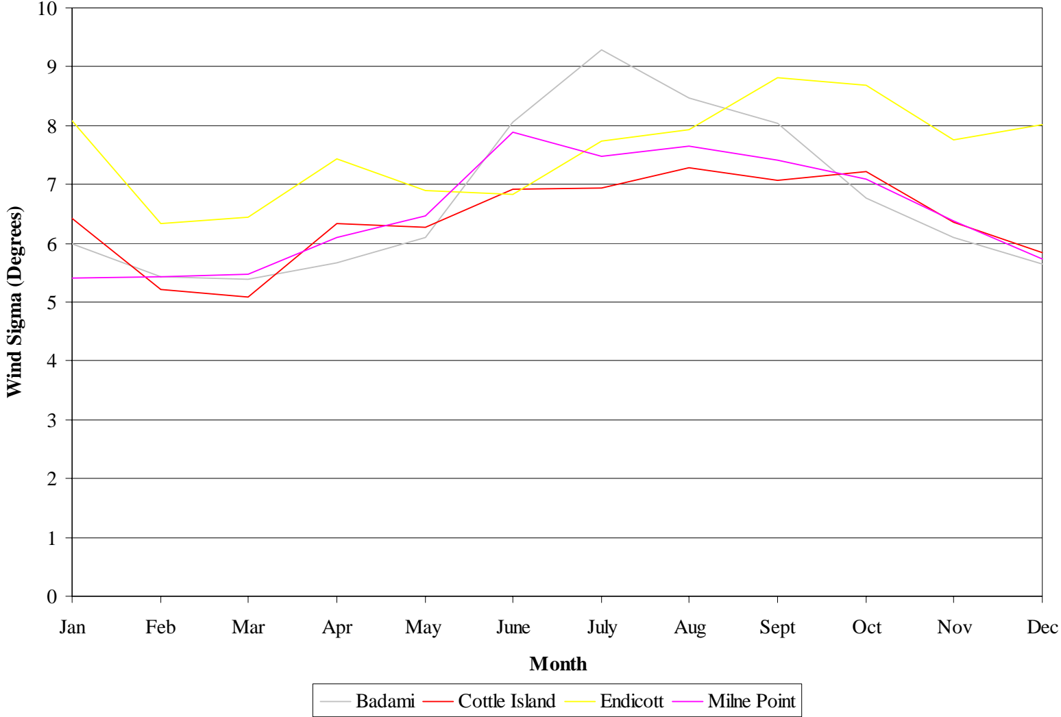
Figure 4-15 Mean Monthly Wind Sigma
