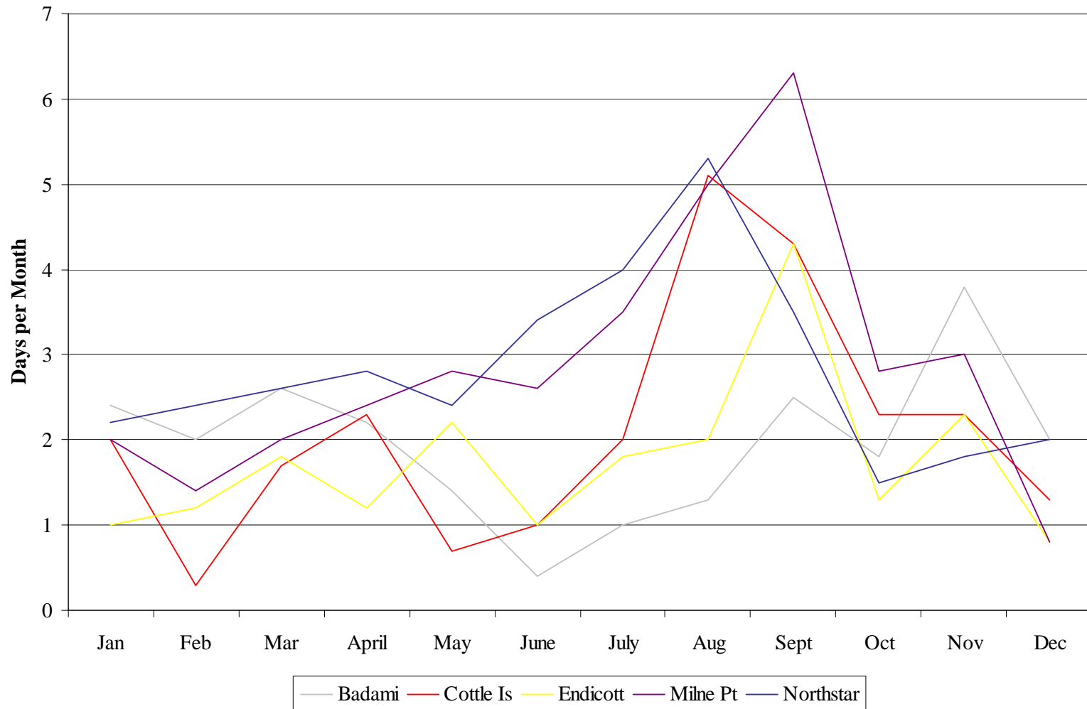
Figure 4-13 Frequency of Shore-Parallel Winds
