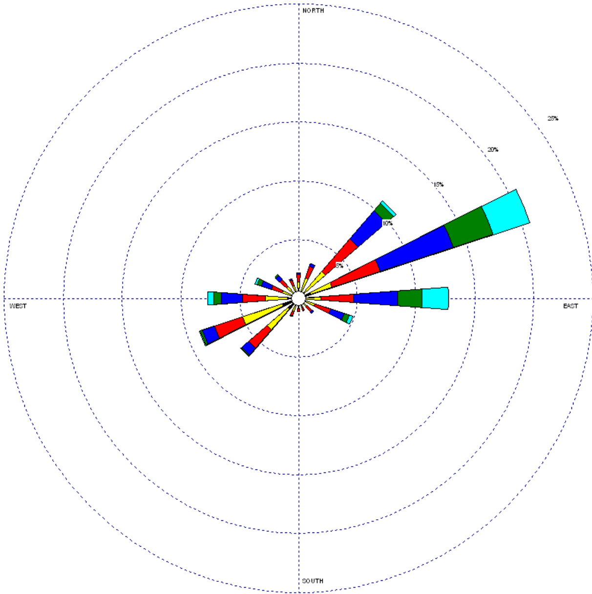
Figure 4-7 Mean Endicott Wind Rose
