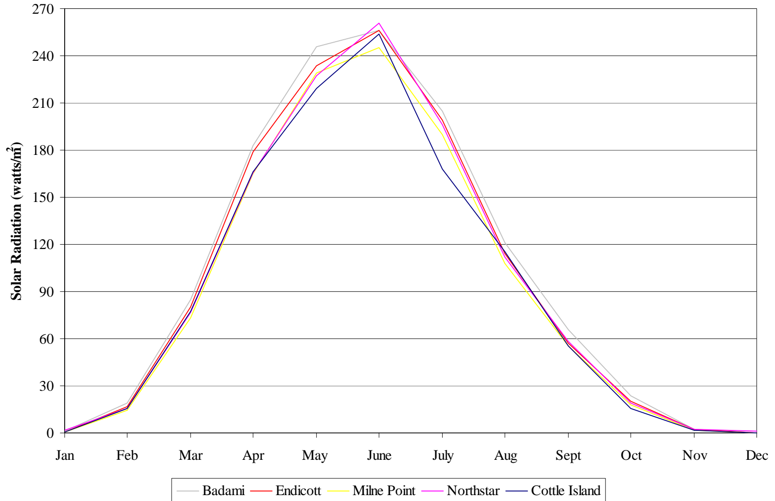
Figure 4-20 Mean Monthly Solar Radiation
