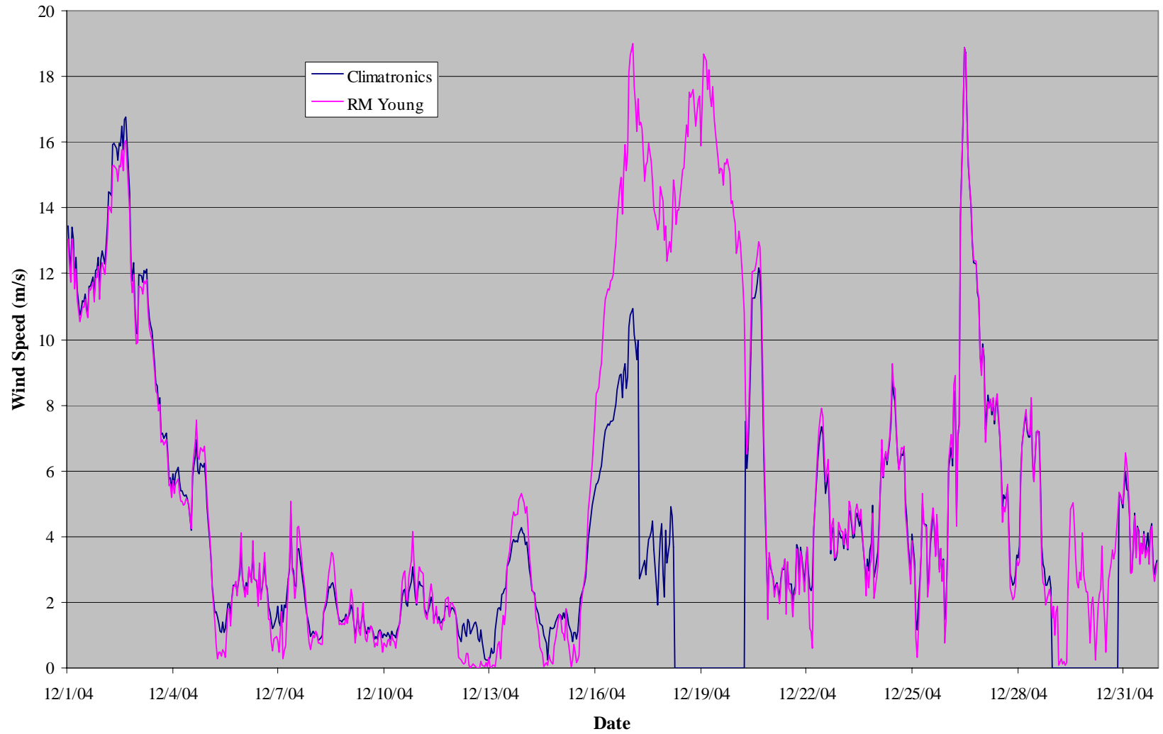
Figure 5-2 Climatronics vs. RM Young Measured Wind Speed
