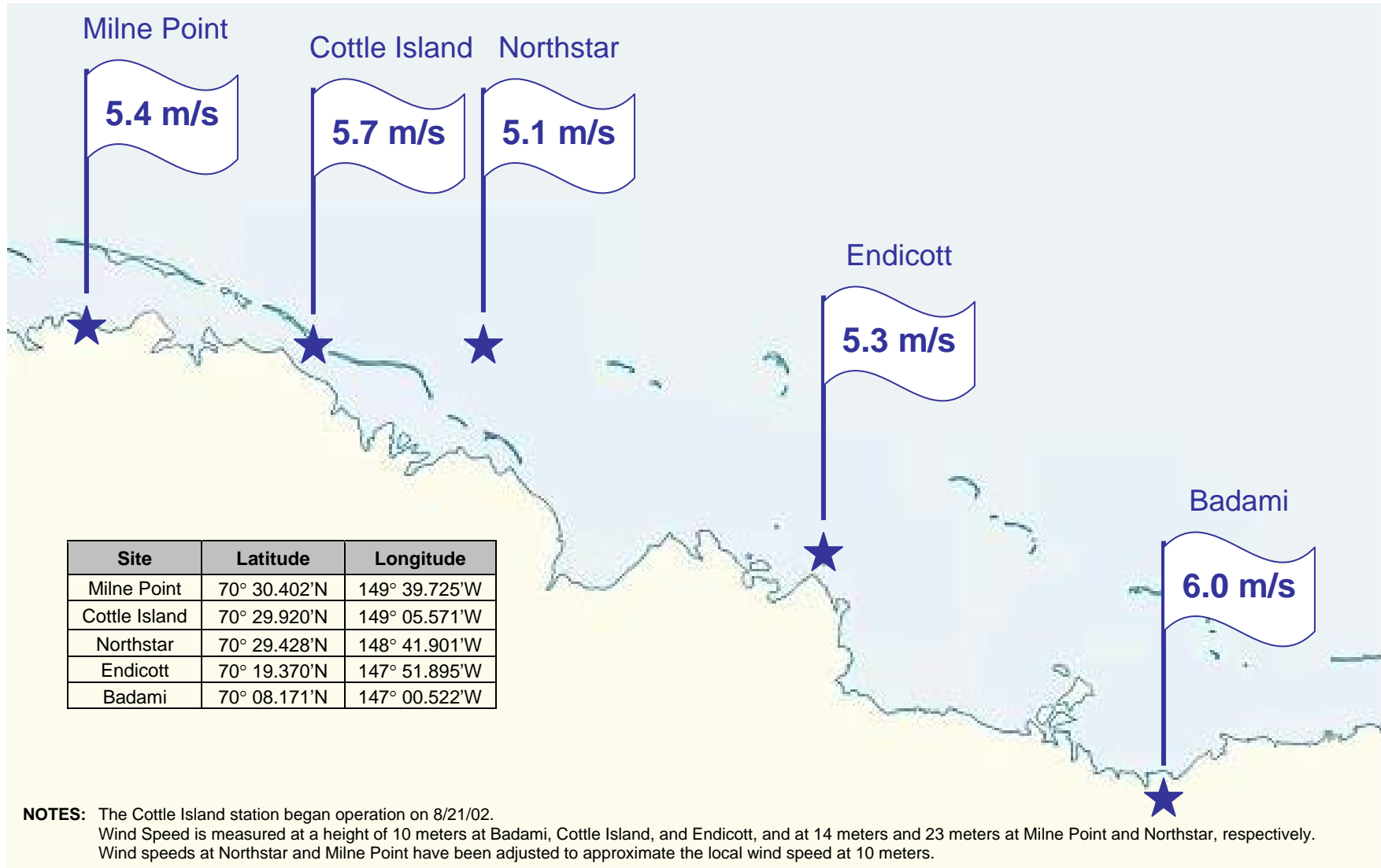
Figure 4-1 Spatial Distribution of Average Hourly Wind Speed
