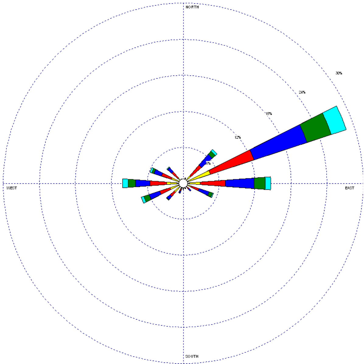
Figure 4-9 Mean Northstar Wind Rose
