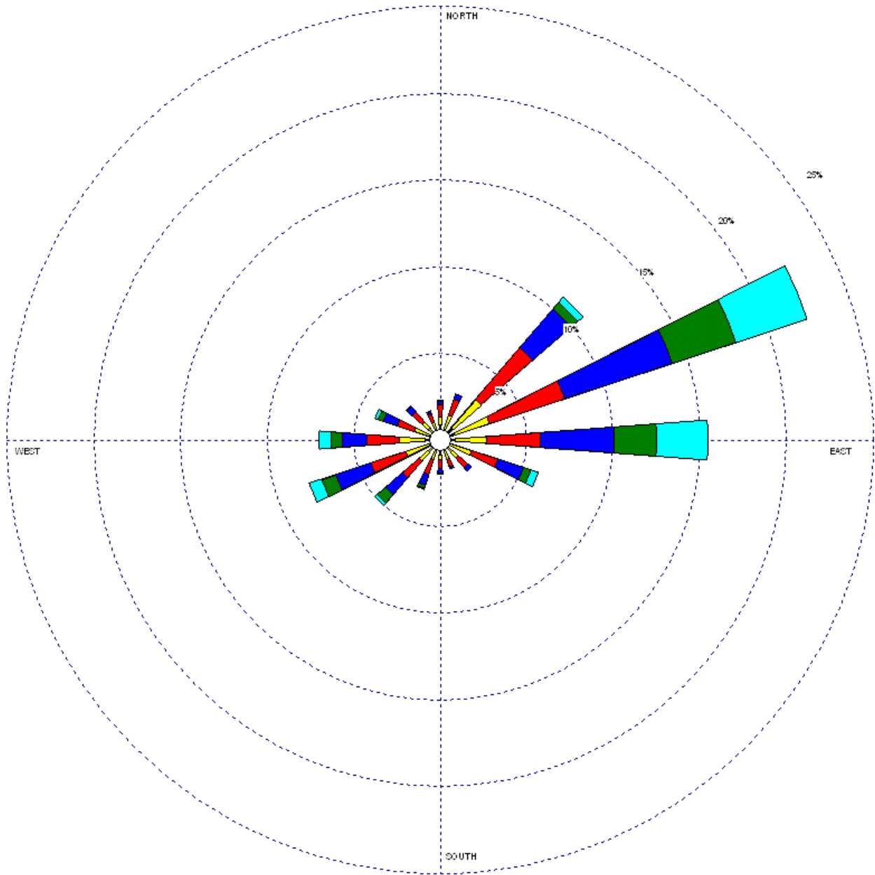
Figure 4-6 Mean Cottle Island Wind Rose
