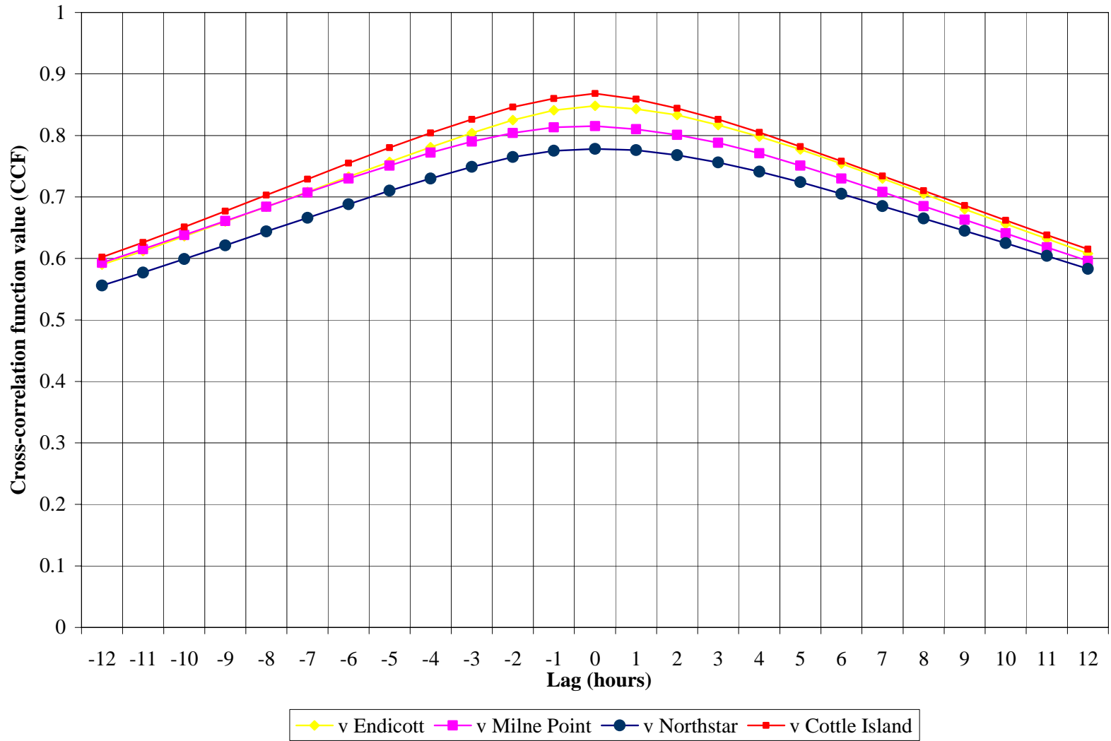
Figure 5-6 Cross Correlation of Wind Speed between Badami and Other Stations at Various Lags
