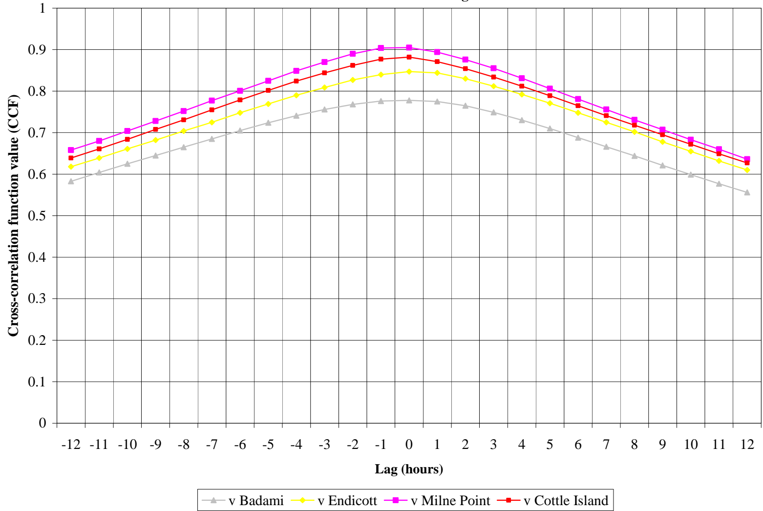
Figure 5-10 Cross Correlation of Wind Speed between Northstar and Other Stations at Various Lags
