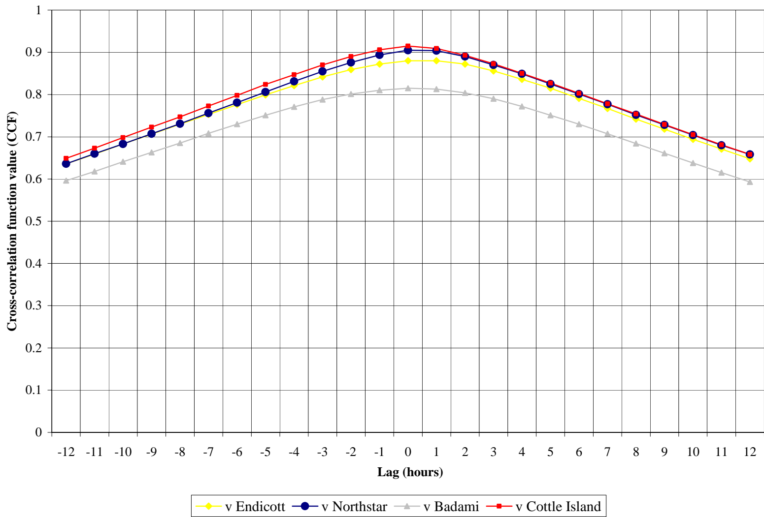
Figure 5-9 Cross Correlation of Wind Speed between Milne Point and Other Stations at Various Lags
