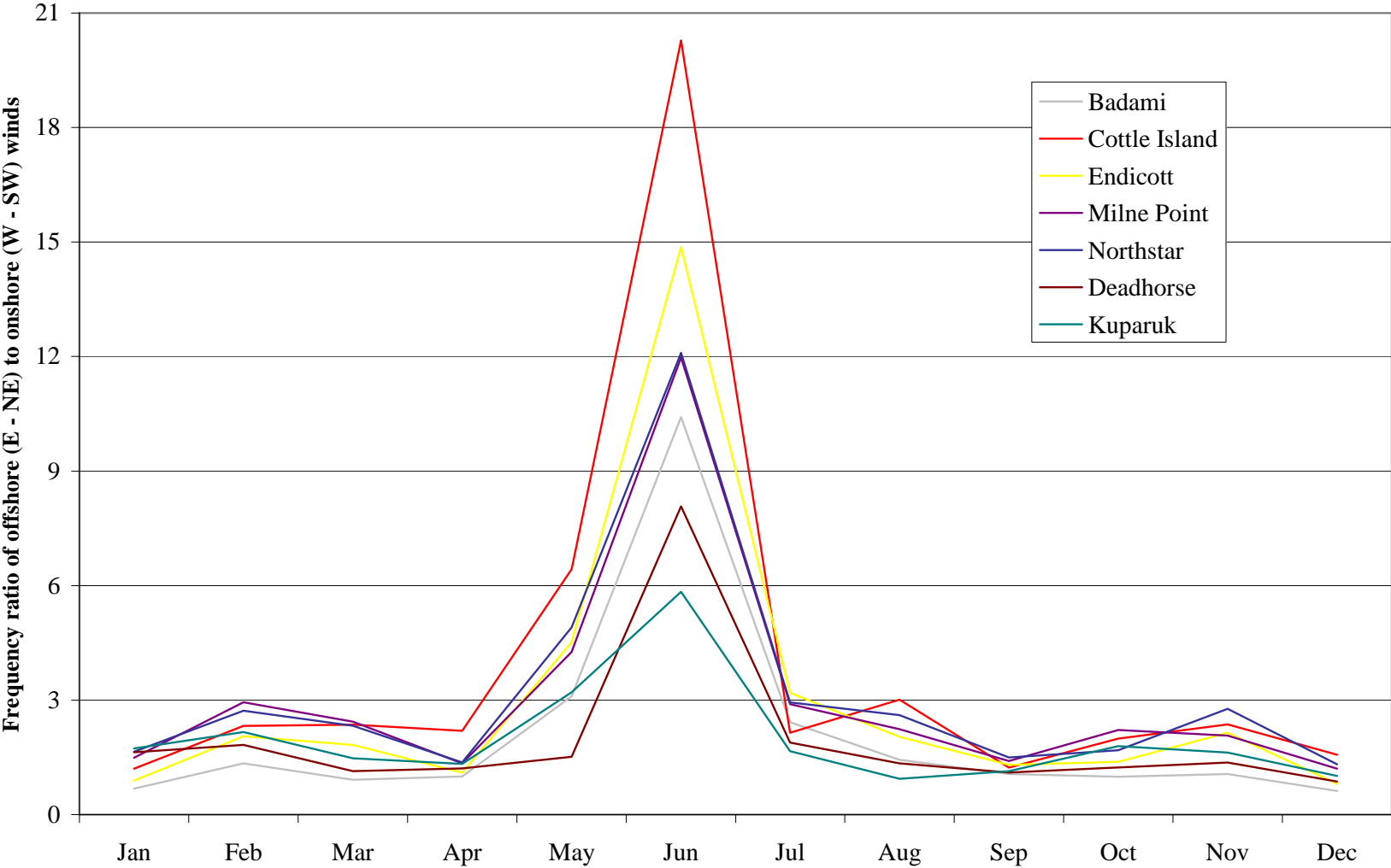
Figure 5-3 Frequency Ratio of Offshore (E - NE) to Onshore (W - SW) Winds by Month
