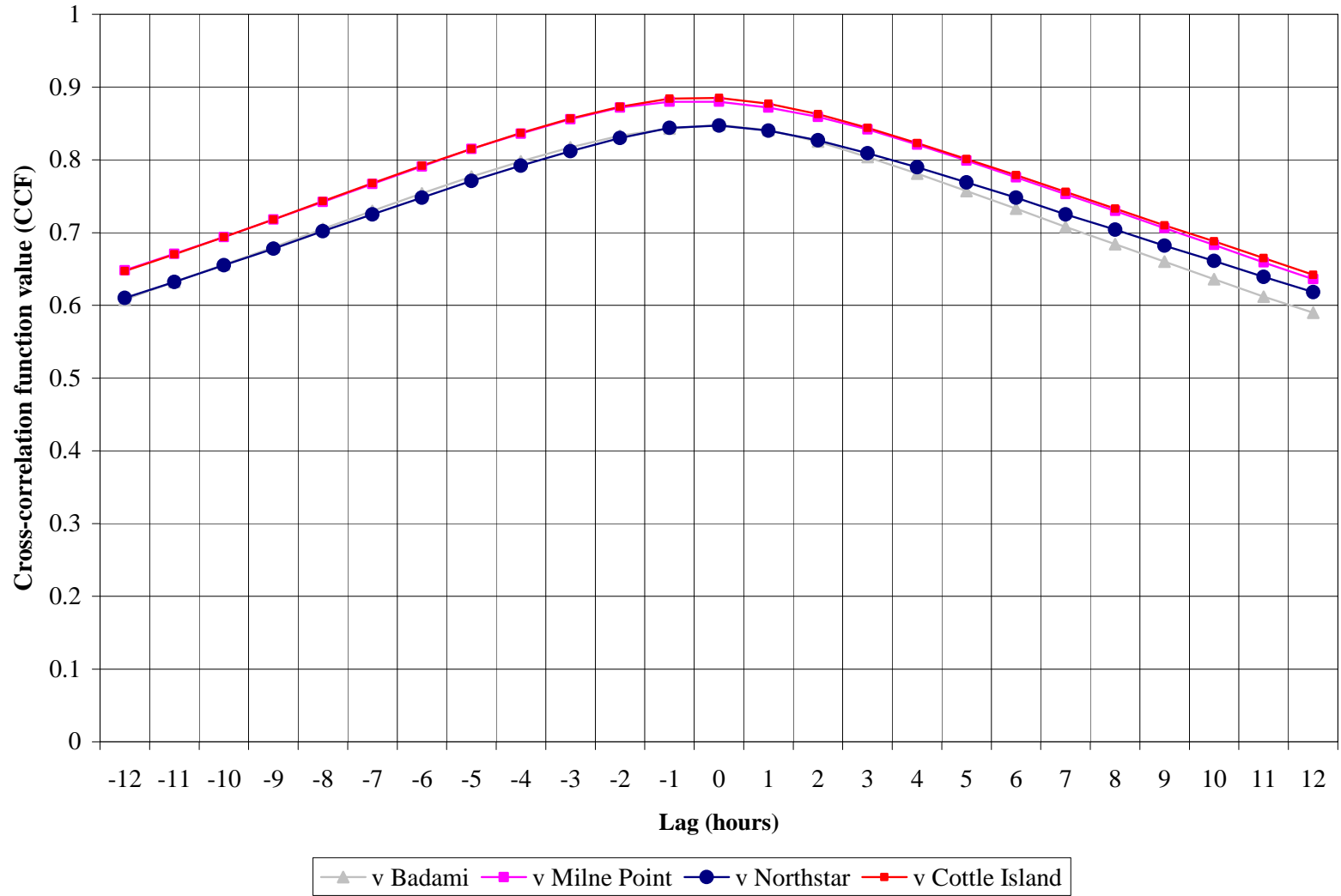
Figure 5-7 Cross Correlation of Wind Speed between Endicott and Other Stations at Various Lags
