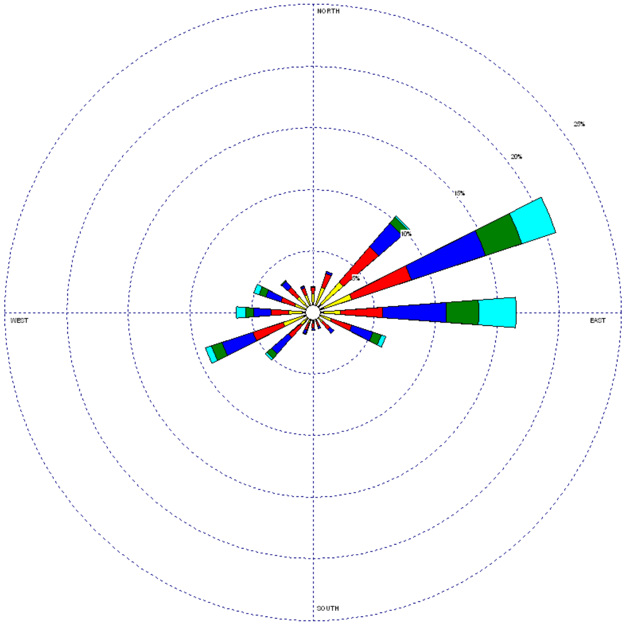
Figure 4-8 Mean Milne Point Wind Rose
