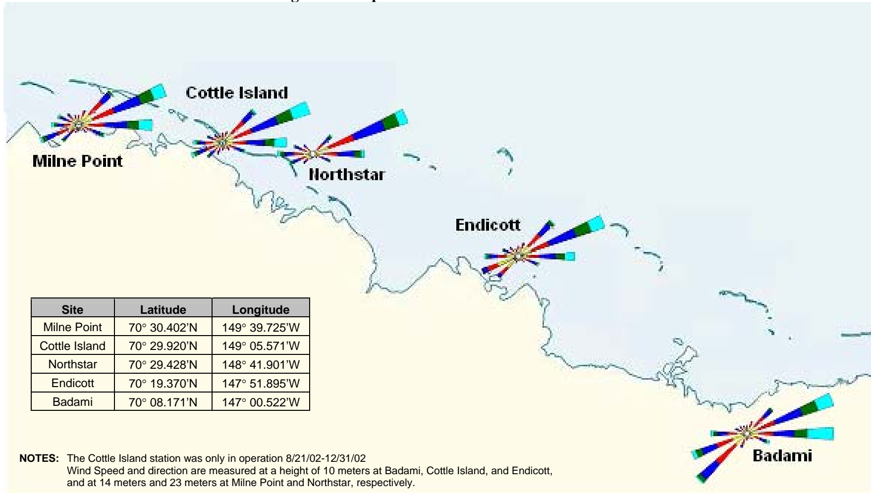
Figure 4-10 Spatial Distribution of Wind Roses
