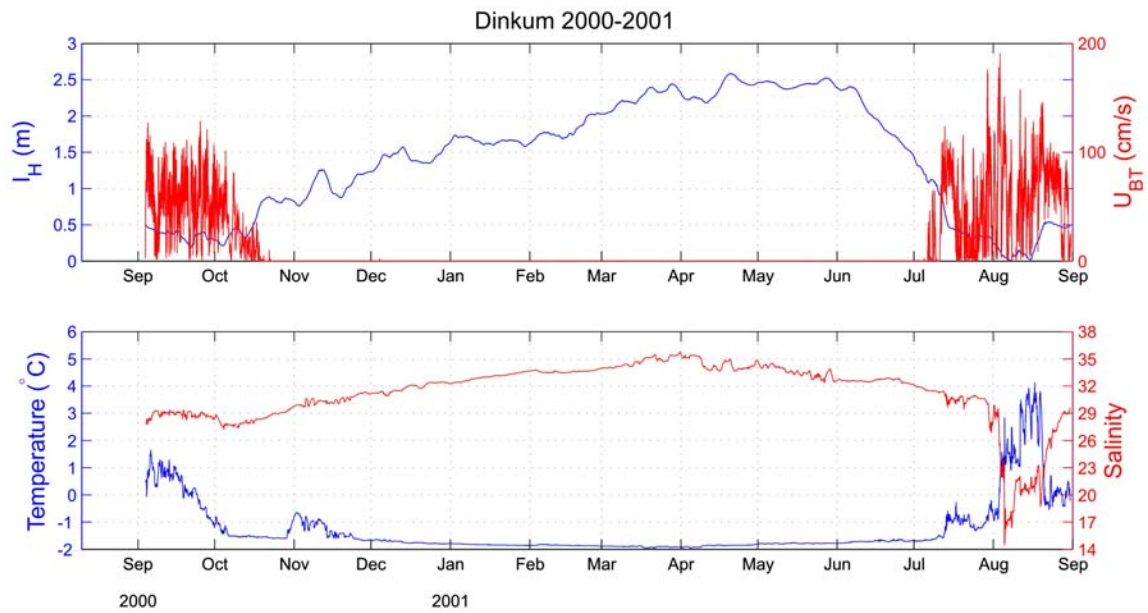
Figure 62. Ice thickness (upper panel) and temperature and salinity (lower panel) at DINKUM during the 2000 - 01 deployment.
