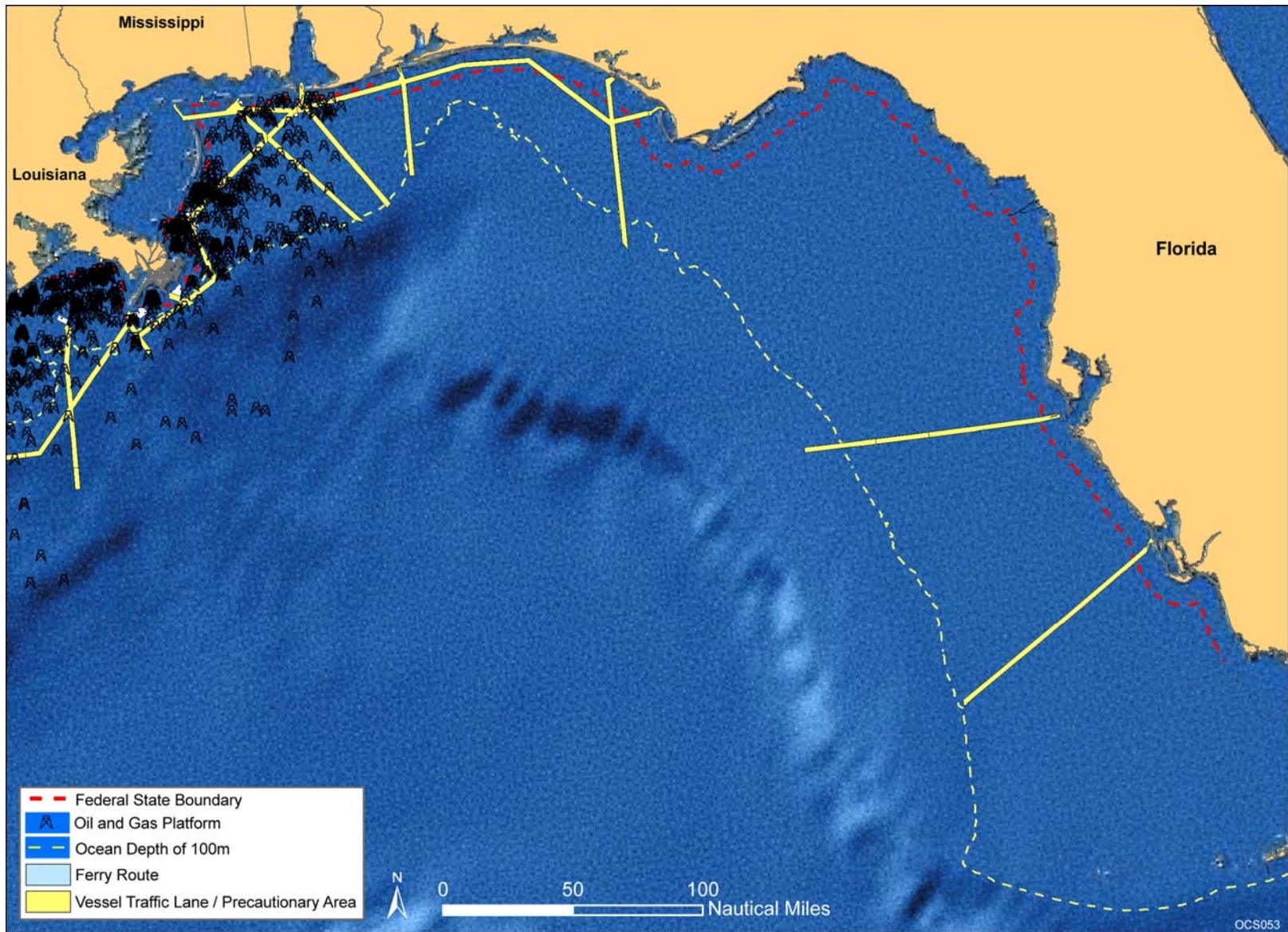
FIGURE 6.1-1 Oil and Gas Platforms in the Eastern Gulf of Mexico
