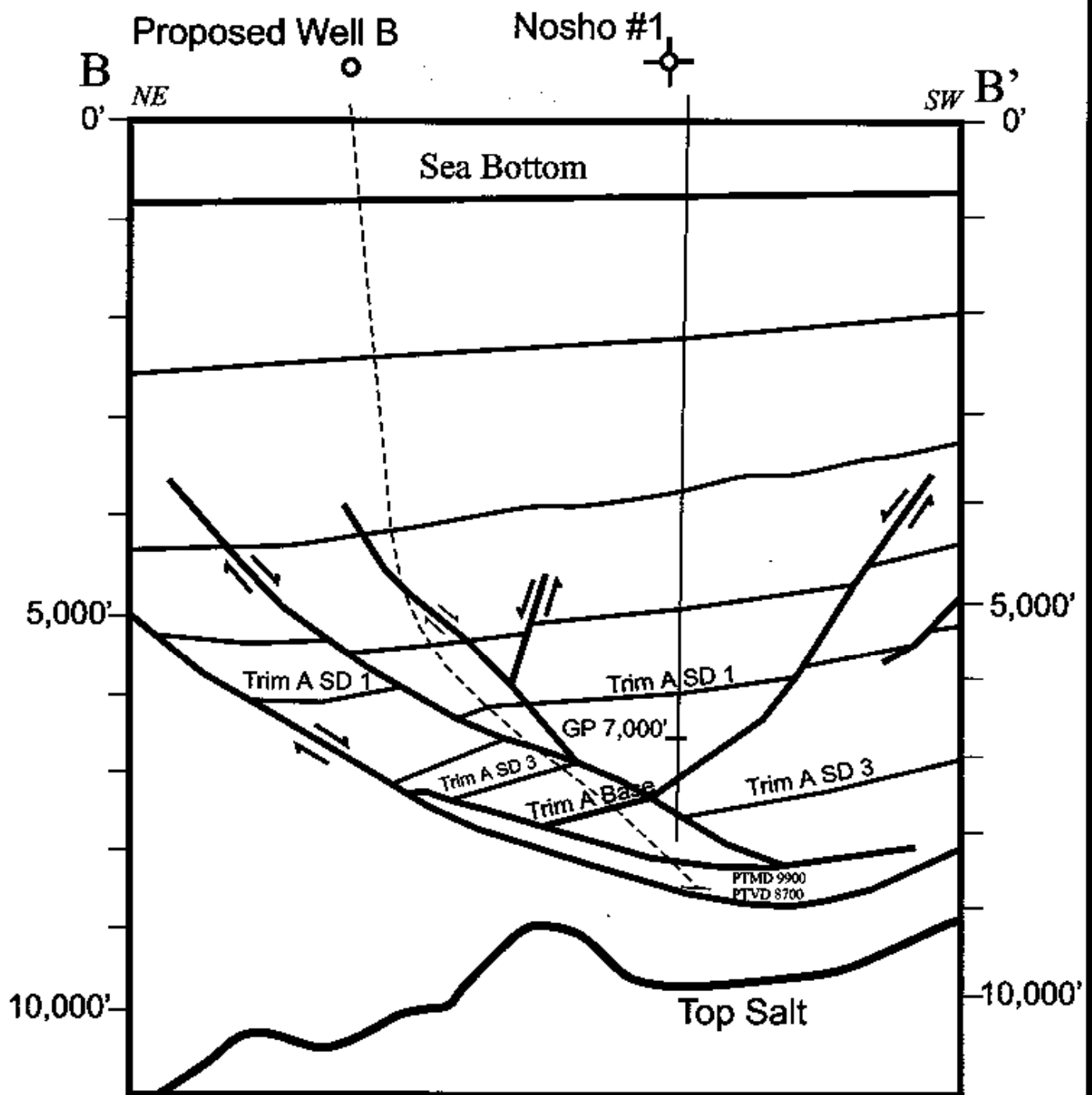
Structural Cross Section "B-B"
