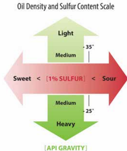
Figure 2. Oil Density and Sulfur Content Scale. Source: Bureau of Ocean Energy Management
