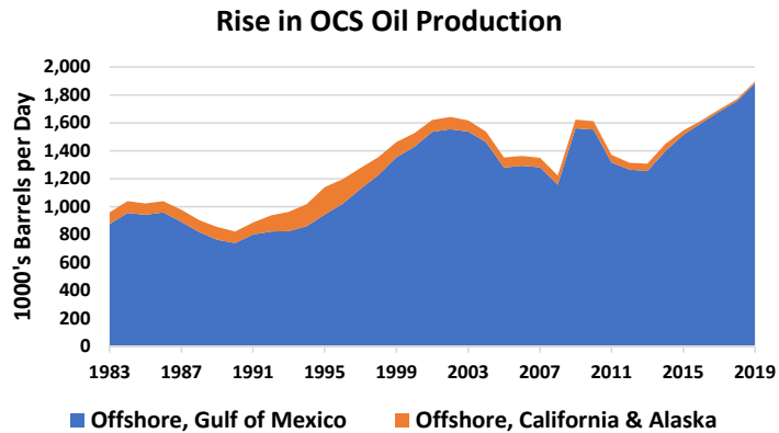
Figure 1. Rise in OCS Oil Production. Source: www.eia.gov
