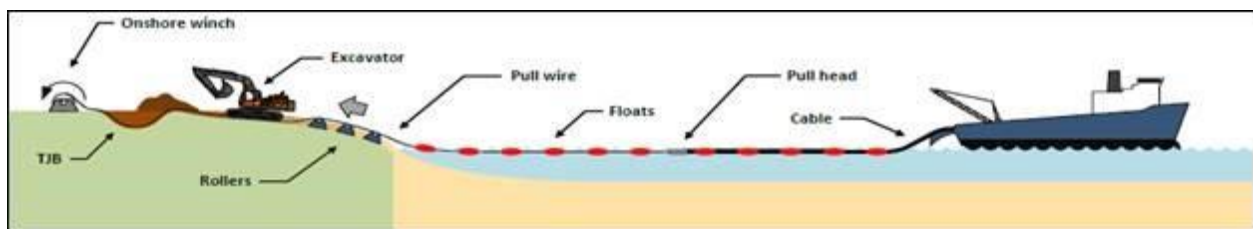
Figure 6.2.2-6. Typical open cut landfall.
