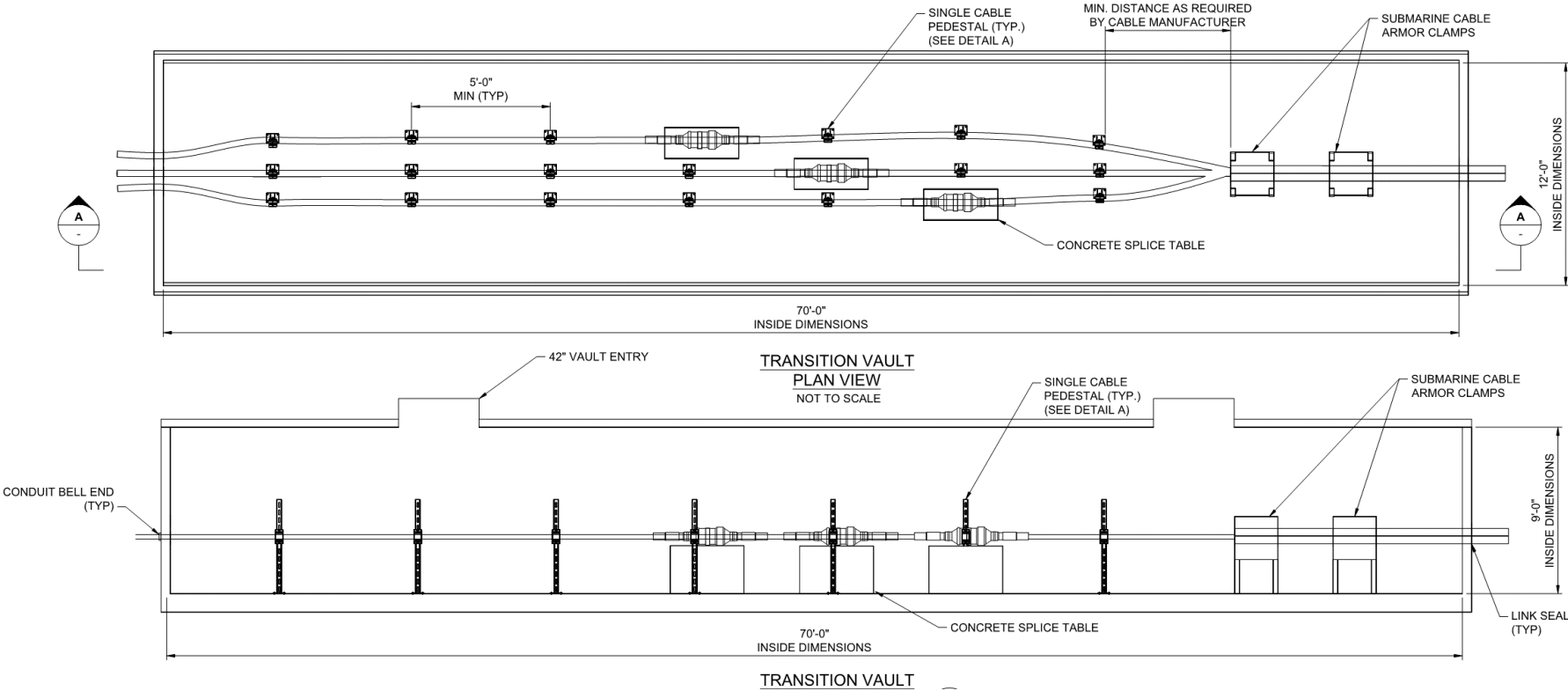
Figure 6.2.2-5. Indicative 275-kV TJB design.
