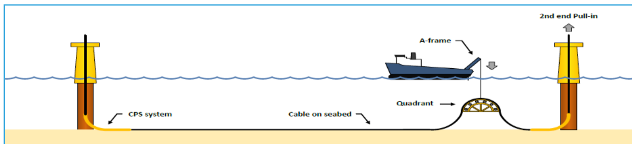
Figure 6.1.2-15. Second-end pull.
