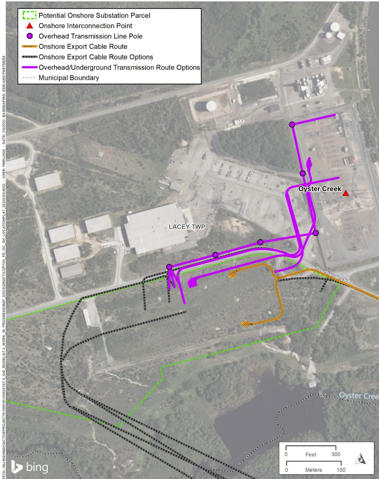
Figure 6.2.1-5. Indicative overhead transmission line/underground cable route options – Oyster Creek.
