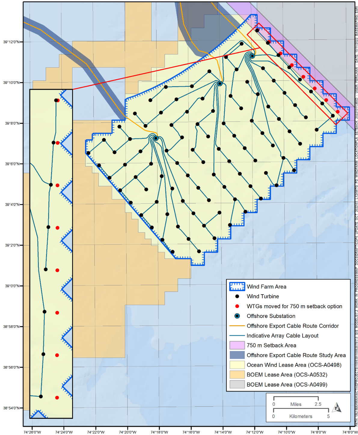
Figure 5.1-5. Indicative Location Plan - 1,500 m separation option.
