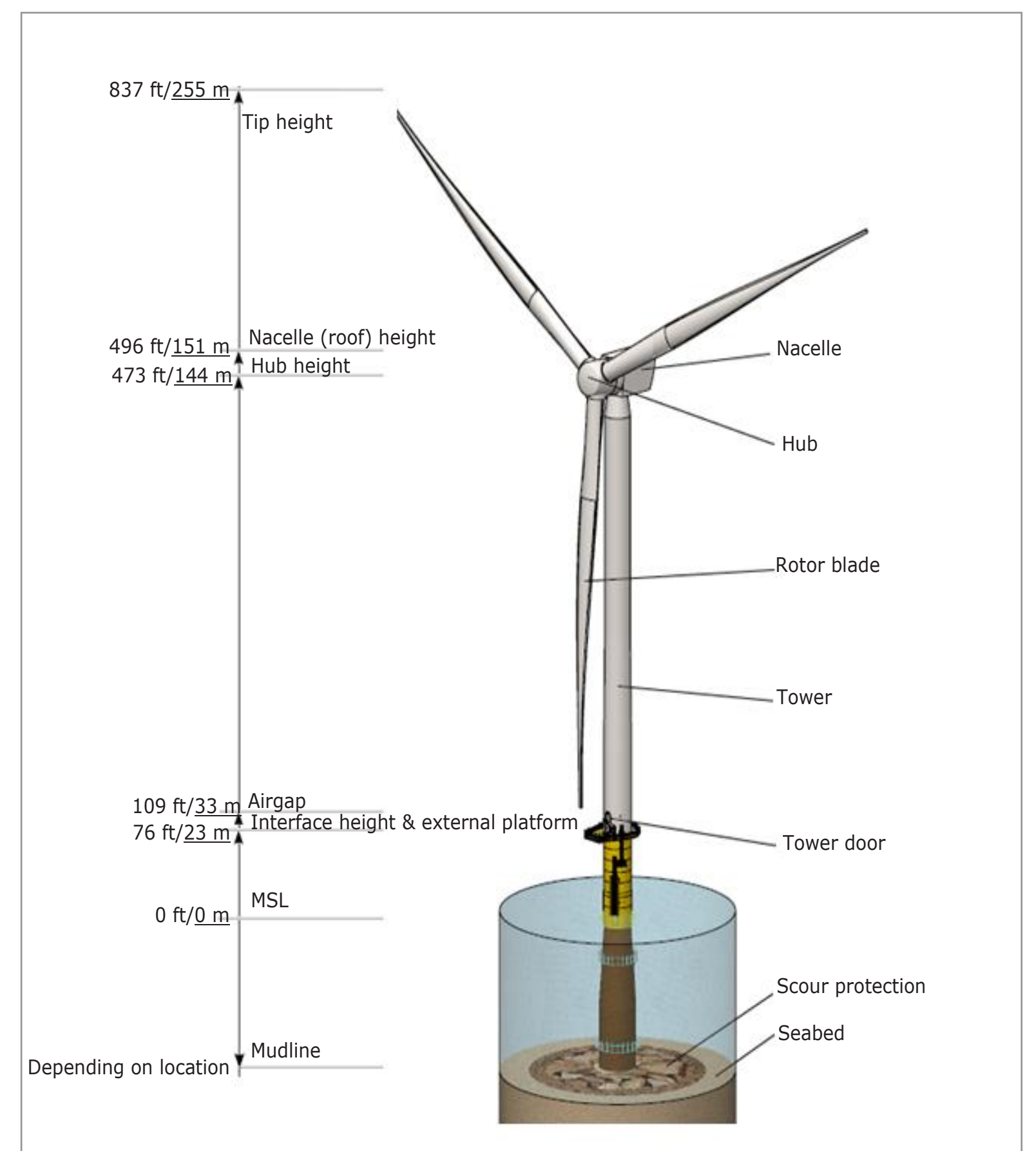
Simplified elevation drawing of the WTG: Maximum Design Wind Turbine
