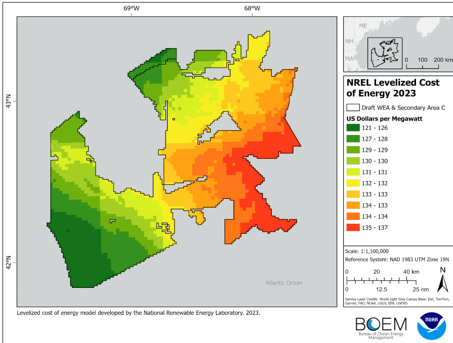
Figure 3.12. The LCOE for 2023 data layer implemented within the Wind submodel of the Final WEA suitability model. The lower the levelized cost of energy (dollars per megawatt hour), the more suitable for wind energy development.
