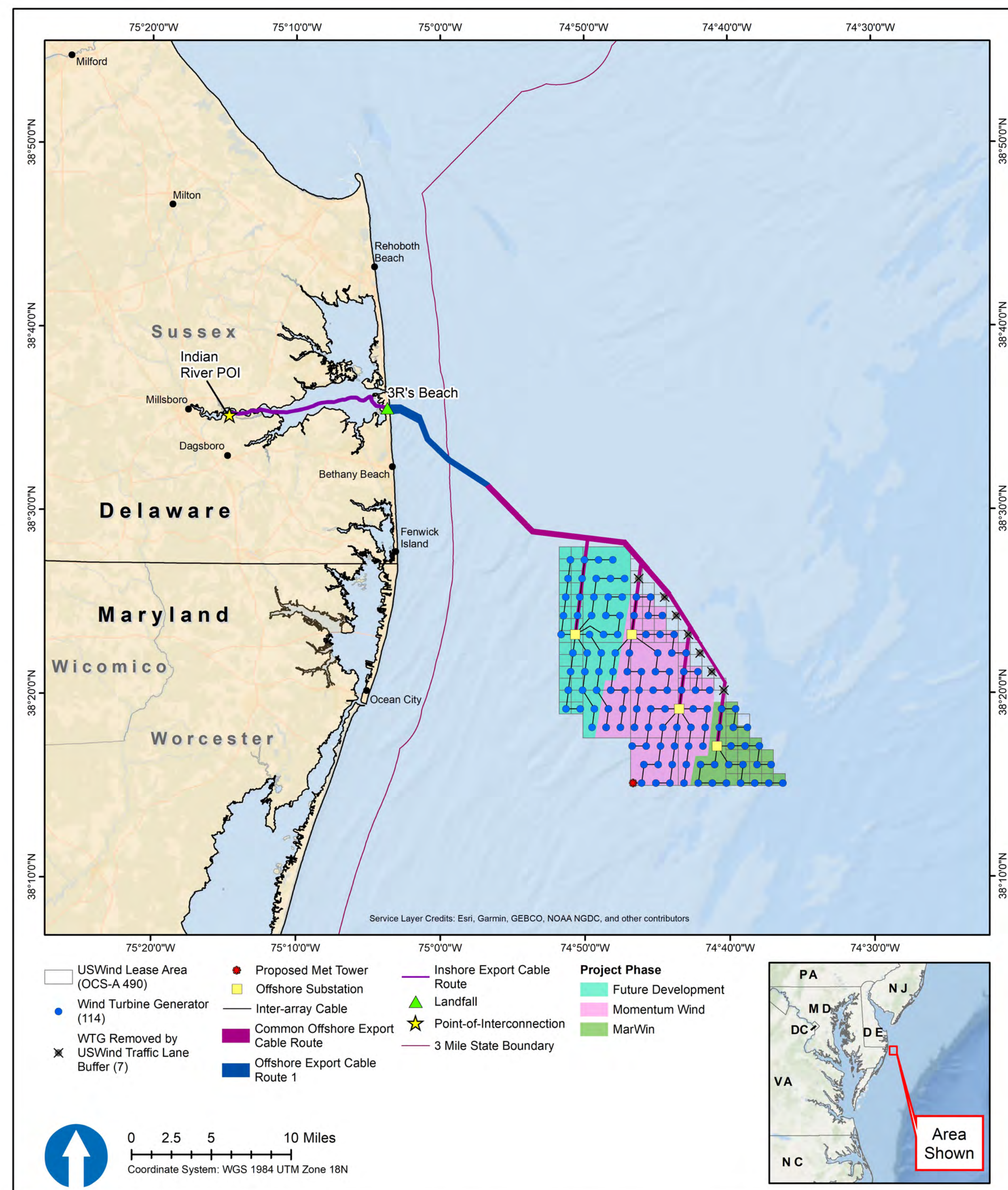
Figure 01. Project location and components under the Proposed Action (status quo).
