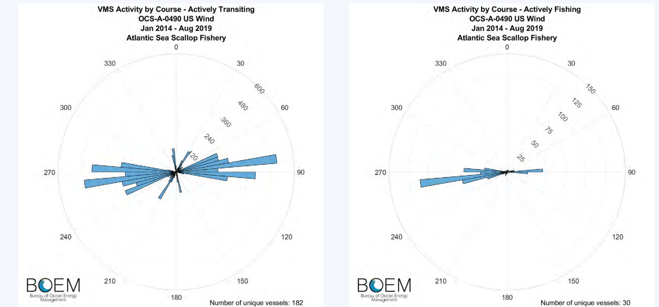
VMS Bearings for Vessels actively transiting and fishing in the Lease Area Atlantic Sea Scallop Fishery, January 2014 to August 2019
