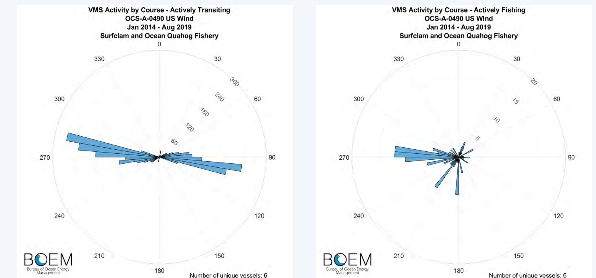
VMS Bearings for Vessels actively transiting and fishing in the Lease Area Surfclam and Ocean Quahog Fishery, January 2014 to August 2019
