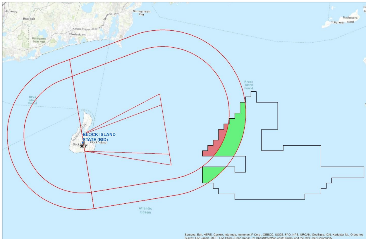
Figure 7: Block Island State (BID) VOR Approach to Runway 28 (red outline)
