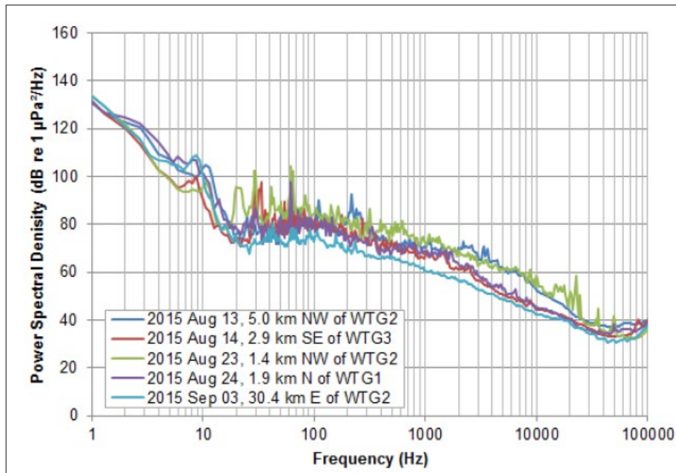
Figure 2.2-2. Power spectral density plot of ambient noise measurements collected within the vicinity of the Block Island Wind Farm. From Amaral et al. (2018). WTG = wind turbine generator
