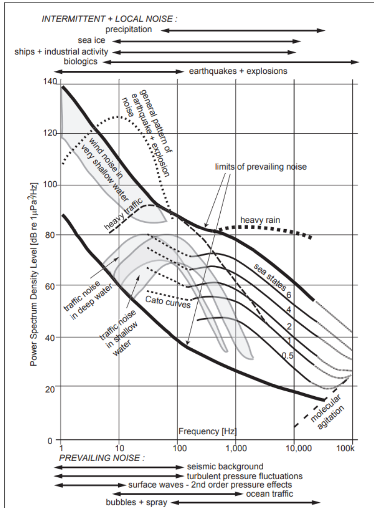
Figure 2.1-1. Wenz curve showing frequency and amplitude range of common sources of noise in the ocean. Figure from Erbe (2011) based on work from Wenz (1962).
