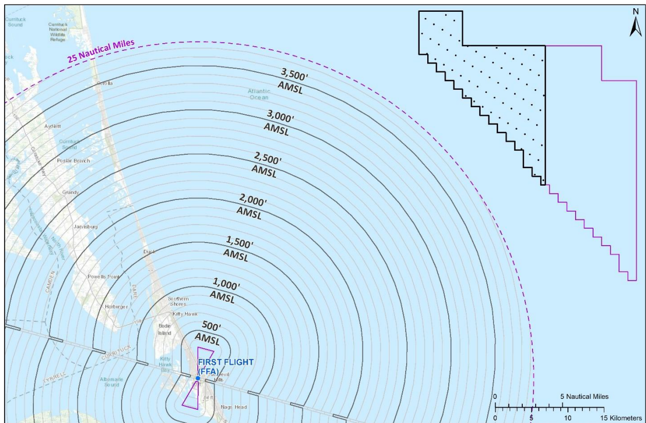
Figure 6: First Flight (FFA) obstacle departure procedure assessment
