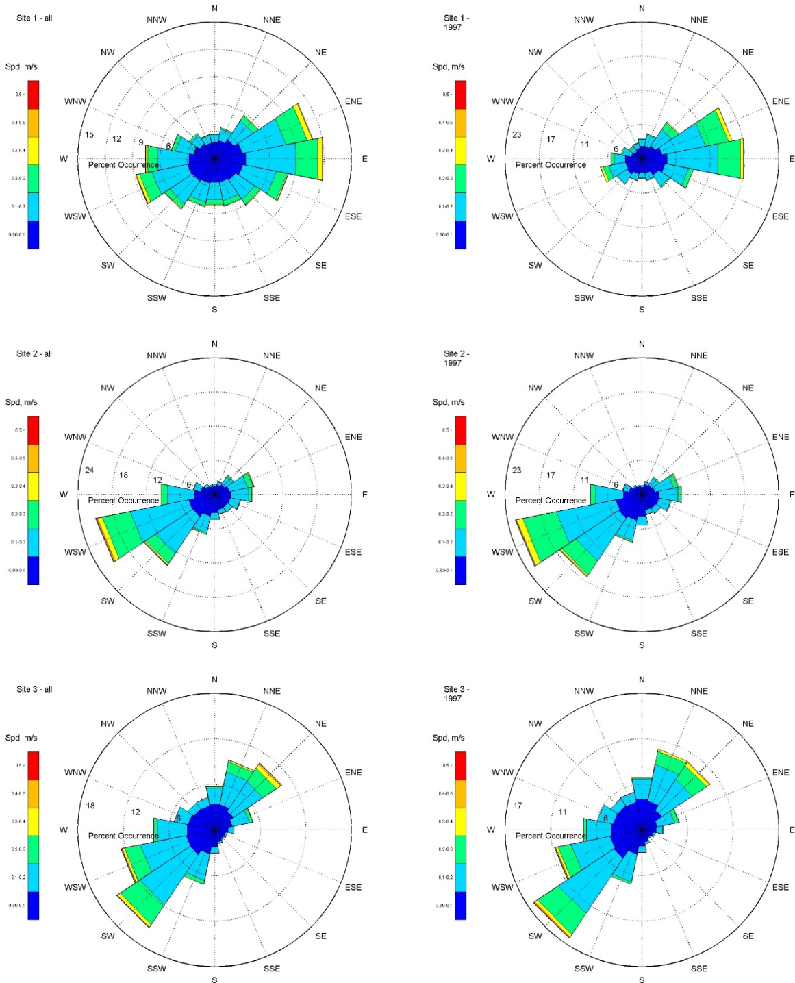
Figure 6.1-2 Current wind rose comparisons between 39-year dataset (left) and the representative year 1997 (right) at sites 1 (top), 2 (middle), and 3 (bottom).
