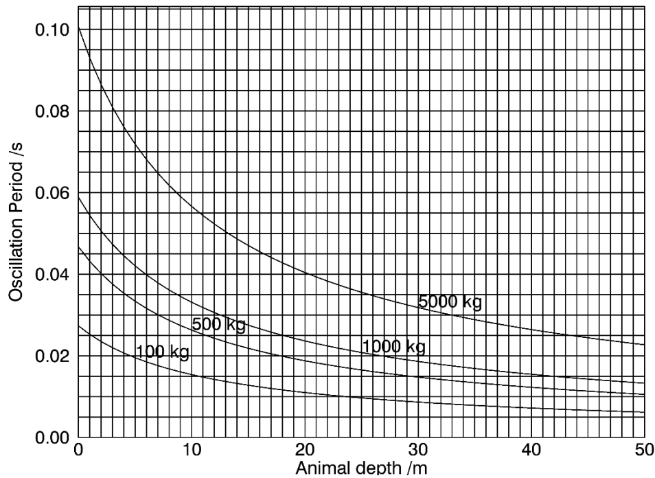
Figure 5. Lung oscillation periods for animal masses of 100, 500, 1000, and 5000 kg versus submersion depth, calculated using equation 10.
