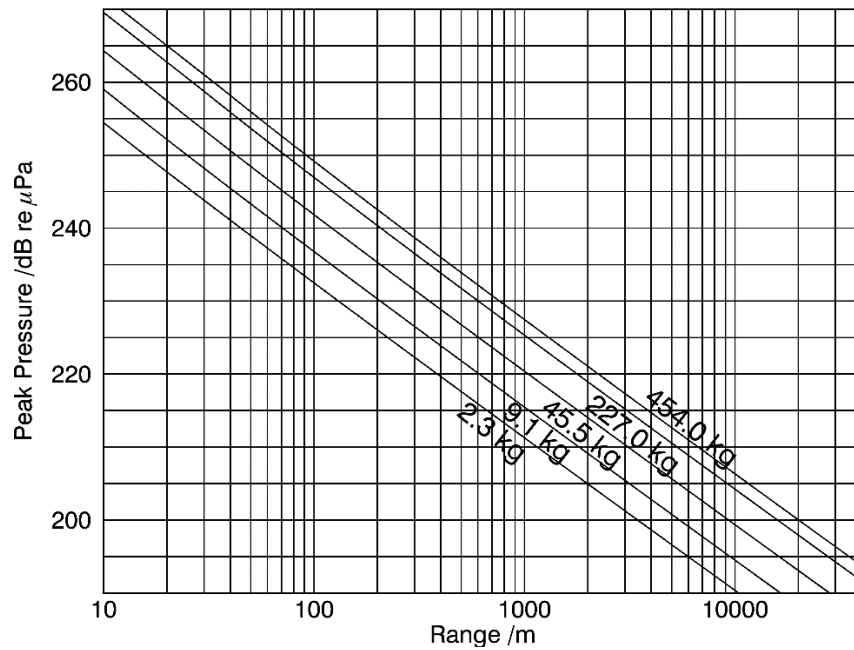
Figure 3. Peak pressures versus distance from detonations of the charge weights listed in Table 1, calculated with equations 2 and 4.
