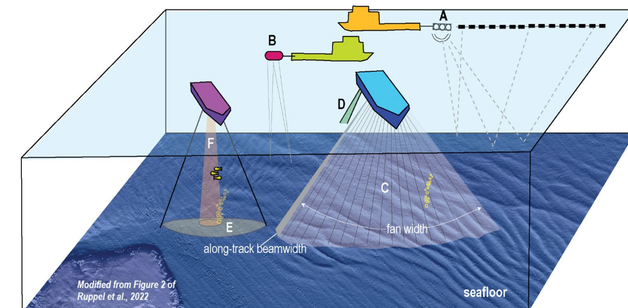
Modified from Figure 2 of Ruppel et al., 2022 Schematic diagram showing common high-resolution geophysical (HRG) sources. High-Resolution Geophysical surveys (HRG surveys) Airgun arrays are not shown because this type of survey equipment is not used for offshore wind surveys.
