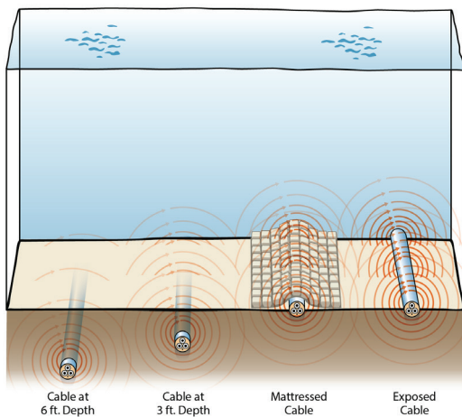
Burying cables reduces EMF
