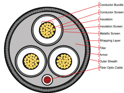
Cable cross-section
