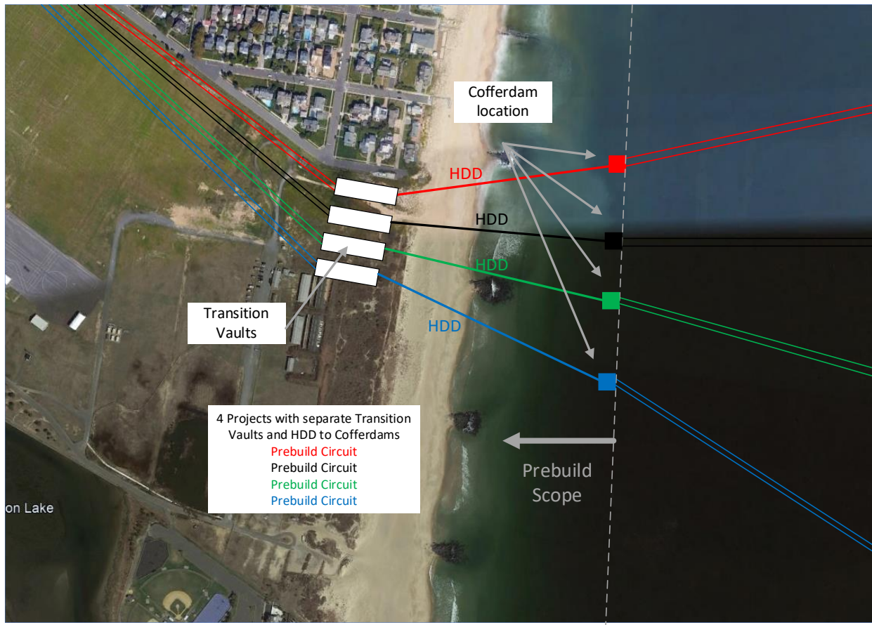
Figure B.10-2. Illustrative example of circuit arrangement at landfall
