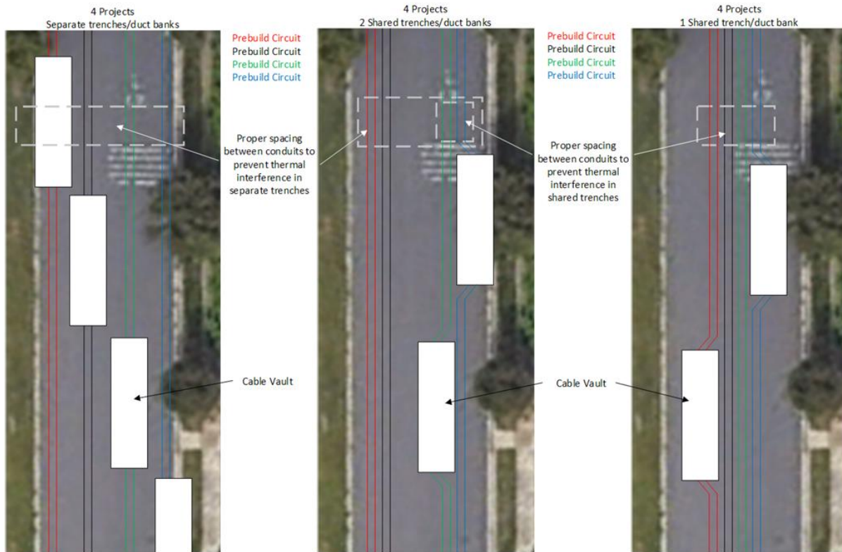
Figure B.10-1. Illustrative example of duct bank and cable vault layout
