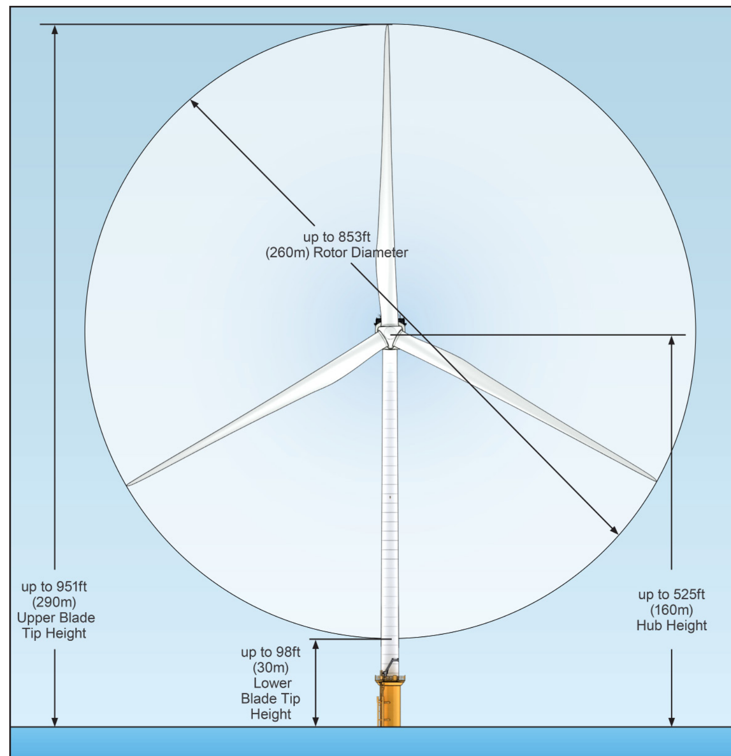
Representative Wind Turbine
