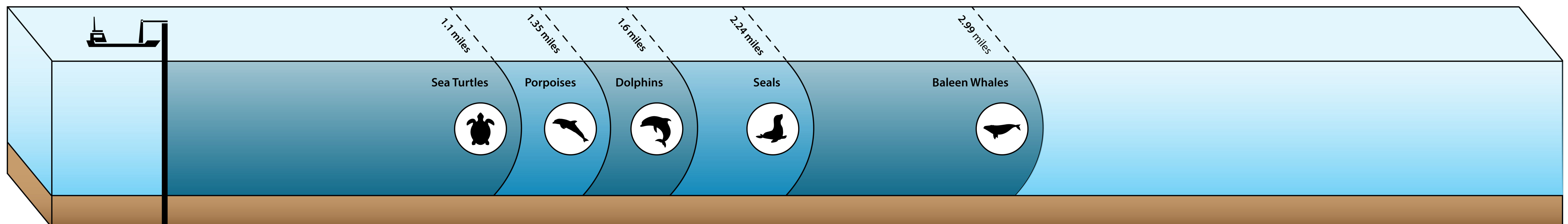
Maximum distance for behavioral impacts for difficult installation of an 11-meter monopile using an IHC S-4000 impact hammer with 10-dB attenuation
