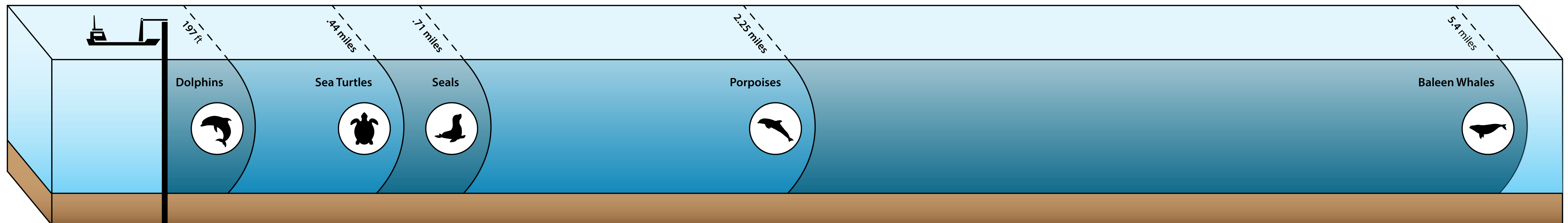
Maximum distance for underwater hearing impacts for difficult installation of an 11-meter monopile using an IHC S-4000 impact hammer with 10-dB attenuation
