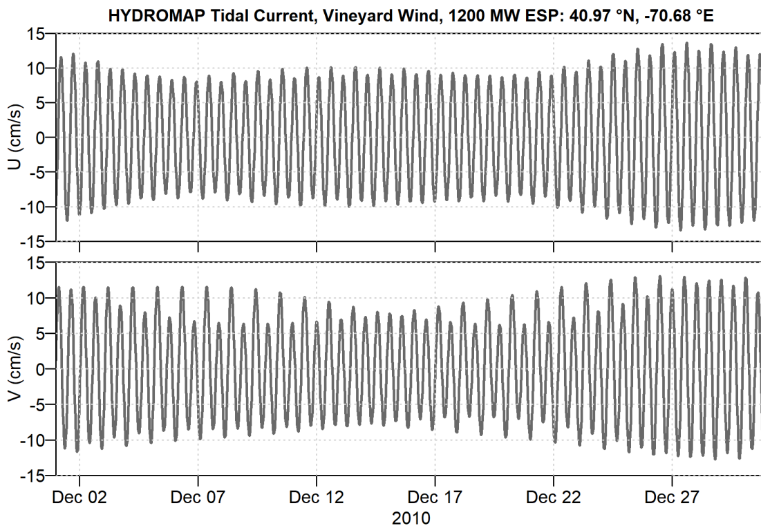
Figure 9. Example of timeseries of U and V component of tidal current (from HYDROMAP) near the 1,200 MW ESP.
