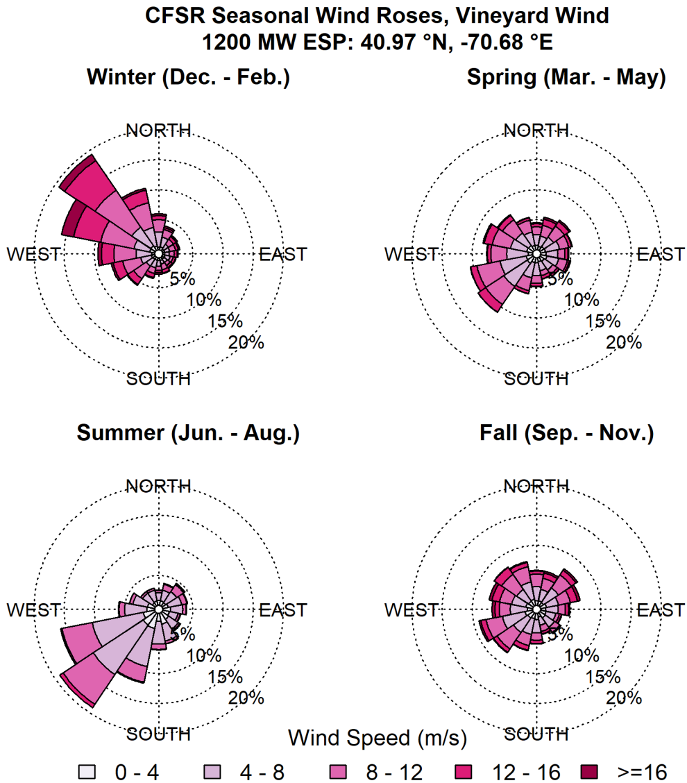
Figure 8. Seasonal CFSR windroses near the 1,200 MW ESP. Wind speeds in m/s, using meteorological convention (i.e. direction wind is coming from).
