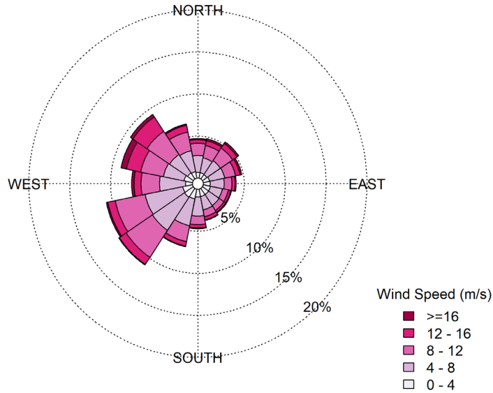
Figure 5. Annual CFSR windrose near the 1,200 MW ESP. Wind speeds in m/s, using meteorological convention (i.e. direction wind is coming from).
