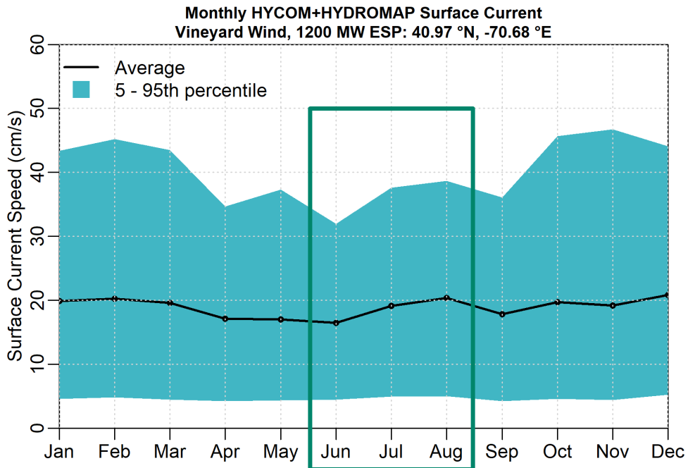
Figure 12. Monthly average (black line) and 5th to 95th percentile (blue polygon) HYCOM+HYDROMAP current speed (cm/s) statistics near the spill site. The green box highlights summer.
