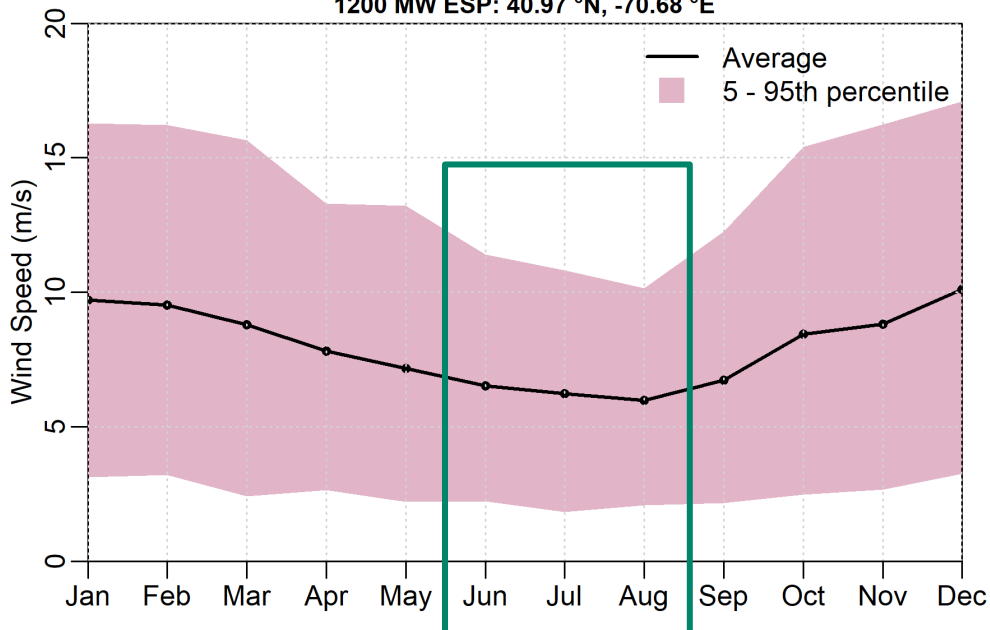
Figure 6. Monthly average (black) and 5 th to 95 th percentile (pink polygon) CFSR wind speed statistics near the 1,200 MW ESP. Wind speed is reported in m/s. The green box highlights summer.
