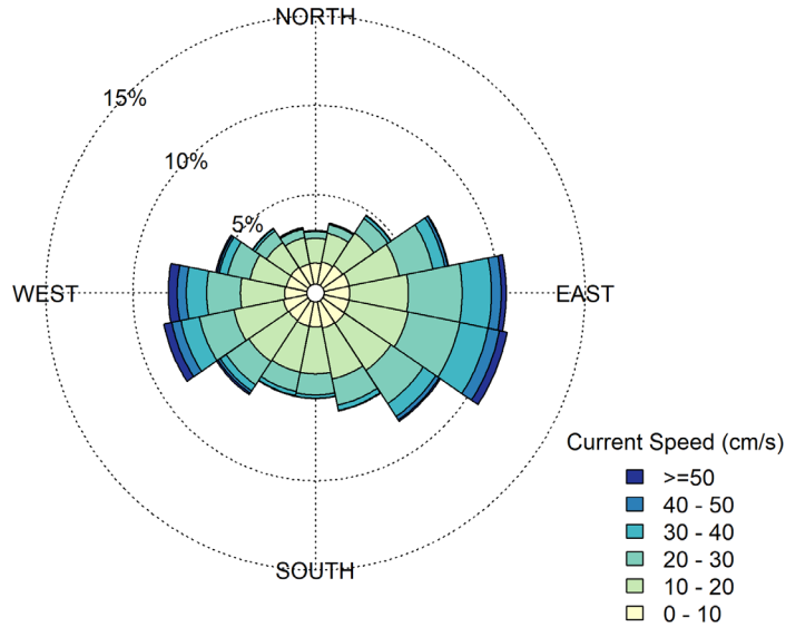
Figure 11. Annual HYCOM+HYDROMAP surface current rose near spill site following oceanographic convention (direction currents are heading towards). Current speeds are in cm/s.
