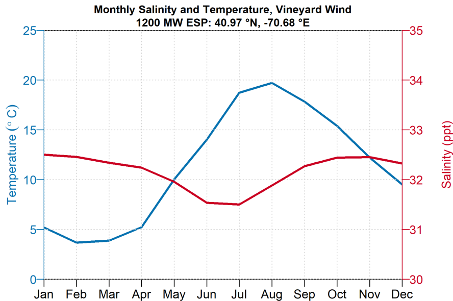
Figure 3. Monthly sea surface temperature (°C) in blue and sea surface salinity (ppt) in red near the 1,200 MW ESP (Locarnini et al. 2018; Zweng et al. 2018).
