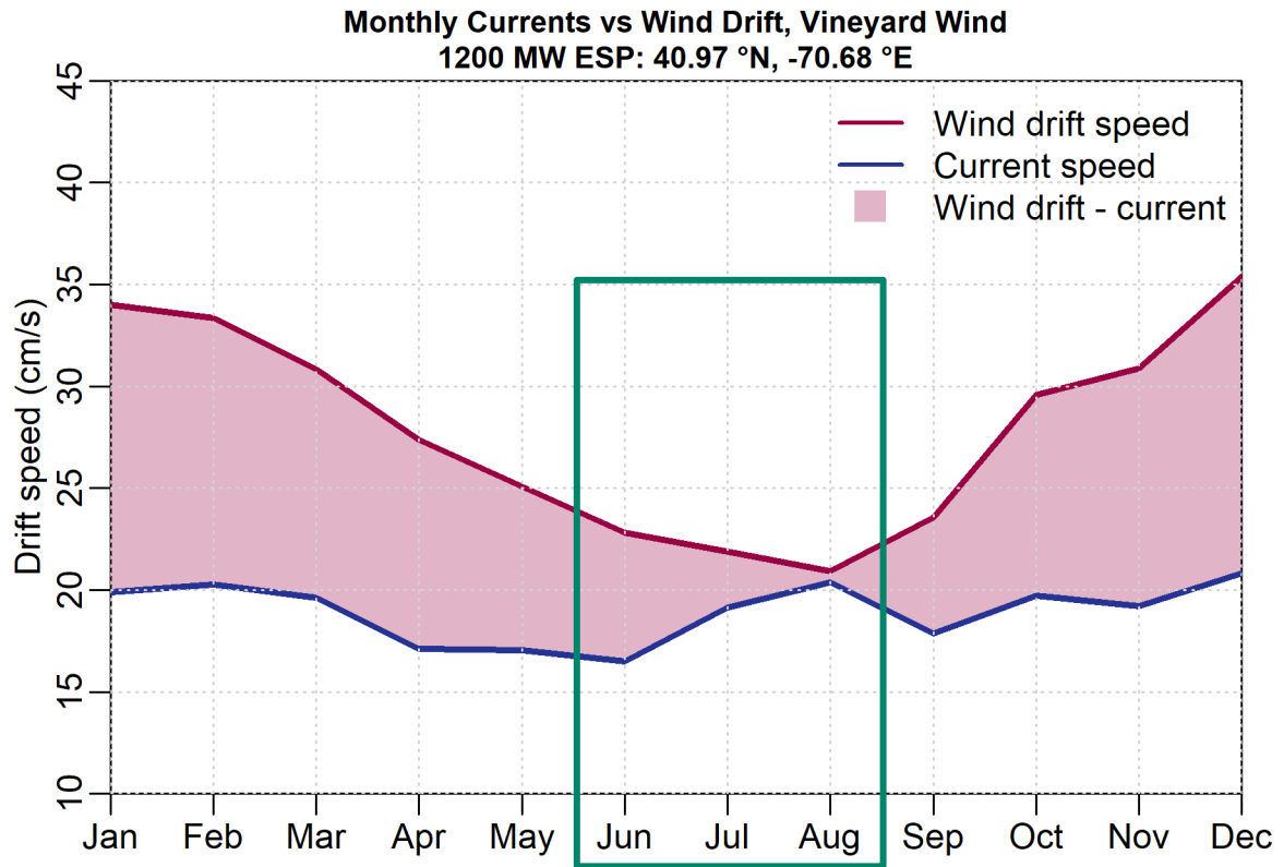
Figure 15. Surface drift forcing comparison statistics near the Vineyard Wind spill site: monthly-averaged CSFR wind drift compared with HYCOM+HYDROMAP current speed. Wind drift is calculated as 3.5% of the wind speed. Periods with predominant wind transport are shaded pink. The green box highlights summer.
