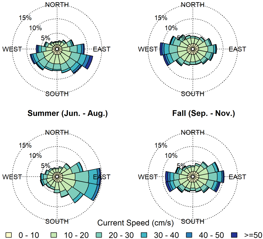
Figure 14. Seasonal HYCOM+HYDROMAP current roses near the 1,200 MW ESP. Current speeds in cm/s, using oceanographic convention (direction currents are heading towards).
