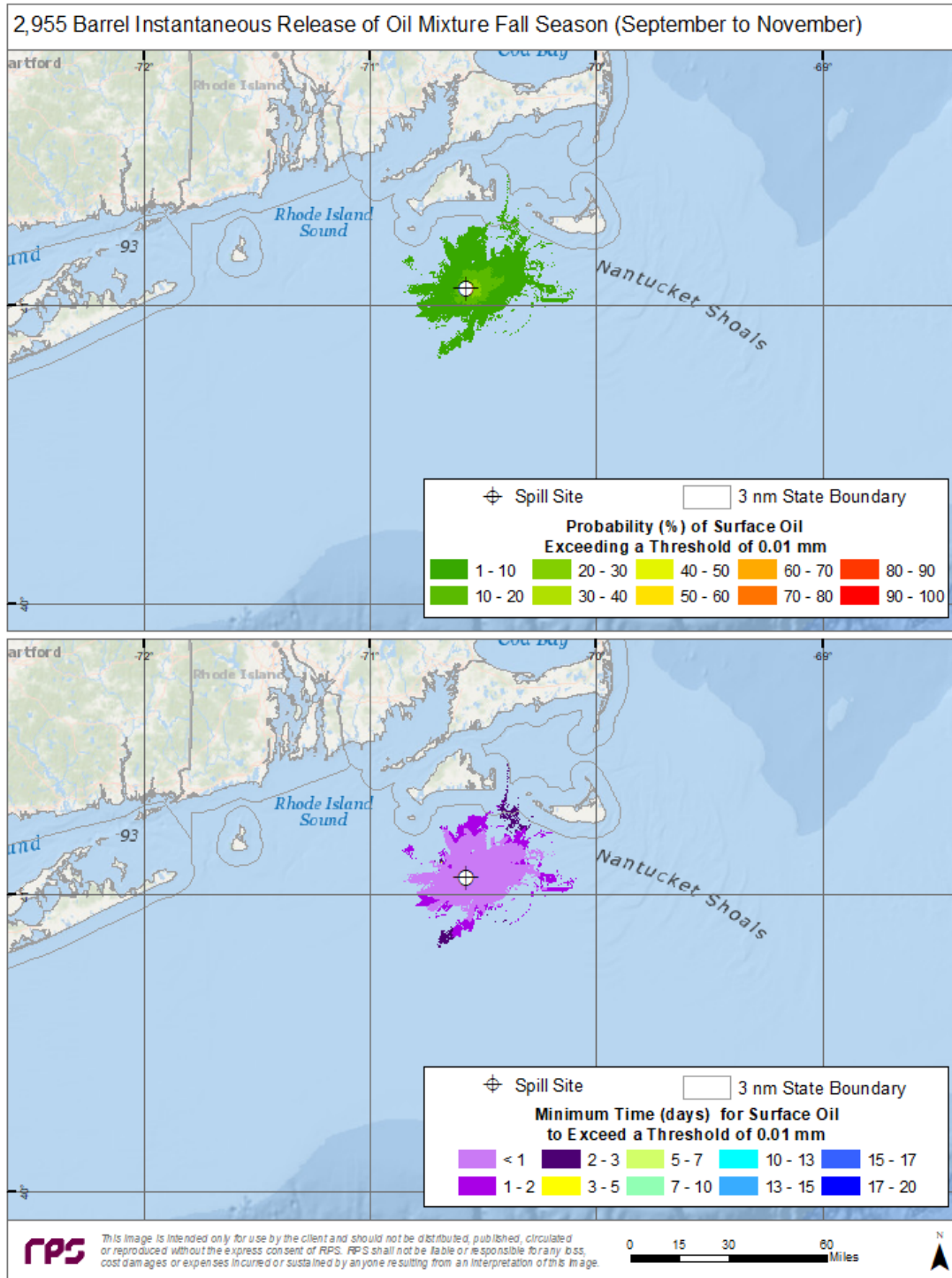
Figure 23. Detail View. Top Panel—Probability of surface oiling above a minimum thickness of 10 \mu\text{m} (10 \text{g}/\text{m}^2 on average over the grid cell) during fall months for an instantaneous release from the 800 MW Phase 1 ESP location. Bottom Panel—Minimum time for surface oiling to occur at thicknesses greater than 10 \text{g}/\text{m}^2 .
