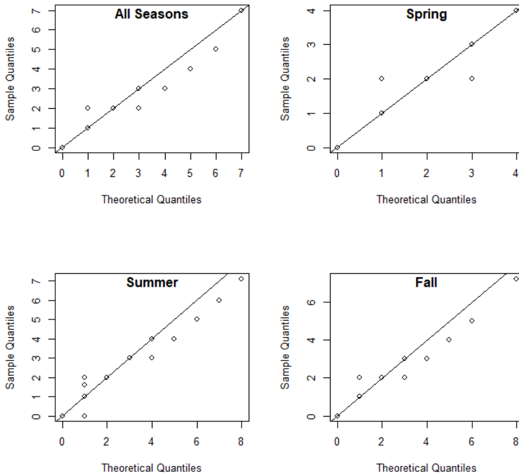
Figure C-5. Quantile-Quantile plots of negative binomial distributions fit to NJDEP fish pot Jonah crab catch data.
