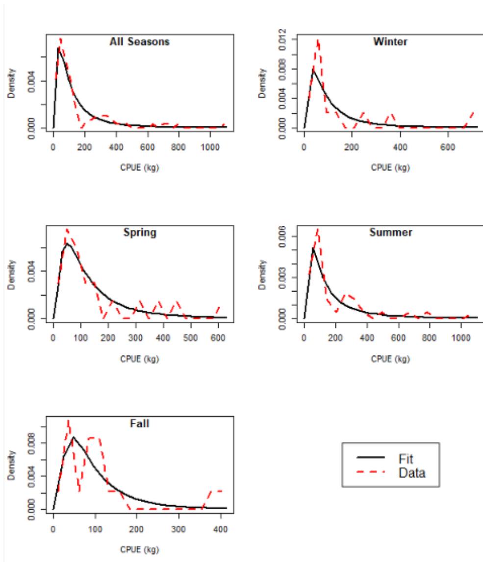
Figure B-4. Lognormal distribution (black) fitted to all-species biomass CPUE from NJDEP trawl data (red, dashed) collected within the Lease Area and Lease Area OCS-A 0499 between 2009 and 2019. The fitted distributions from each season were used to generate datasets for the CPUE power analysis simulation.
