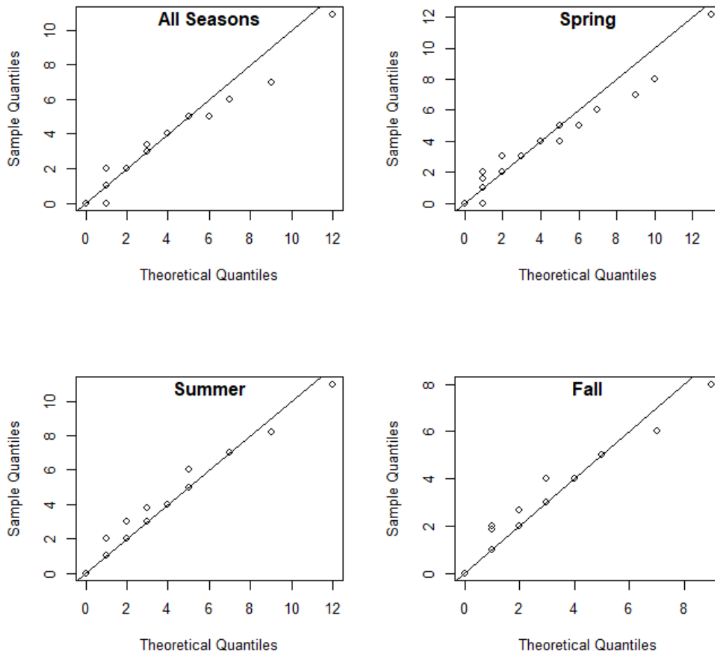
Figure C-3. Quantile-Quantile plots of negative binomial distributions fit to NJDEP fish pot rock crab catch data.
