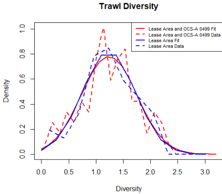
Figure B-5. Normal distributions (solid) fitted to diversity values from NJDEP trawl data (dashed) collected within the Lease Area and Lease Area OCS-A 0499 (red) and just the Lease Area (blue) between 2009 and 2021.
