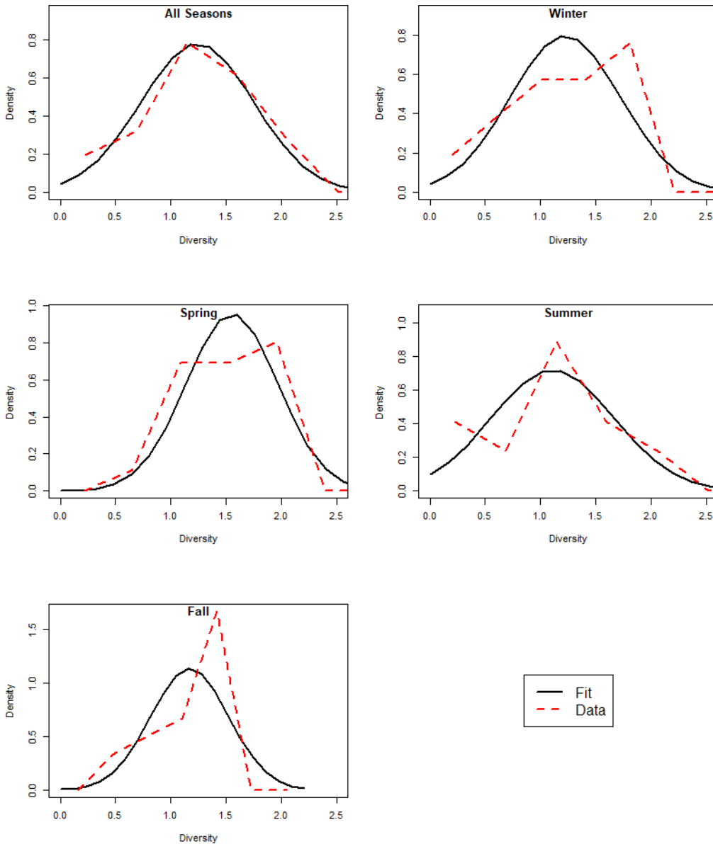
Figure B-3. Normal distribution (black) fitted to H' Diversity from NJDEP trawl data (red, dashed) collected within the Lease Area and Lease Area OCS-A 0499 between 2009 and 2021. Fitted distributions for each season were used to generate datasets for the diversity power analysis simulation.
