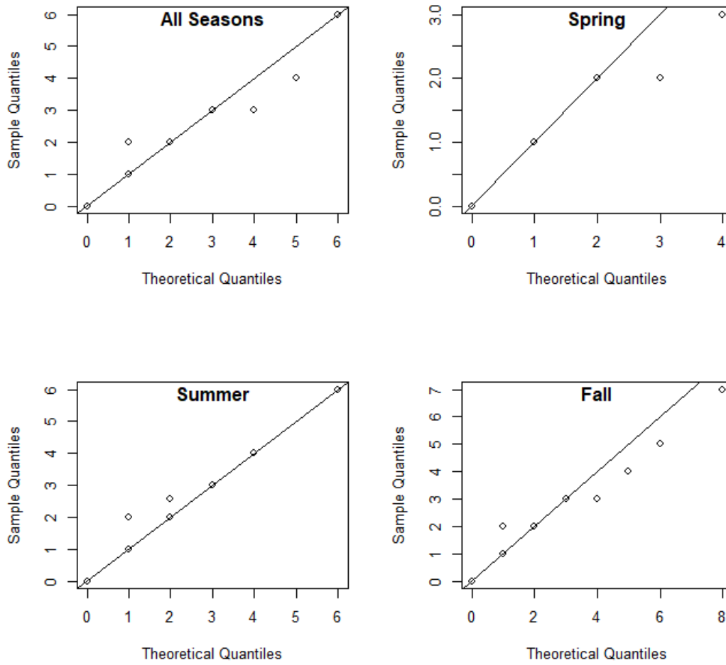
Figure C-7. Quantile-Quantile plots of negative binomial distributions fit to NJDEP fish pot tautog catch data.
