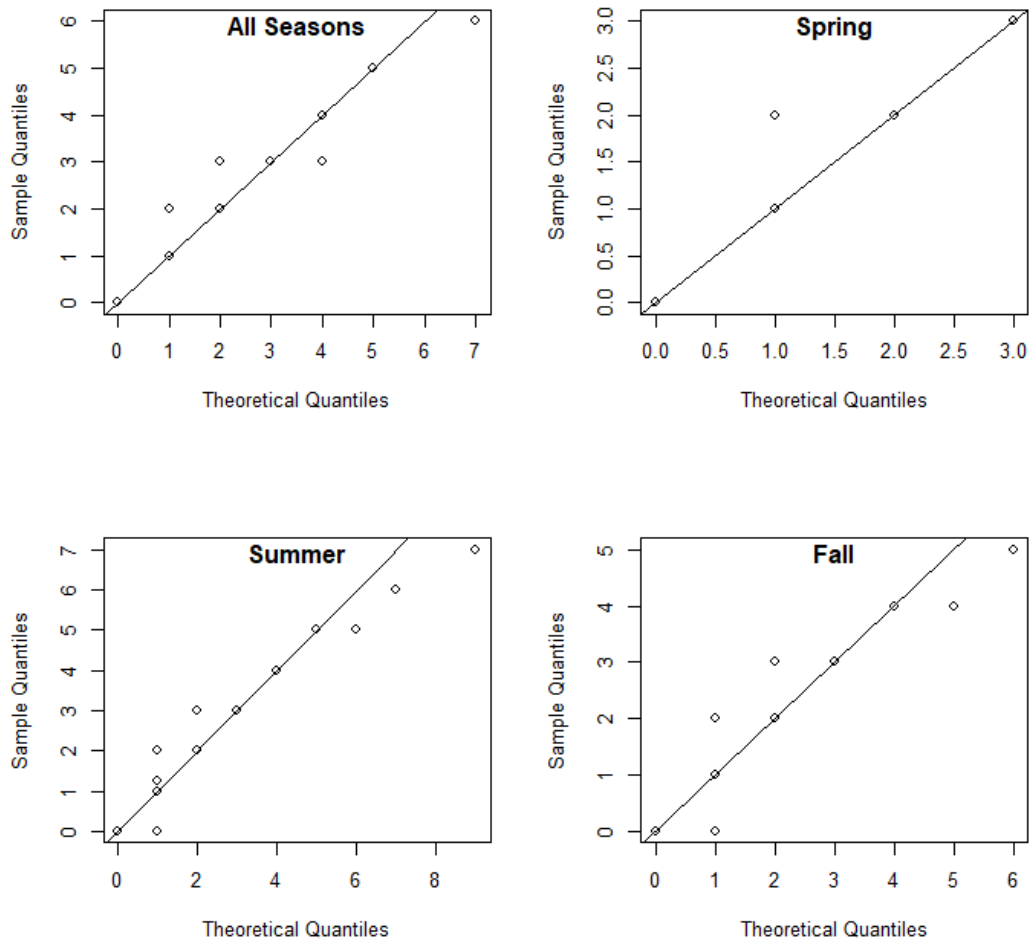
Figure C-6. Quantile-Quantile plots of negative binomial distributions fit to NJDEP fish pot lobster catch data.
