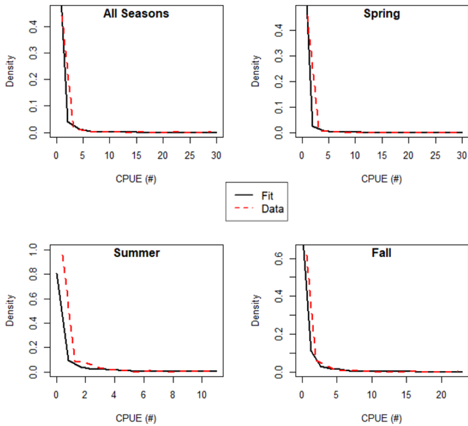
Figure B-8. Negative binomial distribution (black) fitted to tautog abundance CPUE from NJDEP trap data (red, dashed) collected around artificial reefs along the New Jersey coast between 2016 and 2021. The fitted distributions from each season were used to generate datasets for the CPUE power analysis simulation.
