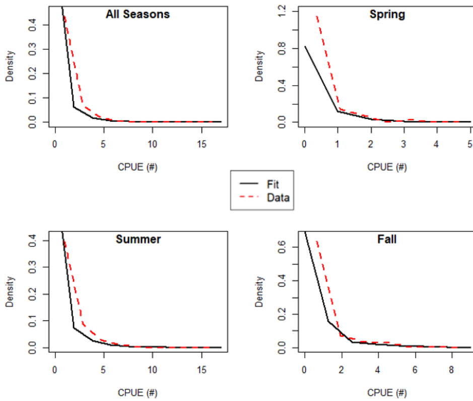
Figure B-9. Negative binomial distribution (black) fitted to lobster abundance CPUE from NJDEP trap data (red, dashed) collected around artificial reefs along the New Jersey coast between 2016 and 2021. The fitted distributions from each season were used to generate datasets for the CPUE power analysis simulation.
