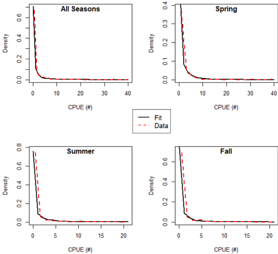
Figure B-10. Negative binomial distribution (black) fitted to rock crab abundance CPUE from NJDEP trap data (red, dashed) collected around artificial reefs along the New Jersey coast between 2016 and 2021. The fitted distributions from each season were used to generate datasets for the CPUE power analysis simulation.
