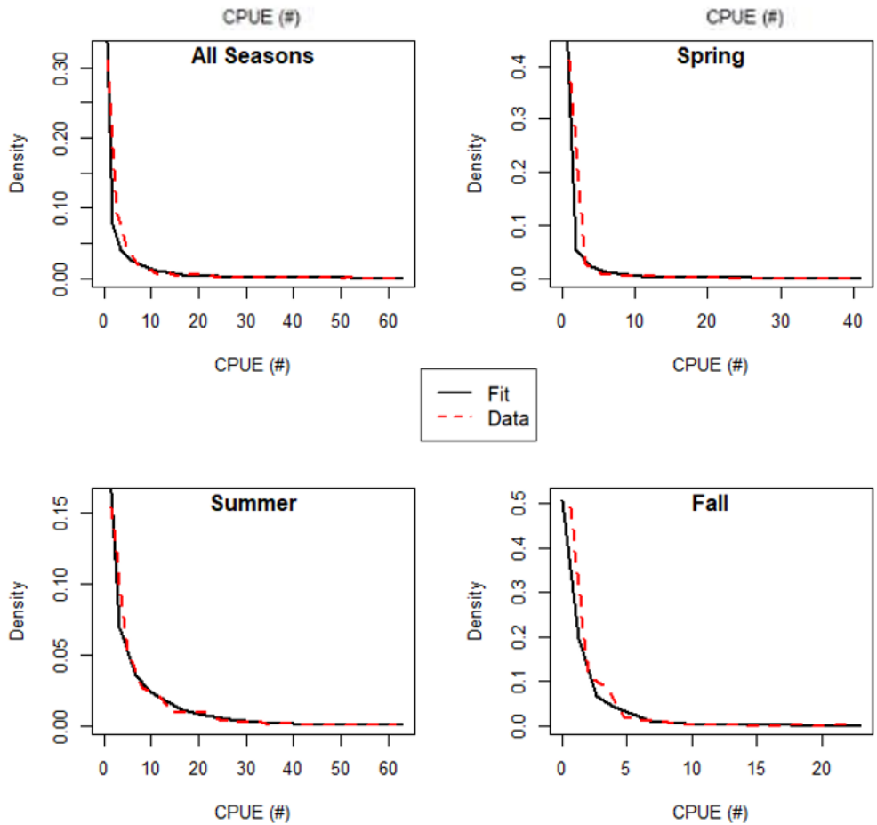
Figure B-7. Negative binomial distribution (black) fitted to black sea bass abundance CPUE from NJDEP trap data (red, dashed) collected around artificial reefs along the New Jersey coast between 2016 and 2021. The fitted distributions from each season were used to generate datasets for the CPUE power analysis simulation.
