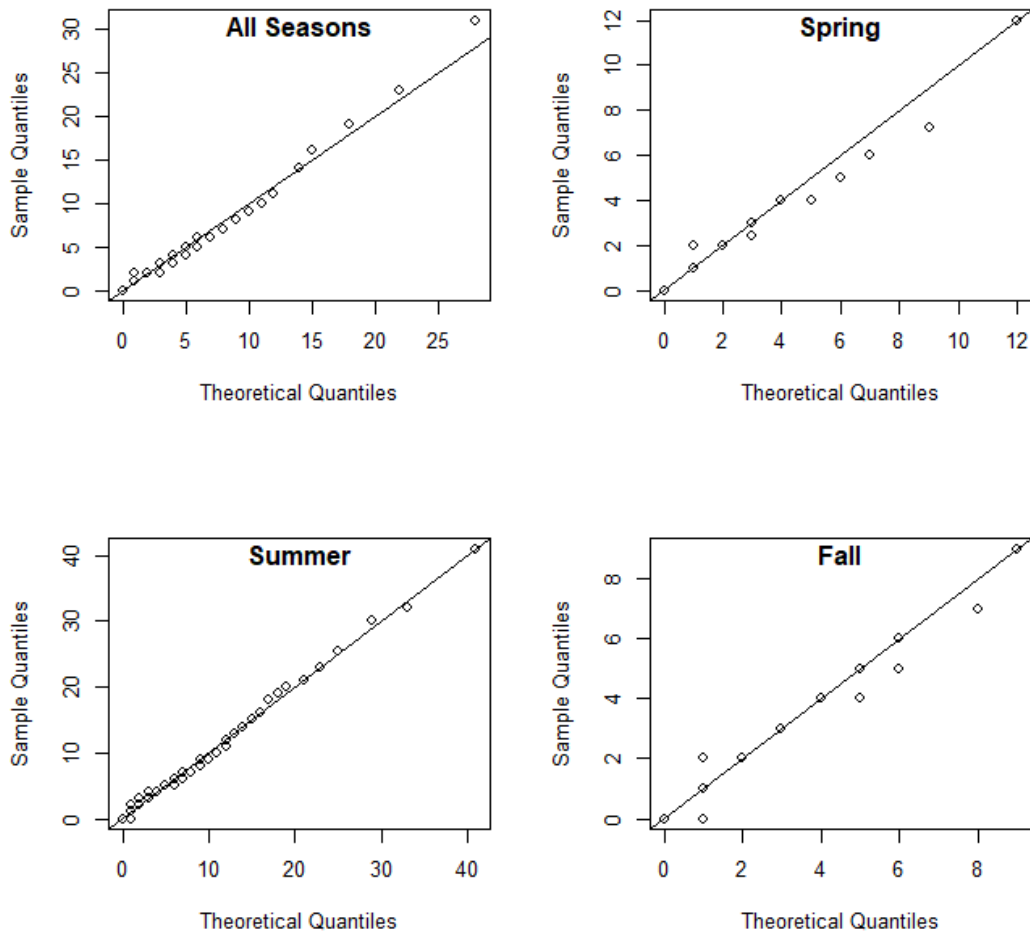
Figure C-4. Quantile-Quantile plots of negative binomial distributions fit to NJDEP fish pot black sea bass catch data.
