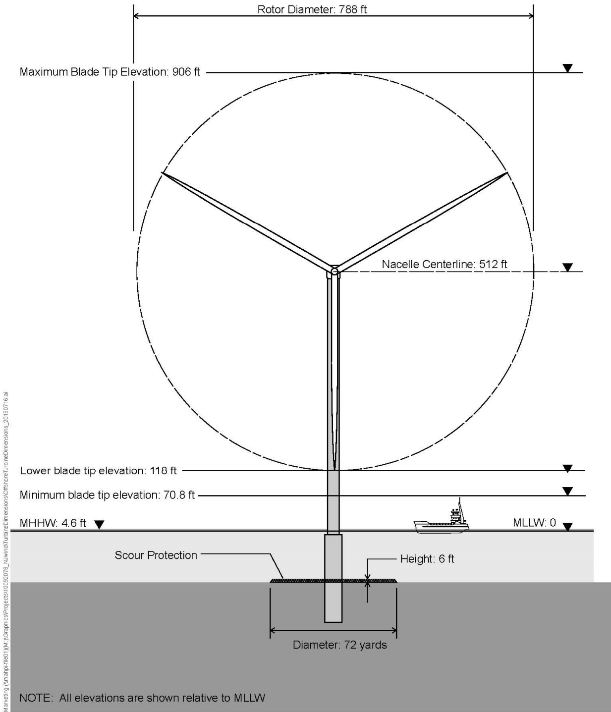
Figure 1-2. Maximum design scenario for wind turbines.
