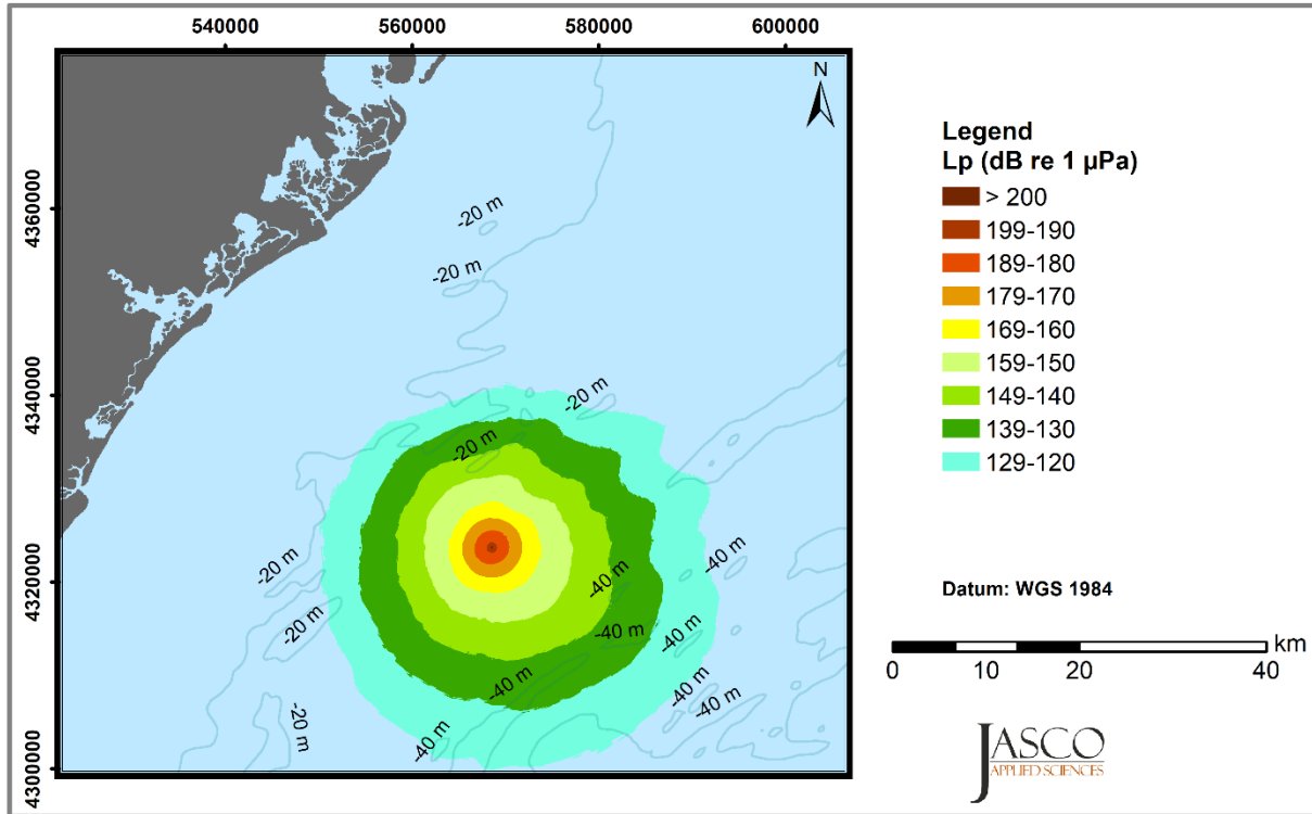
Figure H-3. Unweighted single-strike sound pressure level (SPL) at 4000 kJ at 50 m penetration depth. This sound field was produced by the highest energy for the monopile installation in summer conditions.
