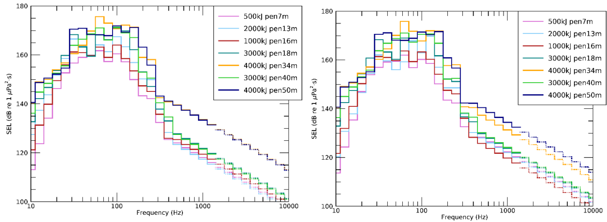
Figure 9. Location G10: Deciddecade band spectral levels at 750 m for an 8/11 m diameter monopile assuming an expected installation scenario using an IHC S-4000 kJ hammer with an average summer sound speed profile (left panel) and winter sound speed profile (right panel).
