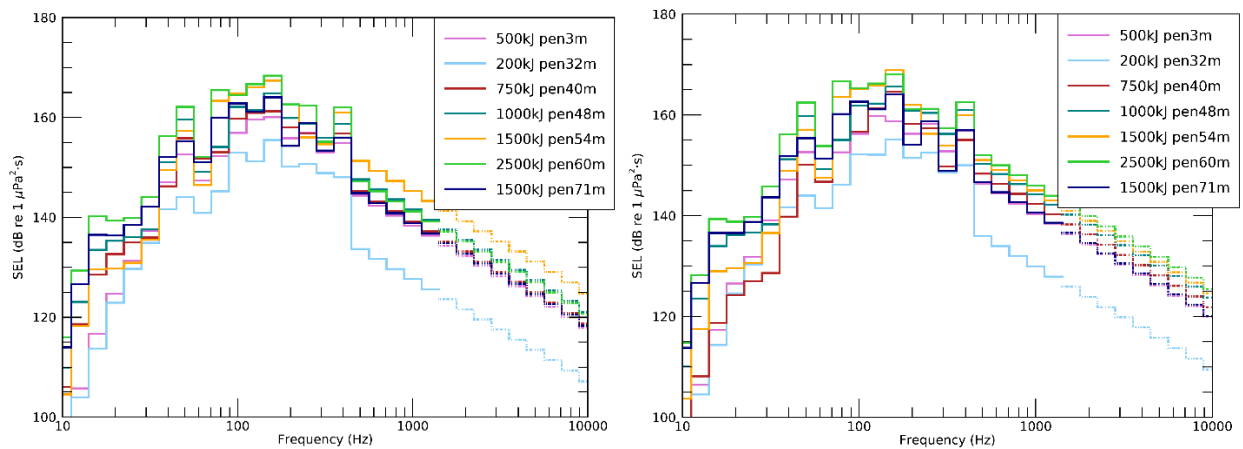
Figure 10. Location Z11: Deciddecade band spectral levels at 750 m for a 2.44 m diameter pin pile assuming an expected installation scenario using an IHC S-2500 kJ hammer with an average summer sound speed profile (left panel) and winter sound speed profile (right panel).
