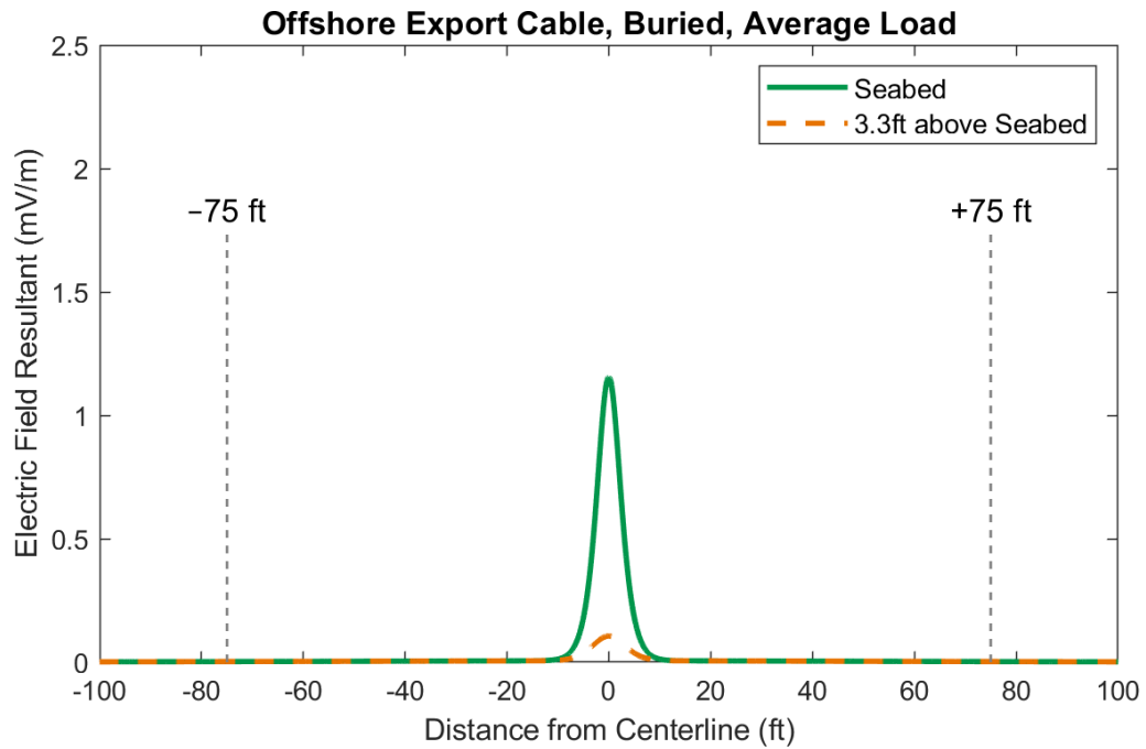
Figure C-8. Calculated induced electric-field levels in seawater above the 230-kV Offshore Export Cable for a 3.3-ft (1-m) burial depth and average loading.
