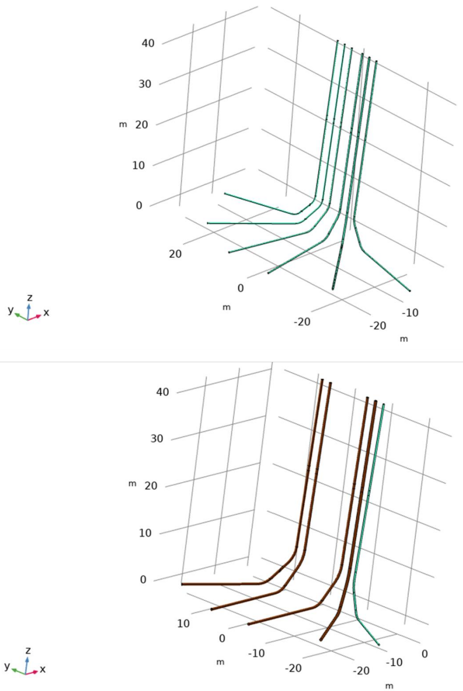
Figure 3. Schematic exemplifying the geometry of Inter-Array Cables (green) and Offshore Export Cables (brown) connecting to an Offshore Substation. The top figure illustrates cables traversing the east face of the jacket structure while the bottom figure shows cables traversing the south face of the jacket structure.
