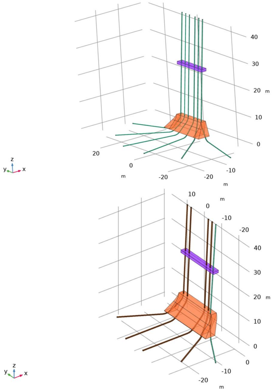
Figure D-4. Volumes over which AC magnetic- and induced-electric field levels are averaged at the Offshore Substation Foundation. The top figure shows the east face while the bottom figure illustrates the south face of the OSS. Green lines represent Inter-Array Cables and brown lines represent Offshore Export Cables.
