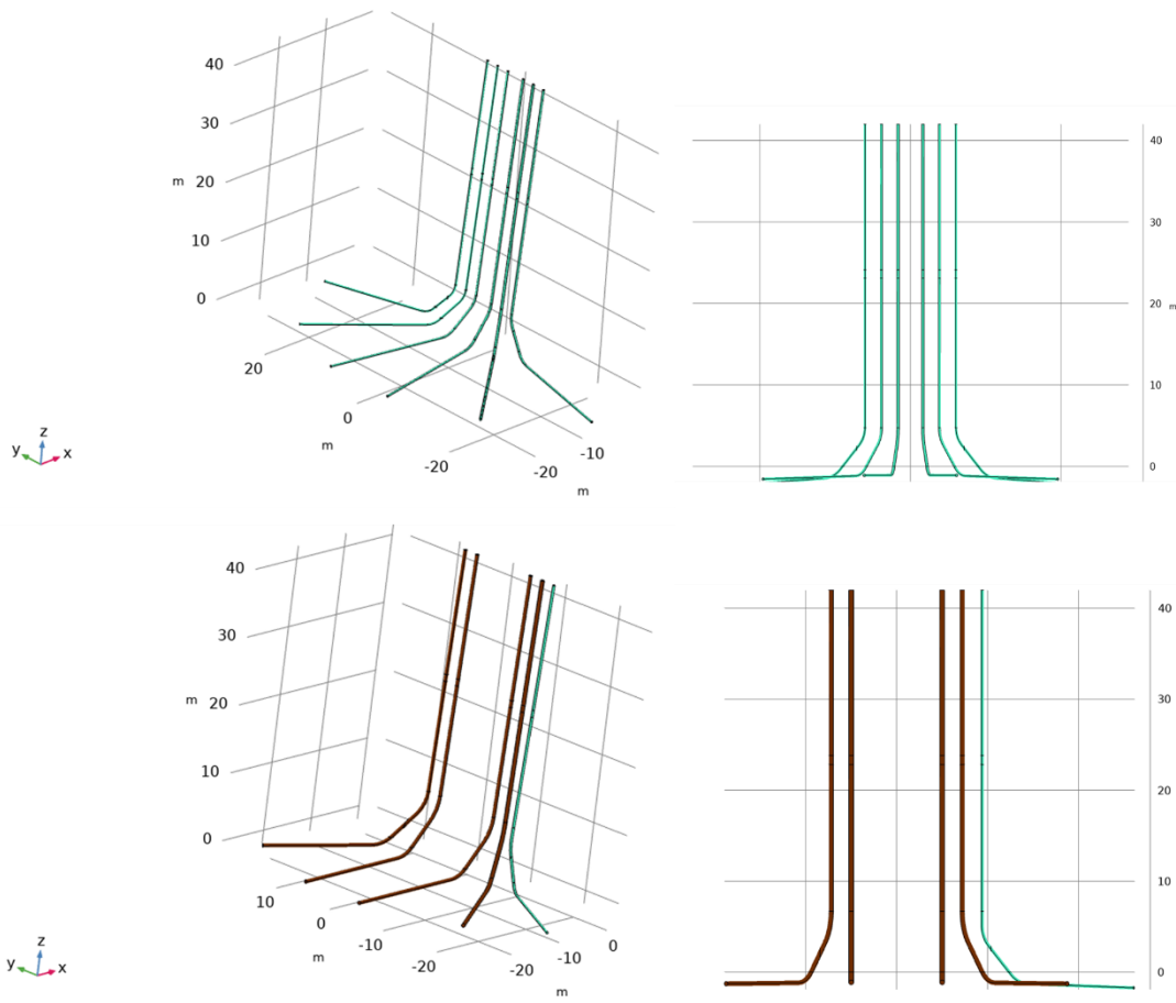
Figure A-3. Jacket foundation modeling configuration for cables on the Offshore Substations. Top images show the east face geometry while the bottom images show the south face geometry. Green lines represent Inter-Array Cables and brown lines represent Offshore Export Cables.
