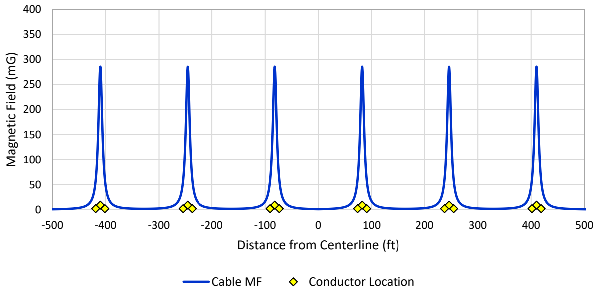
Figure 4.2 AC Magnetic Field Modeling Results at the Seabed for Buried 220-kV HVAC Offshore Export Cables. mG = Milligauss. Modeling results are based on six cables buried 1.2 m (3.94 ft) beneath the seabed, each carrying 1,700 A and with 50-m (164-ft) spacing between cables. Conductor locations on the graph are not to scale and are provided to show relative locations.
