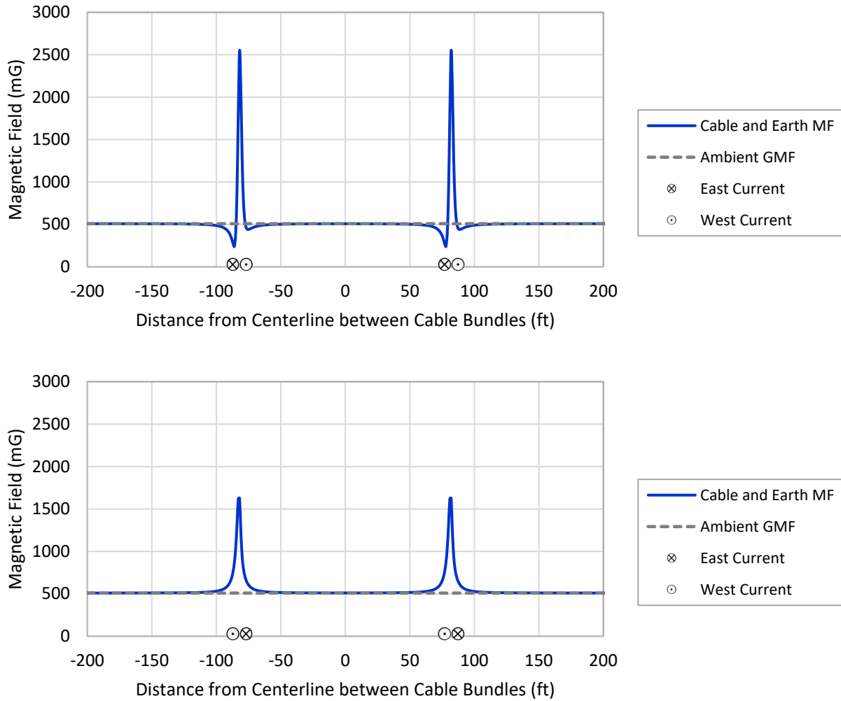
Figure B-4 Total DC Magnetic Field Modeling Results at 0.65 m (2.14 ft) Above the Seabed for Surface-Laid \pm 320 -kV HVDC Offshore Export Cables with East-West Route Orientation. mg= Milligauss. Total DC magnetic field modeling results are the combined fields from the HVDC offshore export cables and the earth's geomagnetic field (GMF). Modeling results are based on two cable bundles installed on the seabed and covered by cable protection with 0.5-m (1.6-ft) thickness, each carrying 2,300 A and with 50-m (164-ft) spacing between cables. Cables are oriented in an east-west direction and the view is facing east.
