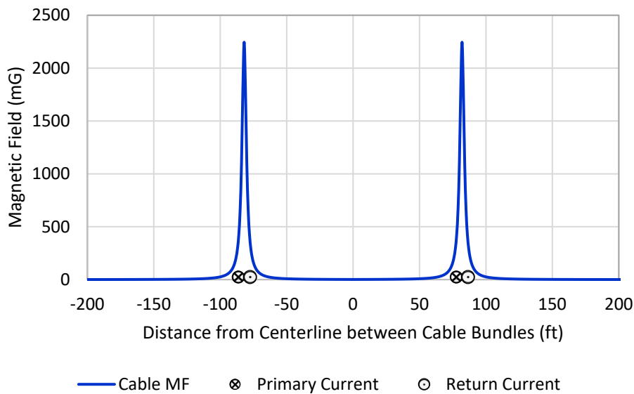
Figure 3.5 Cable-Specific DC Magnetic Field Modeling Results at 0.67 m (2.20 ft) Above the Seabed for Surface-Laid \pm 525 -kV HVDC Offshore Export Cables. mg= Milligauss. It is assumed that cable bundles are installed on the seabed and covered by cable protection with 0.5-m (1.6-ft) thickness. Conductor locations on the graph are not to scale and are provided to show relative locations.
