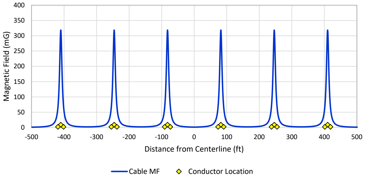
Figure 4.4 AC Magnetic Field Modeling Results at the Seabed for Buried 345-kV HVAC Offshore Export Cables. mG = Milligauss. Modeling results are based on six cables buried 1.2 m (3.94 ft) beneath the seabed, each carrying 1,700 A and with 50-m (164-ft) spacing between cables. Conductor locations on the graph are not to scale and are provided to show relative locations.
