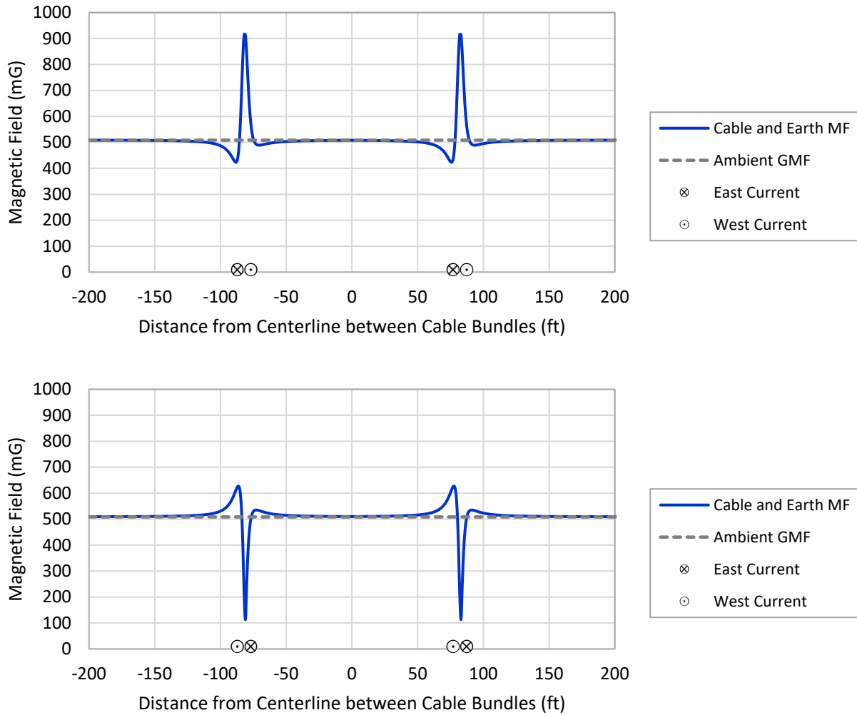
Figure B-2 Total DC Magnetic Field Modeling Results at the Seabed for Buried \pm 320 -kV HVDC Offshore Export Cables with East-West Route Orientation. mG = Milligauss. Total DC magnetic field modeling results are the combined fields from the HVDC offshore export cables and the earth's geomagnetic field (GMF). Modeling results are based on two cable bundles buried 1.2 m (3.94 ft) beneath the seabed, each carrying 2,300 A and with 50-m (164-ft) spacing between cable bundles. Cables are oriented in an east-west direction and the view is facing east.
