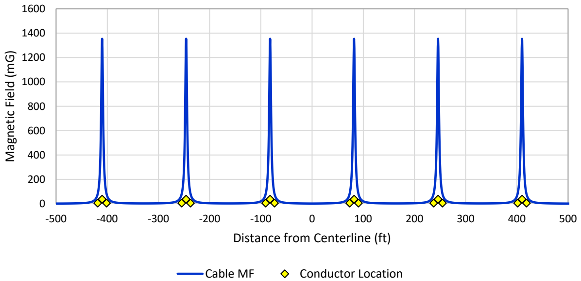
Figure 4.5 AC Magnetic Field Modeling Results at 0.82 m (2.68 ft) Above the Seabed for Surface-Laid 345-kV HVAC Offshore Export Cables. mG = Milligauss. Modeling results are based on six cables installed on the seabed covered by 0.5-m (1.6-ft) thick cable protection, each carrying 1,700 A and with 50-m (164-ft) spacing between cables. Conductor locations on the graph are not to scale and are provided to show relative locations.
