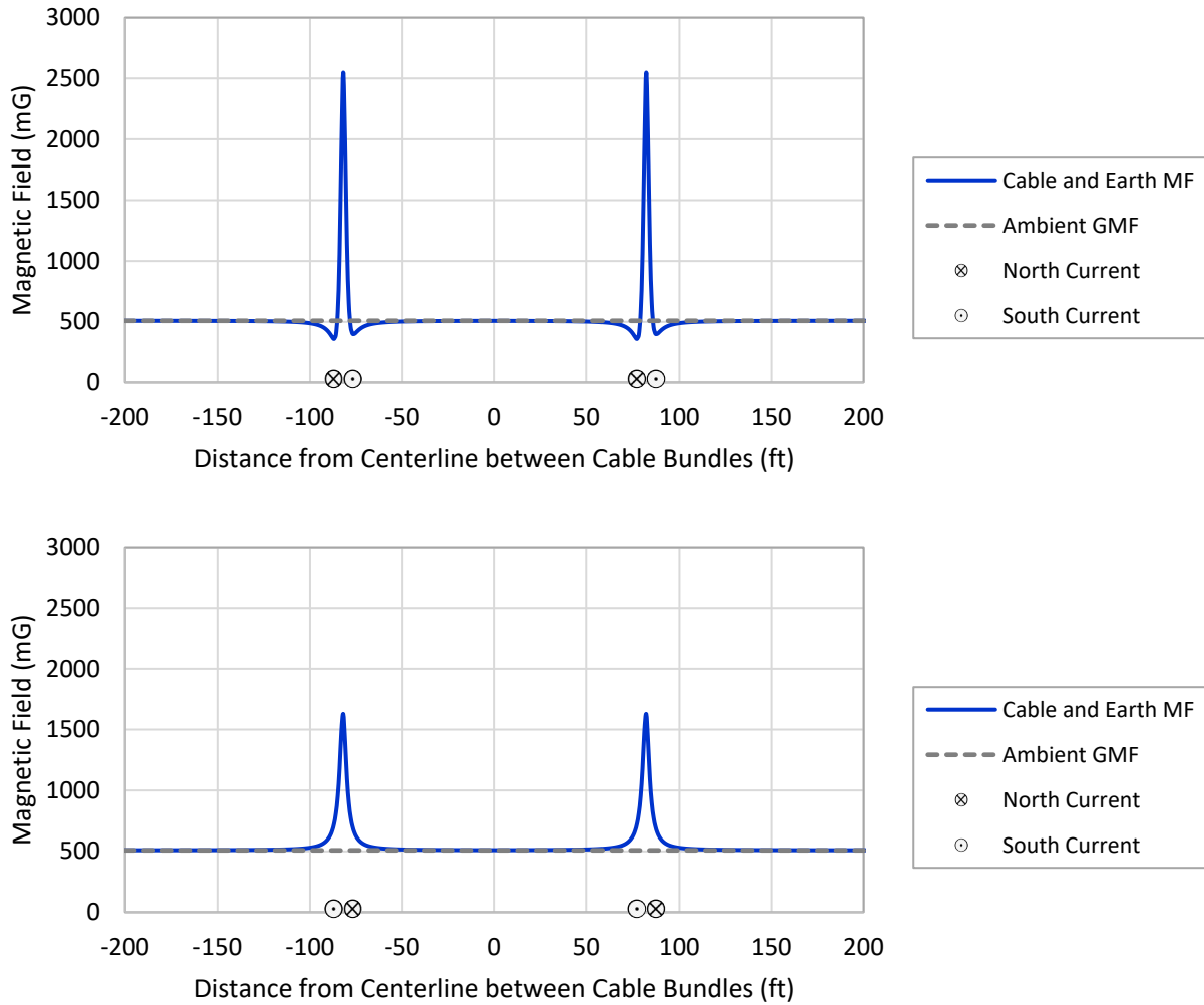
Figure B-3 Total DC Magnetic Field Modeling Results at 0.65 m (2.14 ft) Above the Seabed for Surface-Laid \pm 320 -kV HVDC Offshore Export Cables with North-South Route Orientation. mg= Milligauss. Total DC magnetic field modeling results are the combined fields from the HVDC offshore export cables and the earth's geomagnetic field (GMF). Modeling results are based on two cable bundles installed on the seabed and covered by cable protection with 0.5-m (1.6-ft) thickness, each carrying 2,300 A and with 50-m (164-ft) spacing between cables. Cables are oriented in a north-south direction and the view is facing north.
