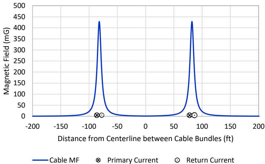
Figure 3.2 Cable-Specific DC Magnetic Field Modeling Results at the Seabed for Buried \pm 320 -kV HVDC Offshore Export Cables. mg= Milligauss. Modeling results are based on two cable bundles buried 1.2 m (3.94 ft) beneath the seabed, each carrying 2,300 A and with 50-m (164-ft) spacing between cable bundles. Conductor locations on the graph are not to scale and are provided to show relative locations.
