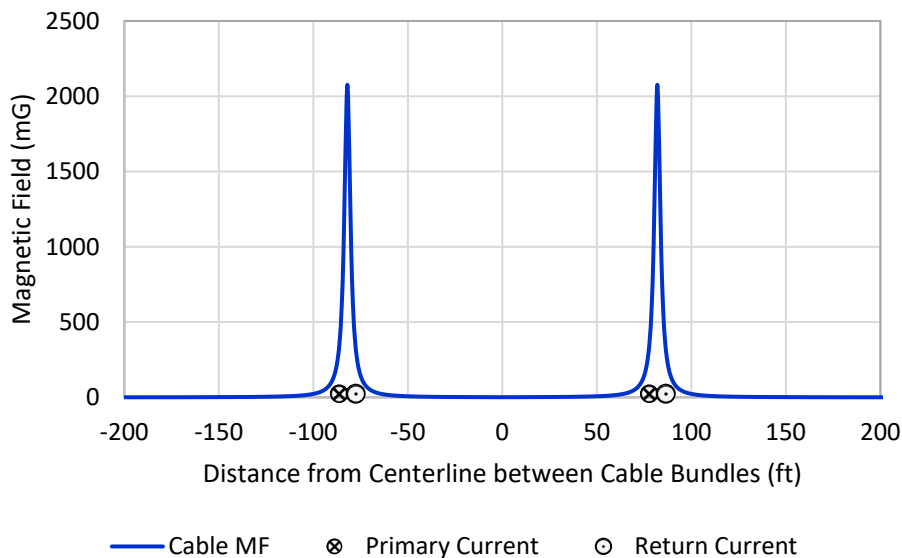
Figure 3.3 Cable-Specific DC Magnetic Field Modeling Results at 0.65 m (2.14 ft) Above the Seabed for Surface-Laid \pm 320 -kV HVDC Offshore Export Cables. mg= Milligauss. It is assumed that cable bundles are installed on the seabed and covered by cable protection with 0.5-m (1.6-ft) thickness. Each cable bundle has a loading of 2,300 A and there is 50-m (164-ft) spacing between cable bundles. Conductor locations on the graph are not to scale and are provided to show relative locations.
