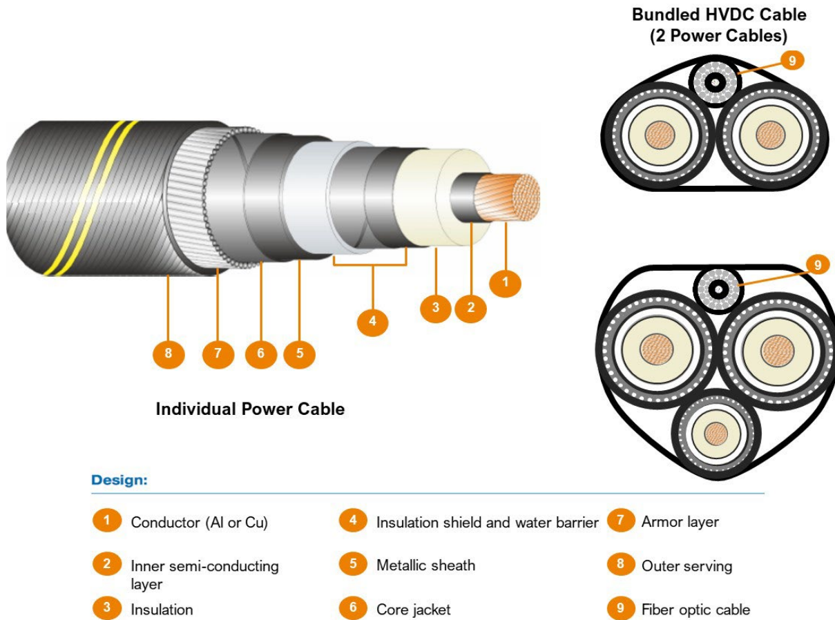
Figure 3.1 Example HVDC Cable Cross Section Illustration
