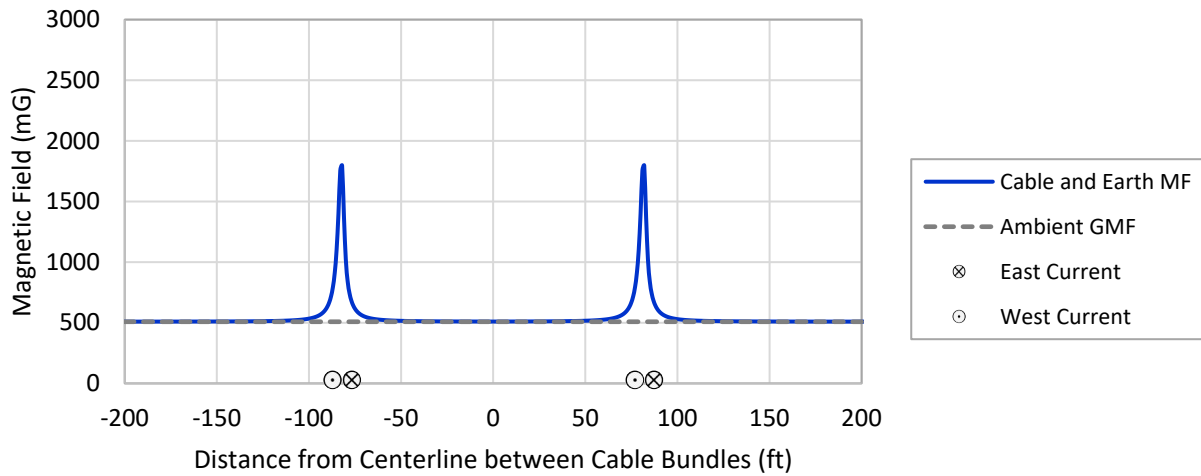
Figure B-8 Total DC Magnetic Field Modeling Results at 0.67 m (2.20 ft) Above the Seabed for Surface-Laid \pm 525 -kV Submarine Cables with East-West Route Orientation. mg= Milligauss. Total DC magnetic field modeling results are the combined fields from the HVDC offshore export cables and the earth's geomagnetic field (GMF). Modeling results are based on two cable bundles installed on the seabed and covered by cable protection with 0.5-m (1.6-ft) thickness, each carrying 2,300 A and with 50-m (164-ft) spacing between cables. Cables are oriented in an east-west direction and the view is facing east.
