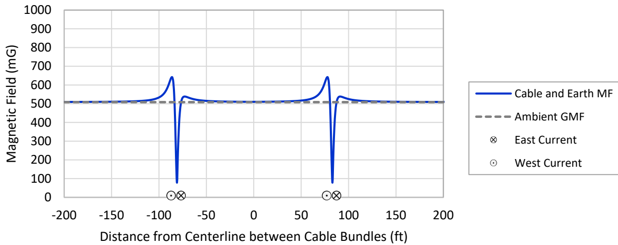
Figure B-6 Total DC Magnetic Field Modeling Results at the Seabed for Buried \pm 525 -kV HVDC Offshore Export Cables with East-West Route Orientation. mG = Milligauss. Total DC magnetic field modeling results are the combined fields from the HVDC offshore export cables and the earth's geomagnetic field (GMF). Modeling results are based on two cable bundles buried 1.2 m (3.94 ft) beneath the seabed, each carrying 2,300 A and with 50-m (164-ft) spacing between cable bundles. Cables are oriented in an east-west direction and the view is facing east.
