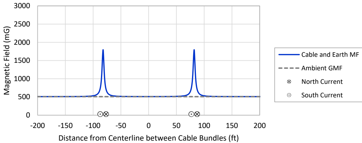
Figure B-7 Total DC Magnetic Field Modeling Results at 0.67 m (2.20 ft) Above the Seabed for Surface-Laid \pm 525 -kV HVDC Offshore Export Cables with North-South Route Orientation. mg= Milligauss. Total DC magnetic field modeling results are the combined fields from the HVDC offshore export cables and the earth's geomagnetic field (GMF). Modeling results are based on two cable bundles installed on the seabed and covered by cable protection with 0.5-m (1.6-ft) thickness, each carrying 2,300 A and with 50-m (164-ft) spacing between cables. Cables are oriented in a north-south direction and the view is facing north.
