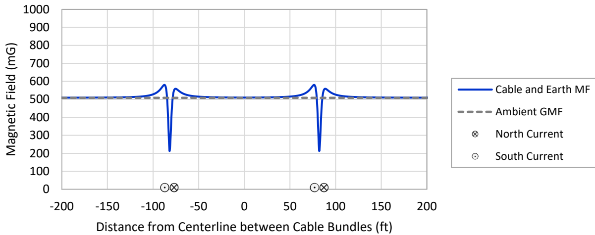
Figure B-1 Total DC Magnetic Field Modeling Results at the Seabed for Buried \pm 320 -kV HVDC Offshore Export Cables with North-South Route Orientation. mG = Milligauss. Total DC magnetic field modeling results are the combined fields from the HVDC offshore export cables and the earth's geomagnetic field (GMF). Modeling results are based on two cable bundles buried 1.2 m (3.94 ft) beneath the seabed, each carrying 2,300 A and with 50-m (164-ft) spacing between cable bundles. Cables are oriented in a north-south direction and the view is facing north.
