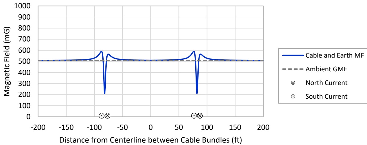
Figure B-5 Total DC Magnetic Field Modeling Results at the Seabed for Buried \pm 525 -kV HVDC Offshore Export Cables with North-South Route Orientation. mG = Milligauss. Total DC magnetic field modeling results are the combined fields from the HVDC offshore export cables and the earth's geomagnetic field (GMF). Modeling results are based on two cable bundles buried 1.2 m (3.94 ft) beneath the seabed, each carrying 2,300 A and with 50-m (164-ft) spacing between cable bundles. Cables are oriented in a north-south direction and the view is facing north.
