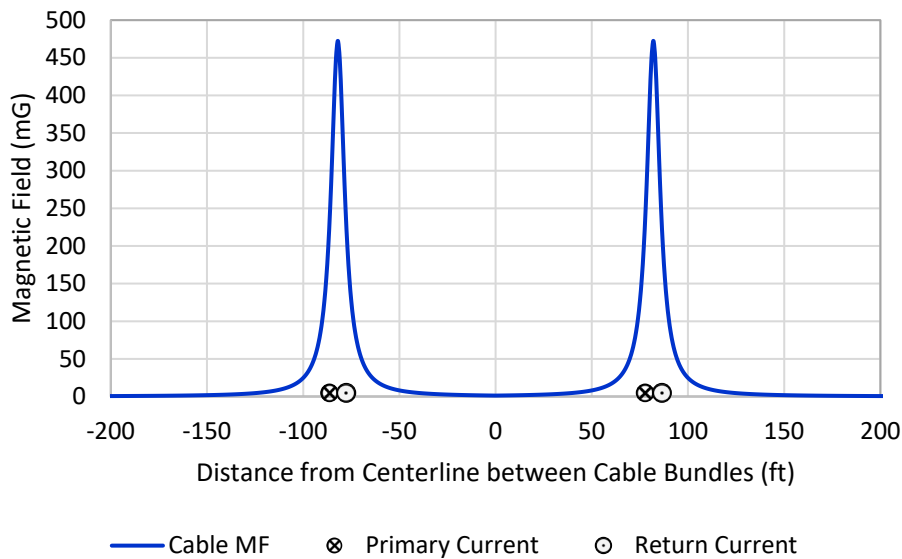
Figure 3.4 Cable-Specific DC Magnetic Field Modeling Results at the Seabed for Buried \pm 525 -kV HVDC Offshore Export Cables. mg= Milligauss. Modeling results are based on two cable bundles buried 1.2 m (3.94 ft) beneath the seabed, each carrying 2,300 A and with 50-m (164-ft) spacing between cable bundles. Conductor locations on the graph are not to scale and are provided to show relative locations.
