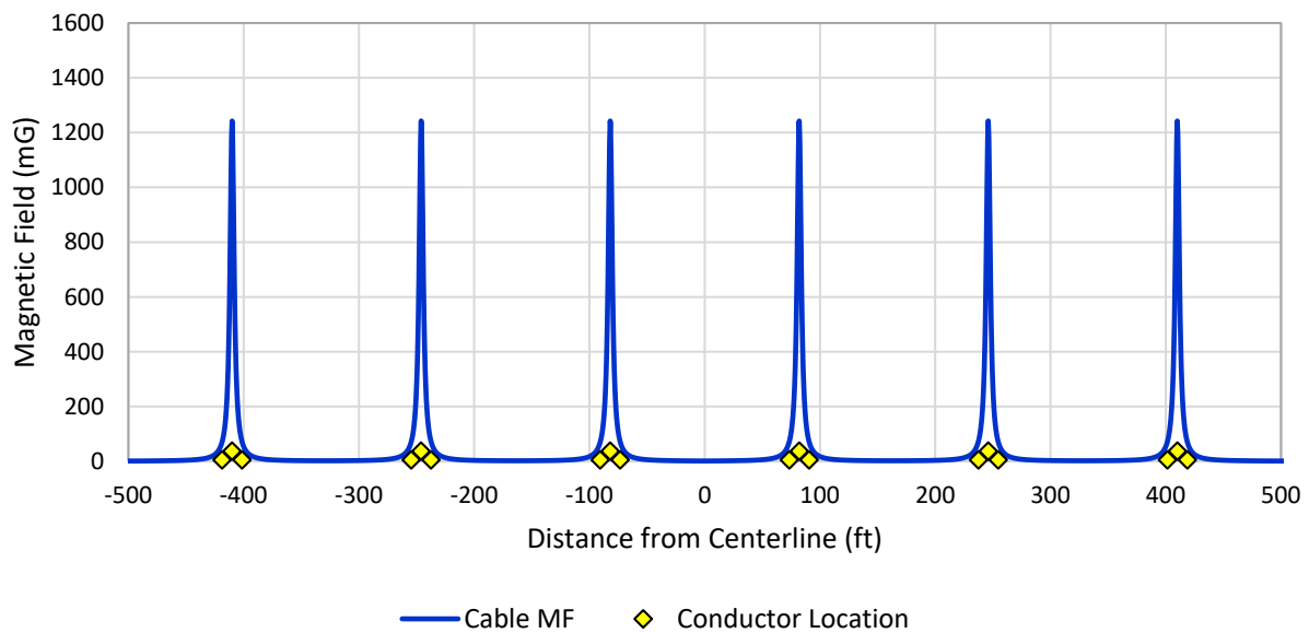
Figure 4.3 AC Magnetic Field Modeling Results at 0.79 m (2.58 ft) Above the Seabed for Surface-Laid 220-kV HVAC Offshore Export Cables. mG = Milligauss. Modeling results are based on six cables installed on the seabed covered by 0.5-m (1.6-ft) thick cable protection, each carrying 1,700 A and with 50-m (164-ft) spacing between cables. Conductor locations on the graph are not to scale and are provided to show relative locations.
