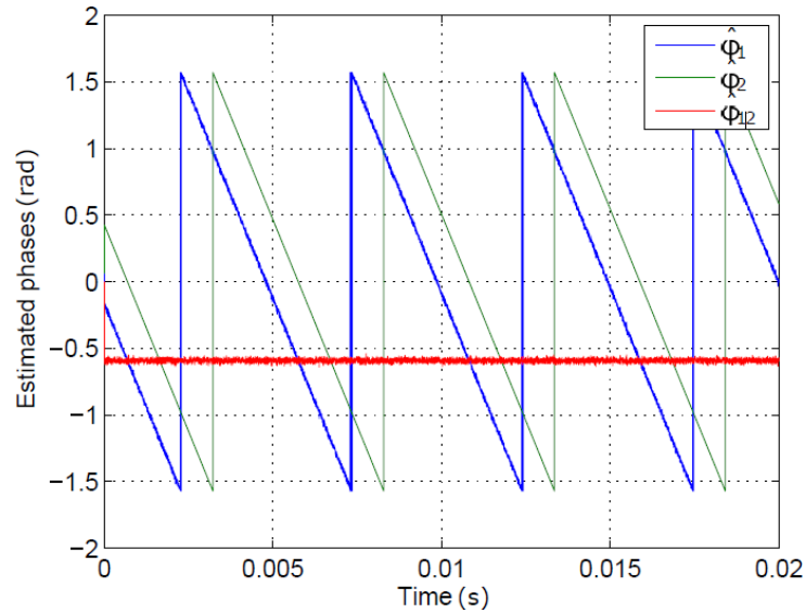
Figure 2.5. Output of phase meters from David et al. (2016).
