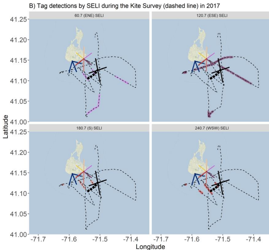
Figure 1.81. Summary of detections at 4 9-element 11-dB antennas of a test tag from a 12 m tall station at Southeast Lighthouse, Block Island, RI during a calibration survey on 13 September 2017. A kite was flown behind a boat (dotted line for 203 min) at altitude of ~20 m. Antennas facing 300 deg and due north (0 deg) had no detections. Detections for the antenna facing 60.7 deg (pink segments) in upper left panel, 120.7 deg (purple segments) in
