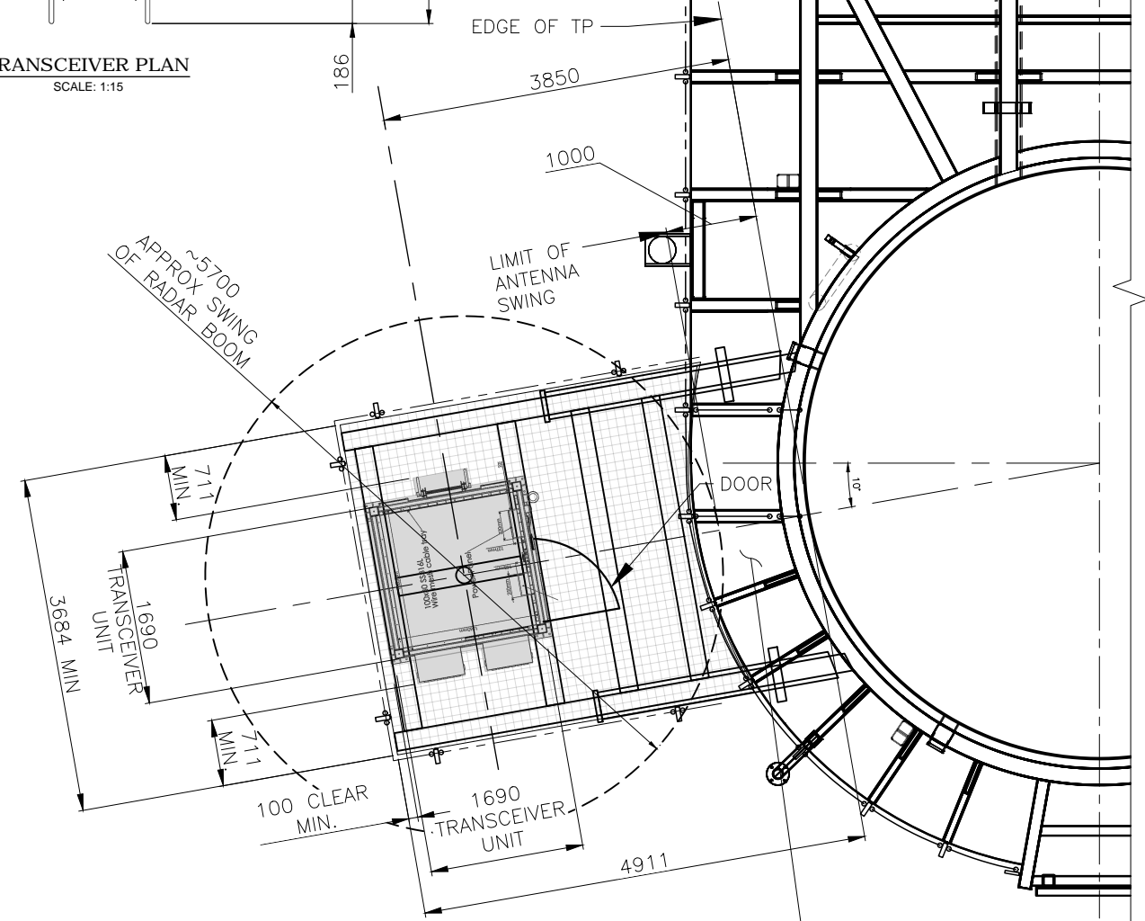
EXTERNAL PLATFORM RADAR/ANTENNA FRAMING PLAN - LOCATION II SCALE: 1:30
