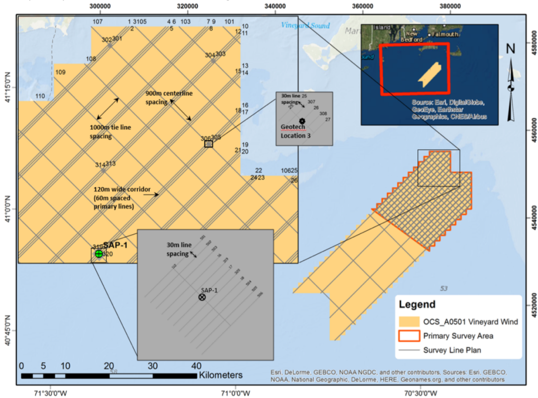
Figure 2-1 Line plan of global geophysical survey
